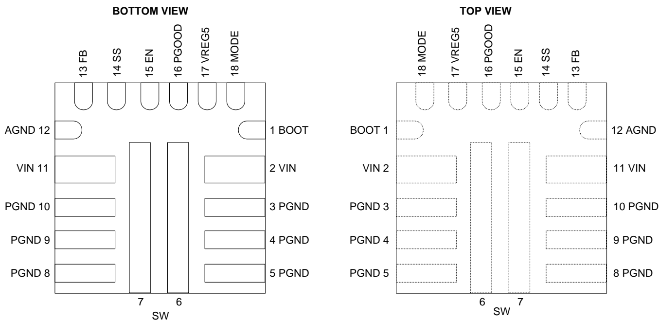
RNN Package 18-Pin VQFN
