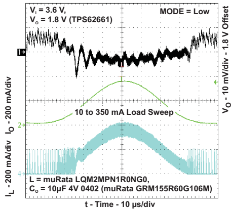
Figure 23. AC Load Transient Response
