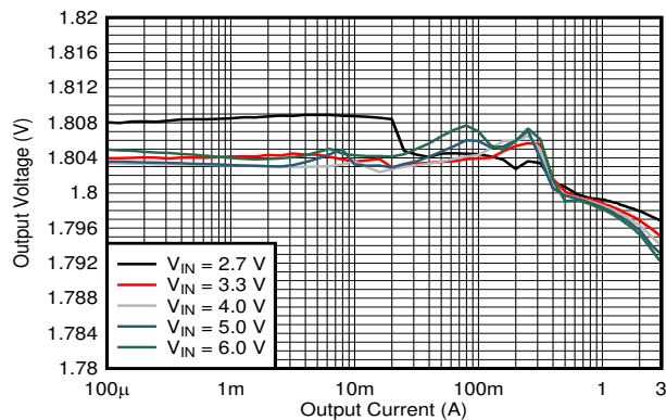
Figure 9-10. Output Voltage Versus Output Current
