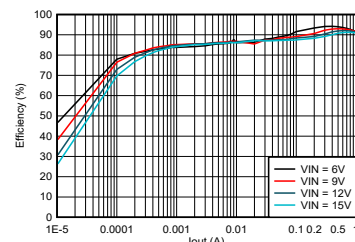
Efficiency Versus Output Current V OUT = 3.3 V at 2.5-MHz Auto PFM/PWM
