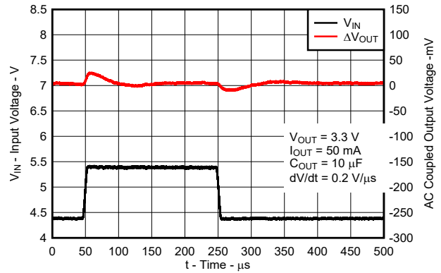
V_{OUT} = 3.3\text{ V} , I_{OUT} = 50\text{ mA} , C_{OUT} = 10\text{ }\mu\text{F}
