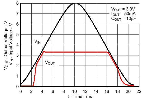
Figure 8-6. TPS71533-Q1 Power-Up and Power-Down Waveform for New Chip
