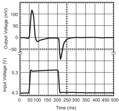
V_{OUT} = 3.3\text{ V} , I_{OUT} = 50\text{ mA} , C_{OUT} = 10\text{ }\mu\text{F}
