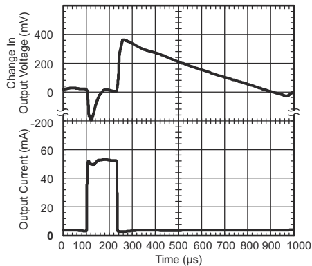
V_{IN} = 4.3\text{ V} , V_{OUT} = 3.3\text{ V} , C_{OUT} = 10\text{ }\mu\text{F}
