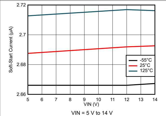
Figure 7-10. Soft-Start Current Variation
