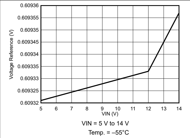
Figure 7-12. Voltage Reference Variation
