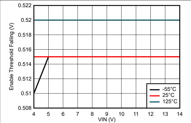
Figure 7-8. Enable Threshold Falling Variation
