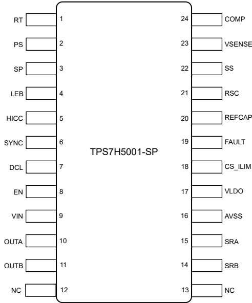
Figure 6-5. TPS7H5001-SP PW Package 24-Pin TSSOP (Top View)
