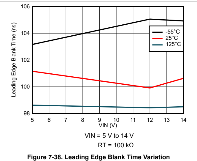
Figure 7-38. Leading Edge Blank Time Variation
