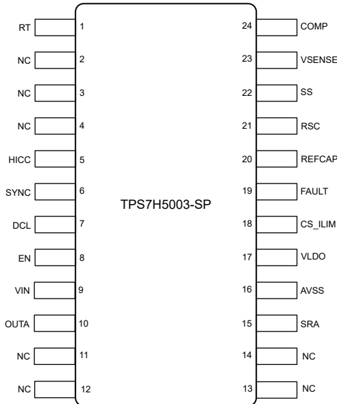
Figure 6-7. TPS7H5003-SP PW Package 24-Pin TSSOP (Top View)
