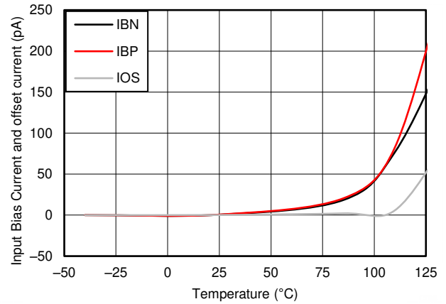
Figure 7-8. Input Bias Current vs Temperature
