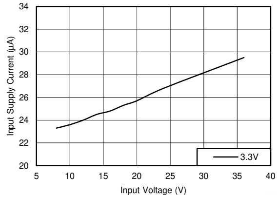
9-26. Input Supply Current
