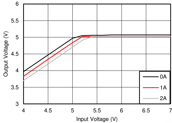
8-9. Overall Dropout Characteristic V_{OUT} = 5\text{ V}
