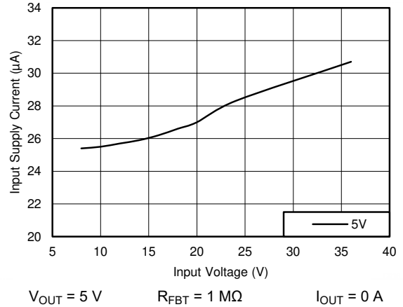
9-20. Input Supply Current
