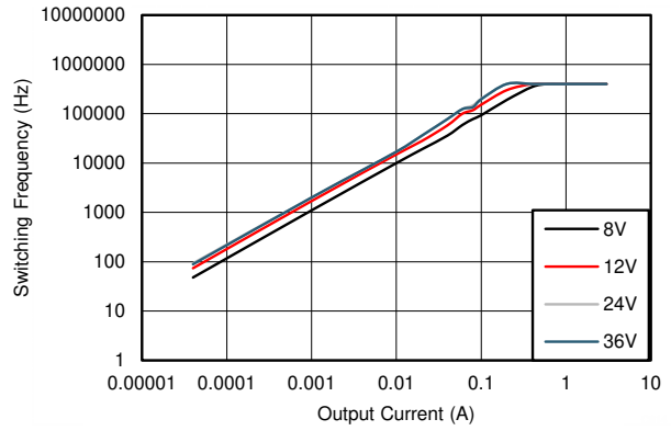
9-22. Switching Frequency versus Output Current
