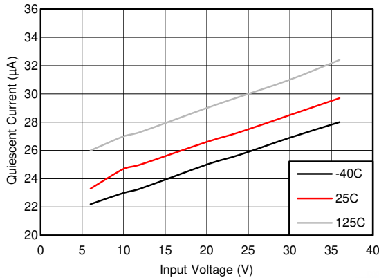
7-1. Non-Switching Input Supply Current
