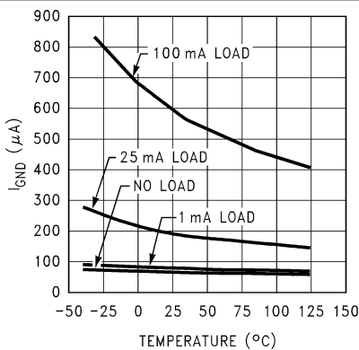
5-15. Ground Pin Current ( I_{GND} ) versus Temperature (Legacy Chip)
