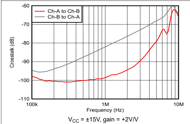
5-21. OPA2891 Crosstalk vs Frequency
