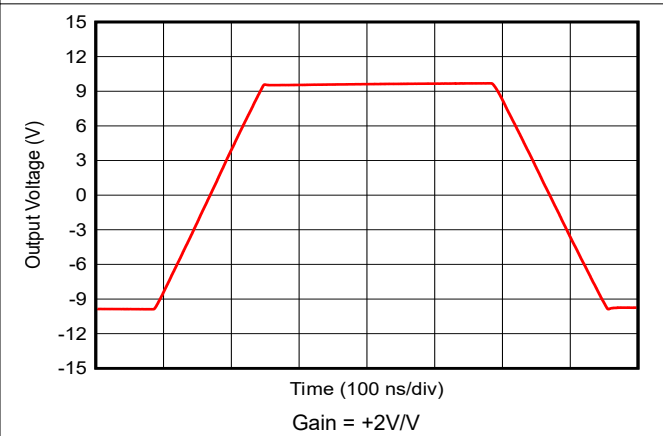
5-24. 20V Step Response
