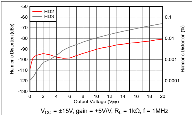
5-19. Harmonic Distortion vs Peak-to-Peak Output Voltage
