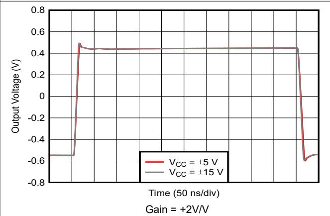
5-22. 1V Step Response
