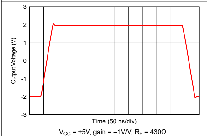
5-23. 4V Step Response
