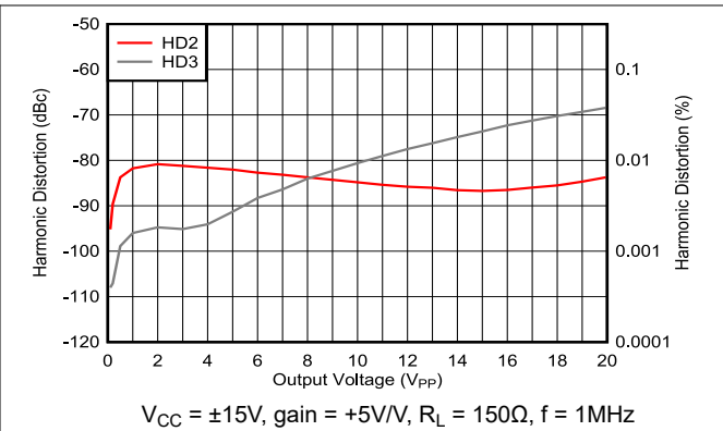
5-20. Harmonic Distortion vs Peak-to-Peak Output Voltage
