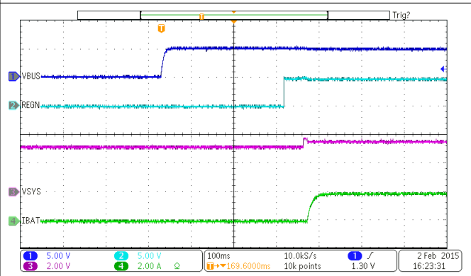
9-5. Power Up with Charge Enabled
