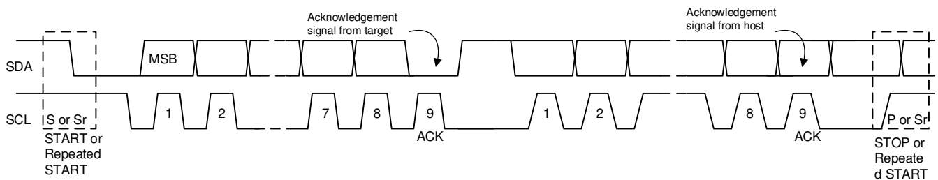
8-11. Data Transfer on the I 2 C Bus
