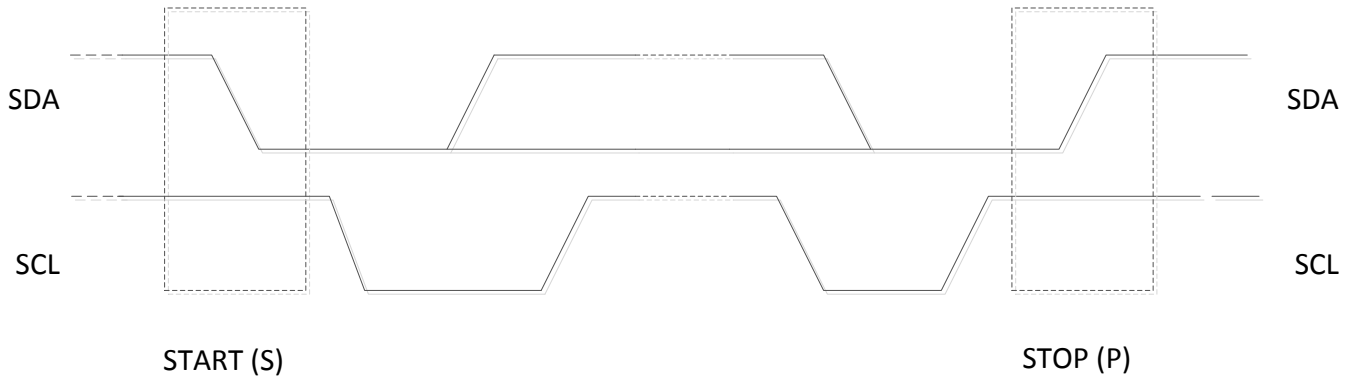
8-10. START and STOP conditions
