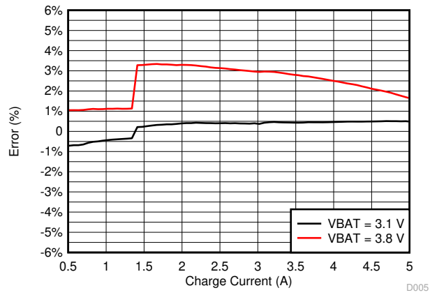
7-4. Charge Current Accuracy vs Charge Current I 2 C Setting
