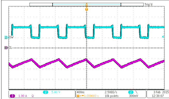
9-12. Boost Mode Switching Waveform
