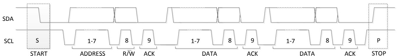
8-12. Complete Data Transfer
