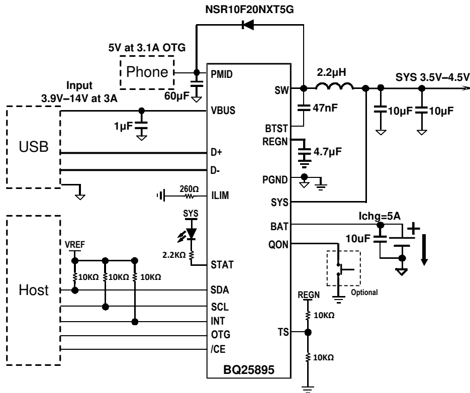
9-14. BQ25895 with D+/D- Interface, 3.1-A Boost Mode Output, and No Thermistor Connections
