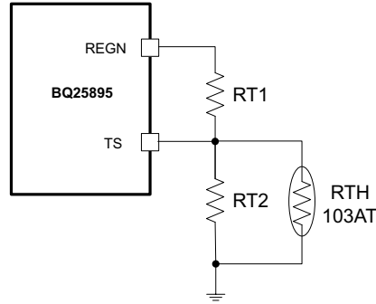
8-6. TS Resistor Network
