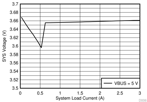
7-5. SYS Voltage Regulation vs System Load Current
