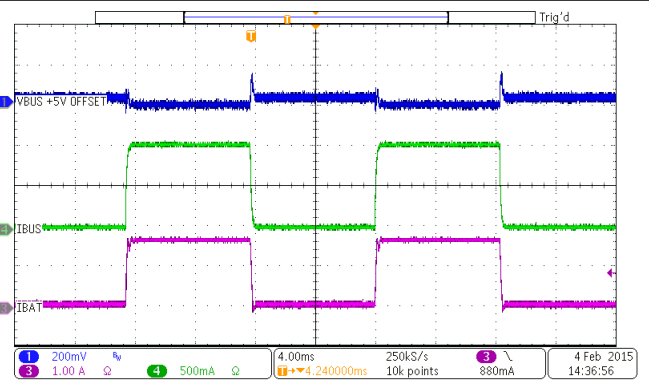
9-11. PFM Switching Waveform
