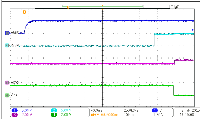
9-2. Power Up from USB100
