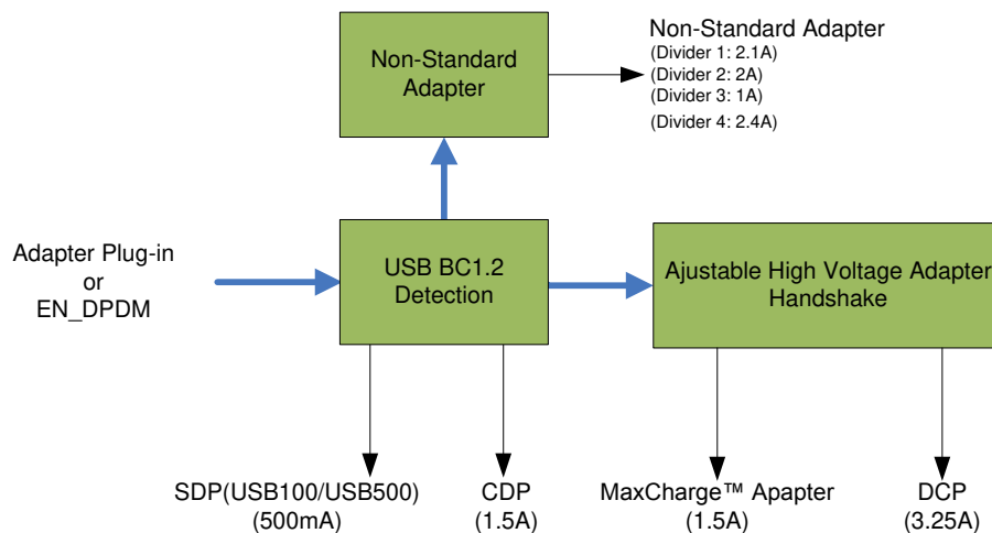
8-1. USB D+/D- Detection
