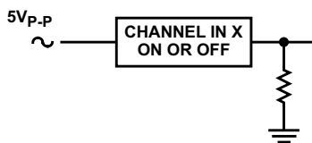
Figure 7-15. Crosstalk Between Duals or Triplets (CD4052B, CD4053B)
