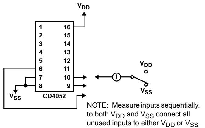
Figure 7-12. Input Current
