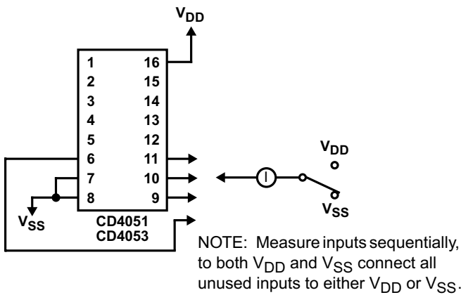
Figure 7-12. Input Current
