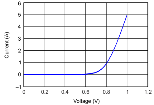
6-4. Drain to Source Diode Forward On Characteristics
