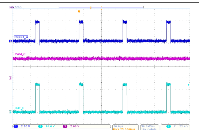
8-3. Input and Output Functionality
