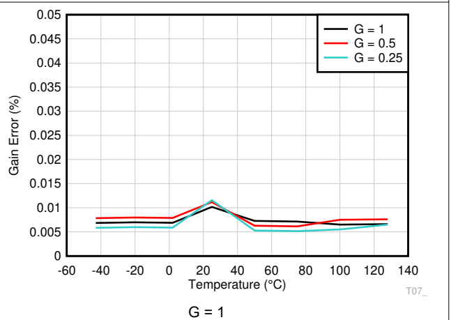
图 6-18. Gain Error vs Temperature
