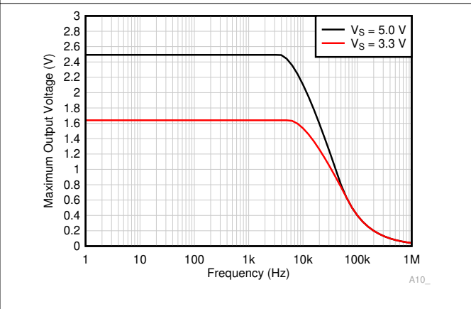
6-44. Maximum Output Voltage vs Frequency
