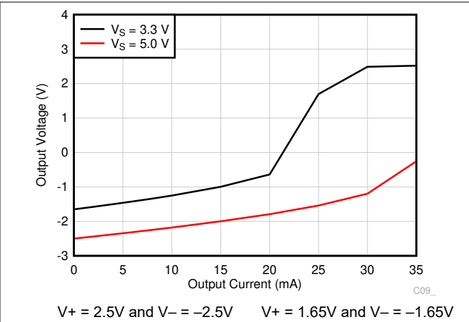
6-34. Output Voltage vs Output Current (Sinking)
