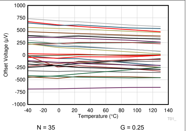
图 6-16. Output Referred Offset Voltage vs Temperature
