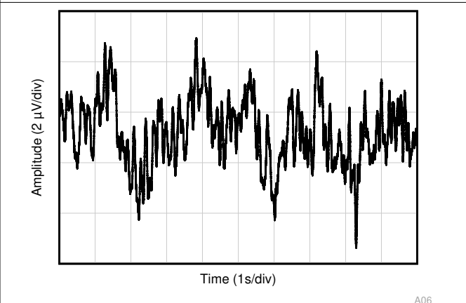
6-42. Output Referred 0.1 Hz to 10 Hz Voltage Noise in Time Domain
