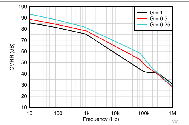
6-36. CMRR (Referred to Output) vs Frequency
