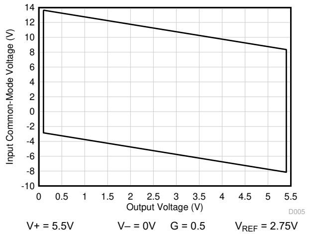
6-76. Input Common-Mode Voltage vs Output Voltage (Rail-to-Rail CMRR Region)
