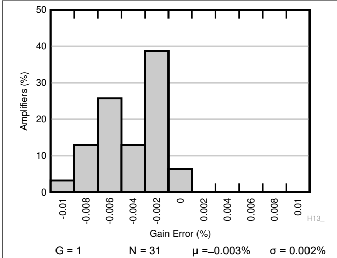
图 6-13. Typical Distribution of Reference Gain Error
