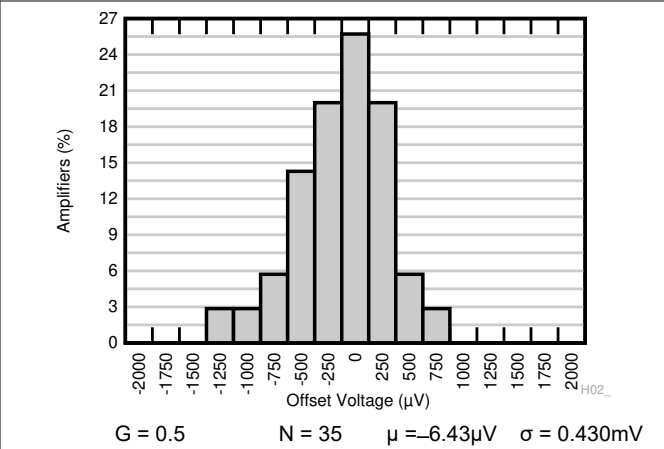
6-2. Typical Distribution of Output Referred Offset Voltage
