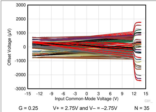
图 6-23. Output Referred Offset Voltage vs Input Common-Mode Voltage
