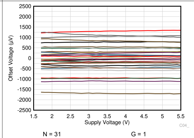
6-30. Output Referred Offset Voltage vs Supply Voltage
