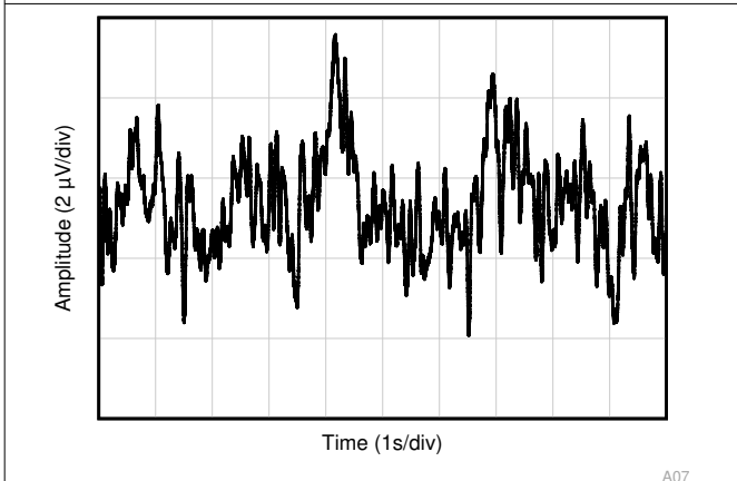
6-41. Output Referred 0.1 Hz to 10 Hz Voltage Noise in Time Domain
