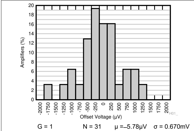
6-1. Typical Distribution of Output Referred Offset Voltage
