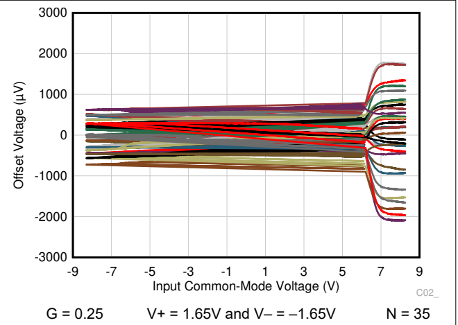
图 6-26. Output Referred Offset Voltage vs Input Common-Mode Voltage
