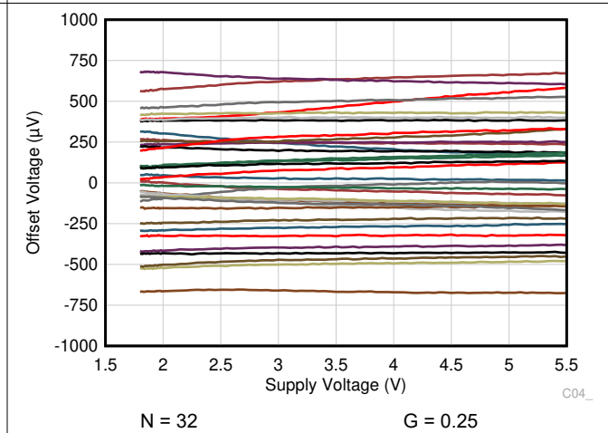
6-32. Output Referred Offset Voltage vs Supply Voltage
