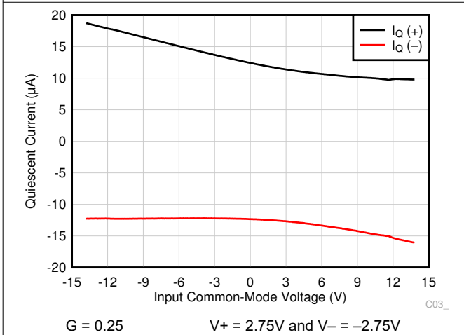
6-29. Quiescent Current vs Input Common-Mode Voltage
