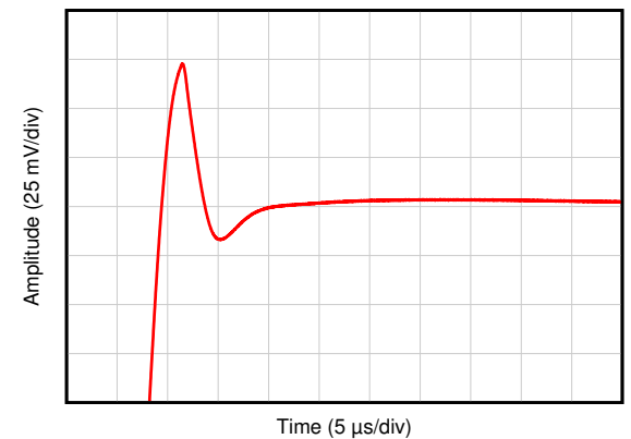
TR05 V_+ = 2.75\text{V} V_- = -2.75\text{V} G = 0.5 V_{OUT} = 4V_{PP}
