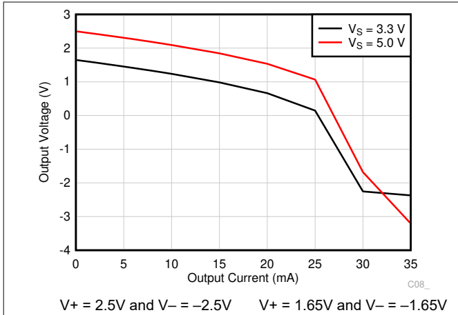
6-33. Output Voltage vs Output Current (Sourcing)
