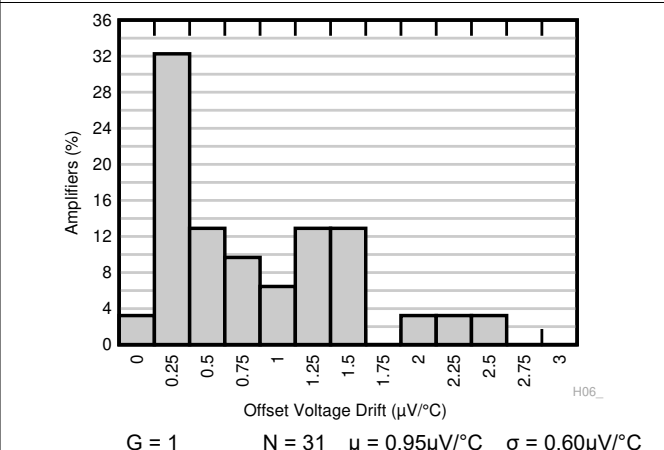
6-4. Typical Distribution of Output Referred Offset Drift
