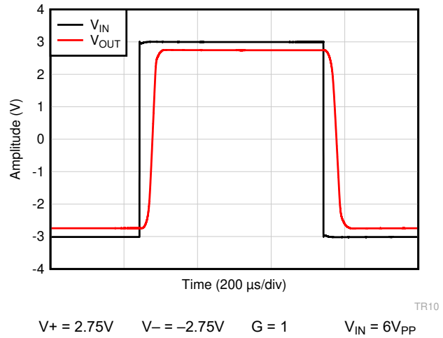
6-64. Over-Load Recovery
