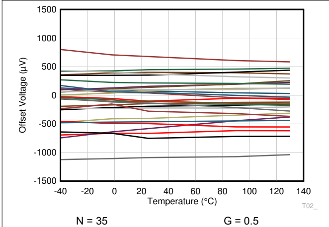
图 6-15. Output Referred Offset Voltage vs Temperature
