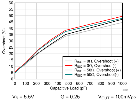
6-63. Small-Signal Overshoot vs Capacitive Load
