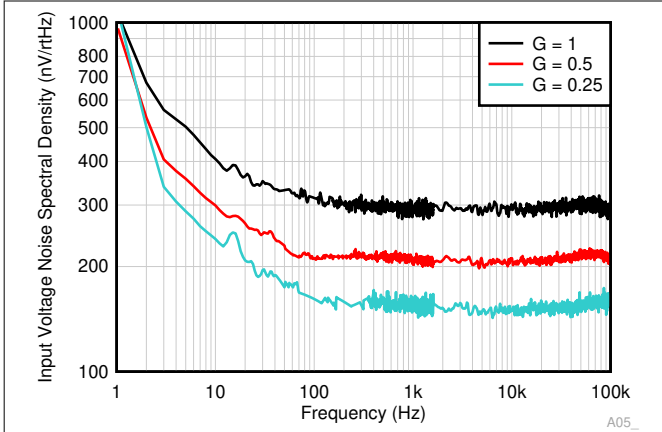
6-39. Output Referred Voltage Noise Spectral Density
