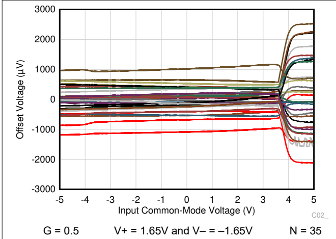
图 6-25. Output Referred Offset Voltage vs Input Common-Mode Voltage
