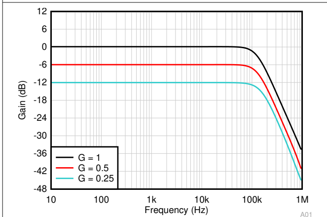
6-35. Closed-Loop Gain vs Frequency
