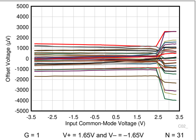
图 6-24. Output Referred Offset Voltage vs Input Common-Mode Voltage
