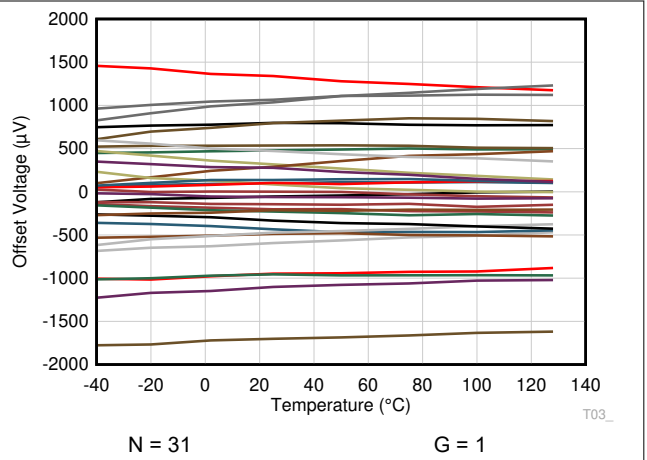
图 6-14. Output Referred Offset Voltage vs Temperature
