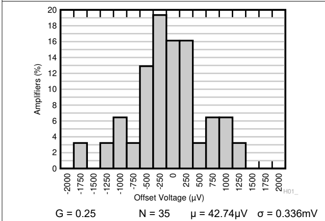
6-3. Typical Distribution of Output Referred Offset Voltage
