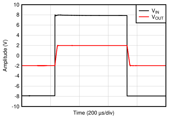
TR04 V_+ = 2.75\text{V} V_- = -2.75\text{V} G = 0.25 V_{OUT} = 4V_{PP}
