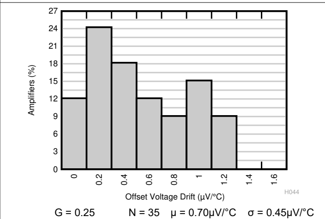
6-6. Typical Distribution of Output Referred Offset Drift
