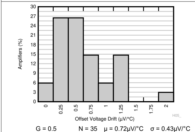
6-5. Typical Distribution of Output Referred Offset Drift
