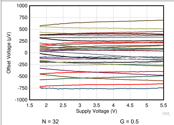
6-31. Output Referred Offset Voltage vs Supply Voltage
