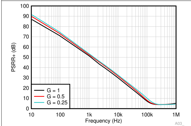
6-37. PSRR+ (Referred to Output) vs Frequency
