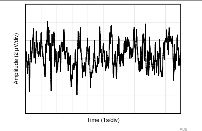
6-40. Output Referred 0.1 Hz to 10 Hz Voltage Noise in Time Domain
