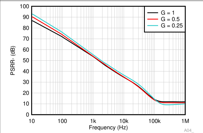
6-38. PSRR- (Referred to Output) vs Frequency
