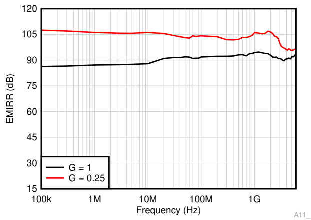
7-4. Electromagnetic Interference Rejection Ratio Referred to Output vs Frequency (Differential Input)
