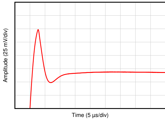
TR06 V_+ = 2.75\text{V} V_- = -2.75\text{V} G = 1 V_{OUT} = 4V_{PP}
