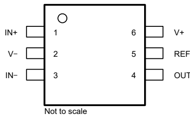
図 5-1. INA500 DCK Package, 6-Pin SC70 (Top View)
