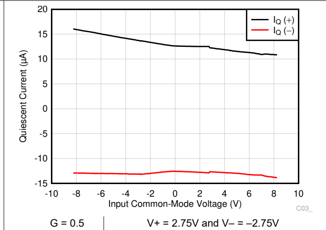
6-28. Quiescent Current vs Input Common-Mode Voltage
