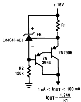
Figure 26. Current Source
