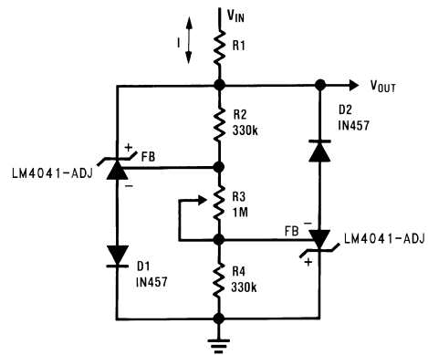
Figure 30. Bidirectional Adjustable Clamp ±2.4 V to ±6 V
