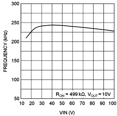
8-3. Frequency vs Input Voltage
