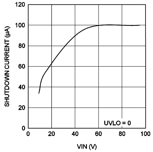
6-8. I_{IN} vs V_{IN} (Shutdown)
