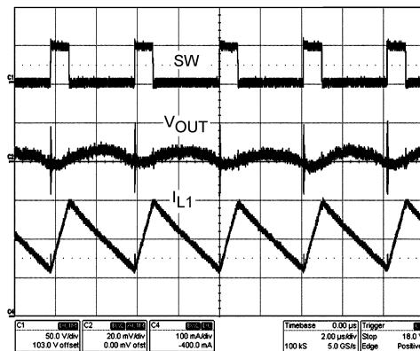
8-4. Typical Switching Waveform ( V_{IN} = 48\text{ V} , I_{OUT} = 200\text{ mA} )
