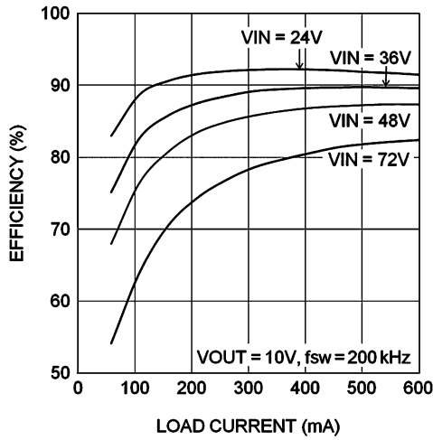
6-1. Efficiency at 200 kHz, 10 V
