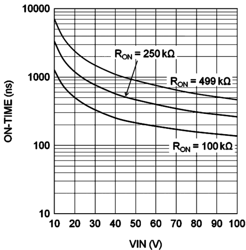
6-5. T_{ON} vs V_{IN} and R_{ON}
