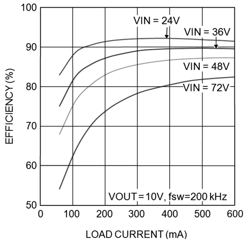
8-2. Efficiency vs Load Current
