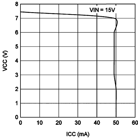
6-3. V_{CC} vs I_{CC}
