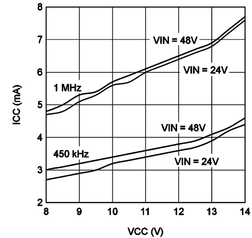
6-4. I_{CC} vs External V_{CC}
