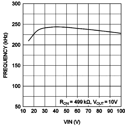
6-9. Switching Frequency vs V_{IN}
