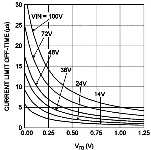
6-6. T_{OFF} ( I_{LIM} ) vs V_{FB} and V_{IN}
