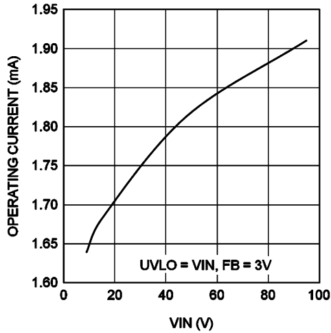
6-7. I_{IN} vs V_{IN} (Operating, Non-Switching)
