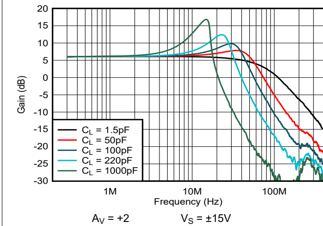
5-33. Closed-Loop Frequency Response vs Capacitive Load
