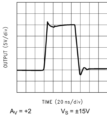
5-68. Large-Signal Pulse Response
