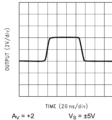
5-69. Large-Signal Pulse Response
