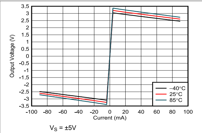
図 5-8. Output Voltage vs Output Current
