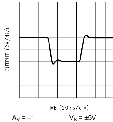
5-67. Large-Signal Pulse Response
