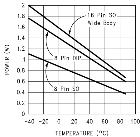
5-92. Maximum Power Dissipation vs Ambient Temperature
