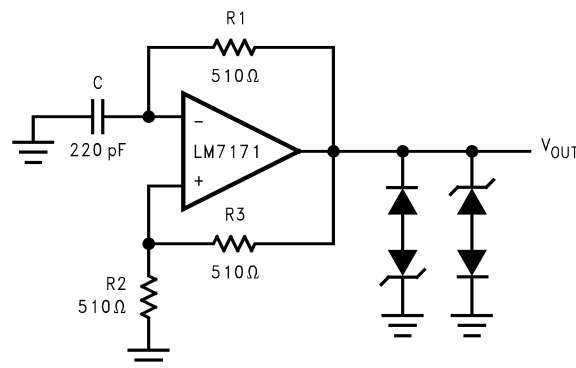
6-3. Multivibrator
