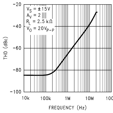
图 5-85. Total Harmonic Distortion vs Frequency
