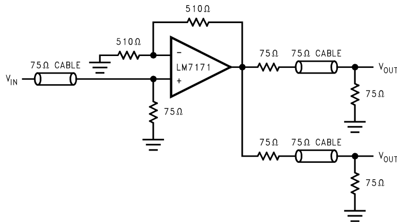
図 6-5. Video Line Driver
