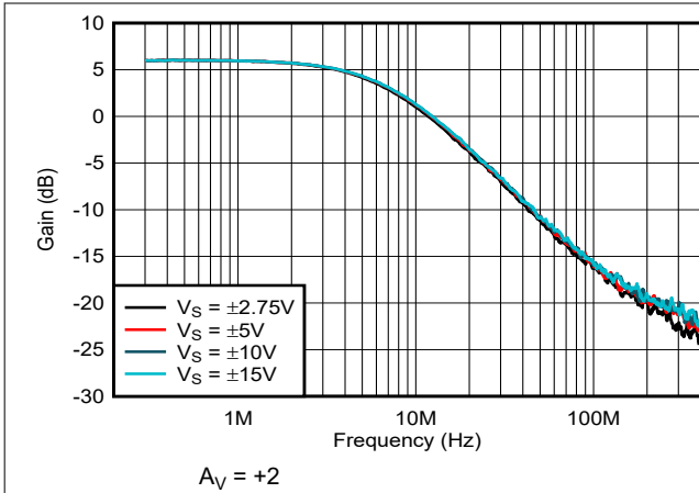
5-31. Closed-Loop Frequency Response vs Supply Voltage
