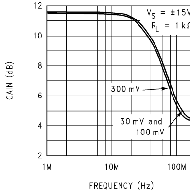
5-79. Closed-Loop Frequency Response vs Input Signal Level
