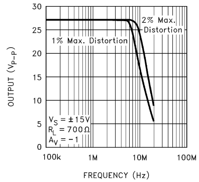
5-89. Undistorted Output Swing vs Frequency
