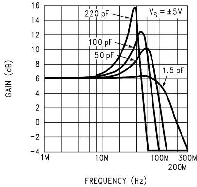
5-76. Closed-Loop Frequency Response vs Capacitive Load
