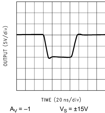
5-66. Large-Signal Pulse Response
