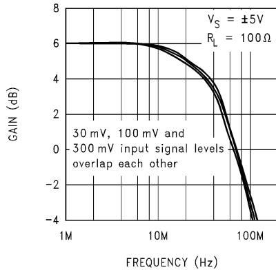
5-78. Closed-Loop Frequency Response vs Input Signal Level
