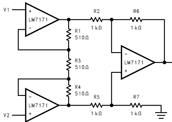
6-2. Fast Instrumentation Amplifier
