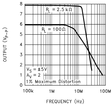
5-88. Undistorted Output Swing vs Frequency
