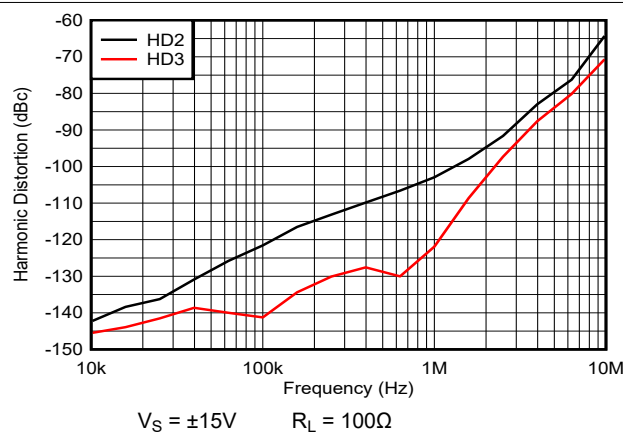
5-36. Total Harmonic Distortion vs Frequency
