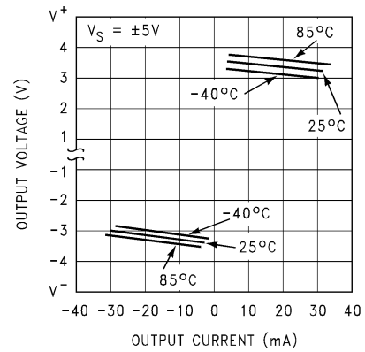
5-47. Output Voltage vs Output Current
