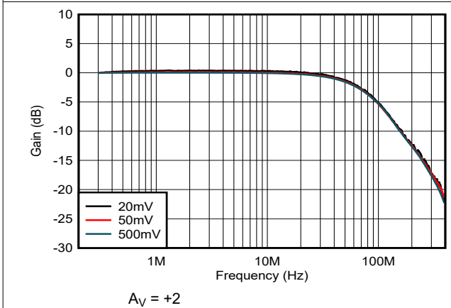
5-35. Closed-Loop Frequency Response vs Input Signal Level
