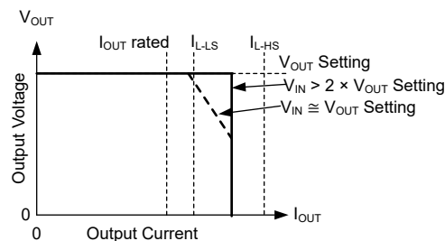
Figure 7-14. Output Voltage Versus Output Current
