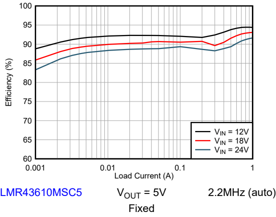
図 8-5. Efficiency
