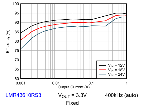
図 8-8. Efficiency
