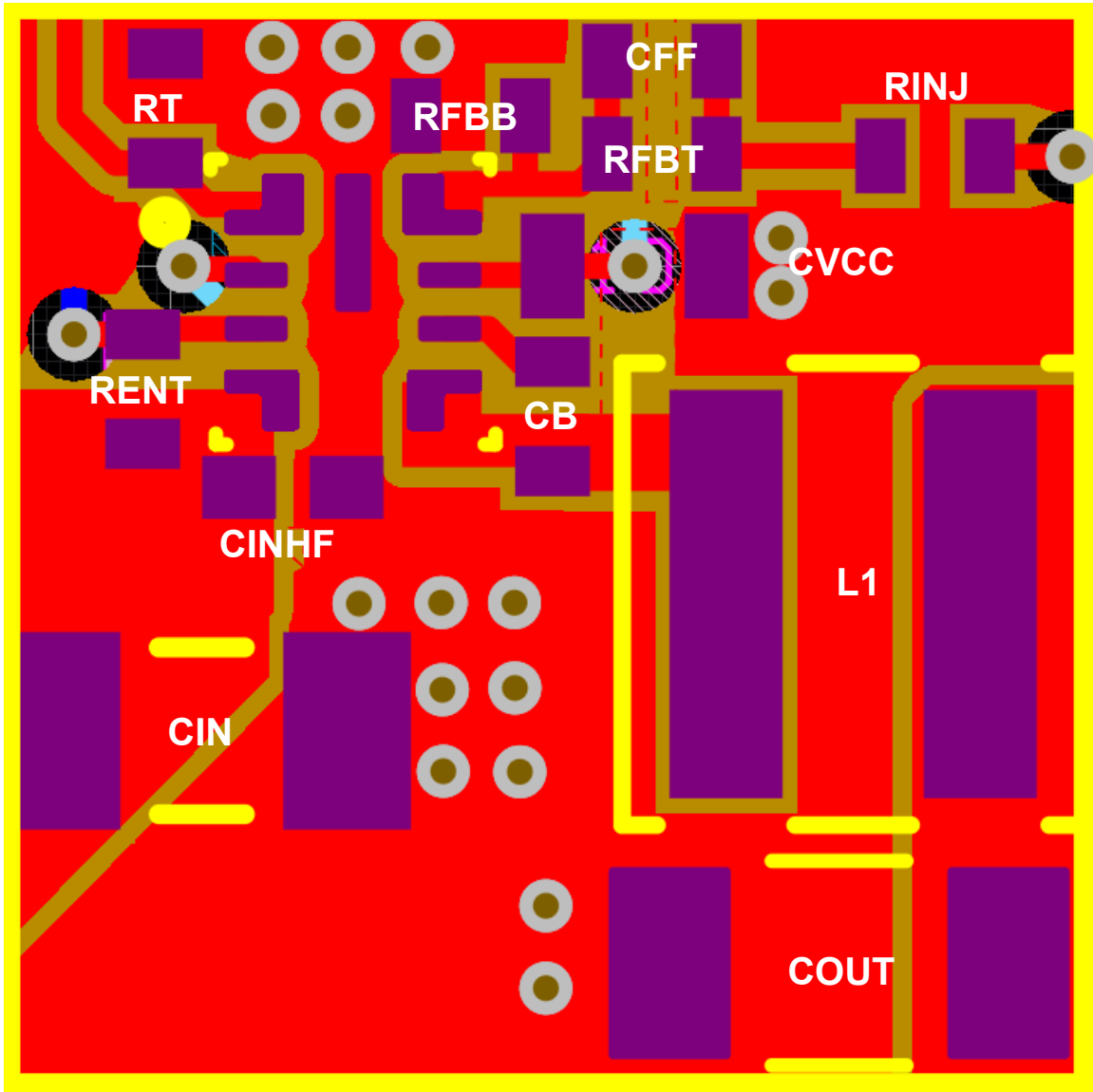
8-32. Example Layout
