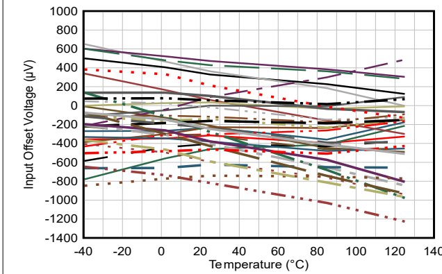
5-1. Offset Voltage Production Distribution
