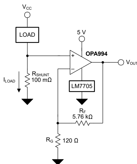
Figure 7-1. OPA994 in a Low-Side, Current-Sensing Application
