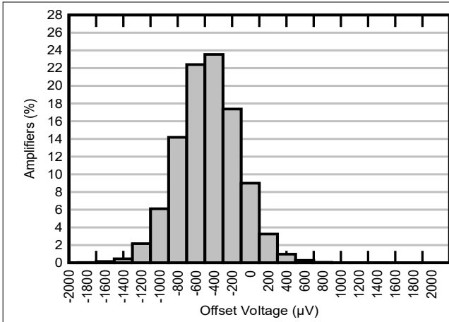
5-1. Offset Voltage Production Distribution
