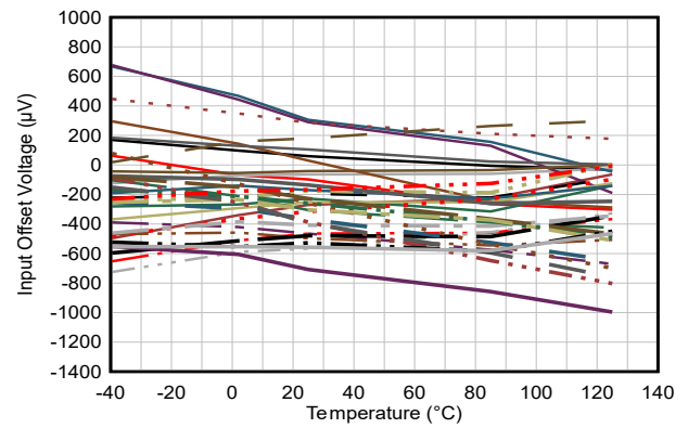
5-2. Offset Voltage Drift Distribution
