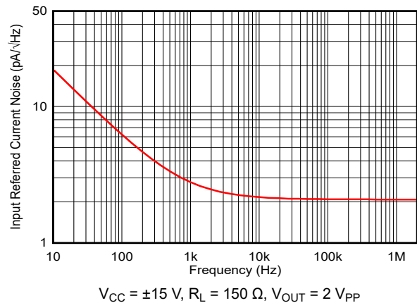
5-12. Input-referred Current Noise vs Frequency
