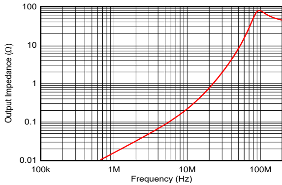
5-7. Closed-loop Output Impedance
