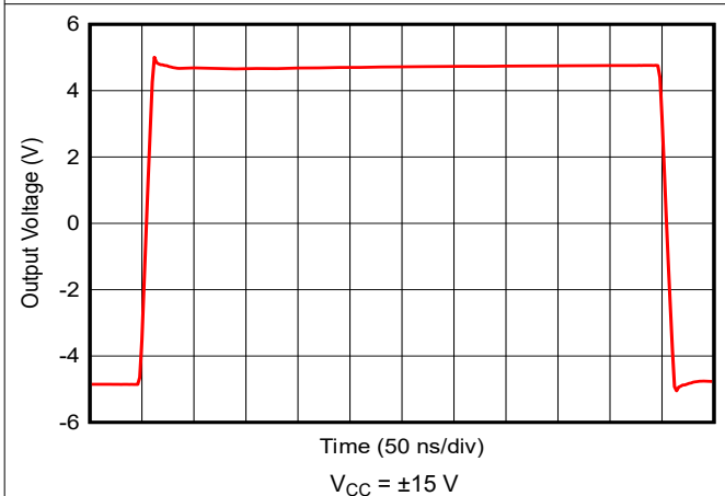
5-23. 10-V Step Response
