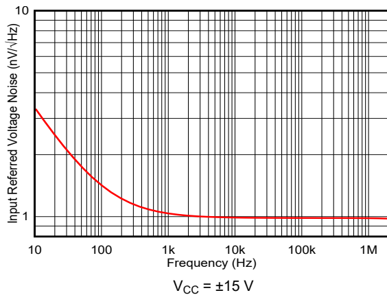
5-11. Input-referred Voltage Noise vs Frequency
