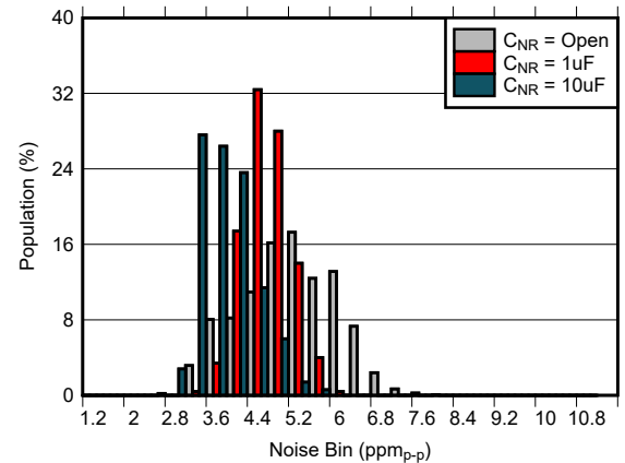
8-10. 0.1 Hz to 10 Hz Noise Distribution vs NR Capacitance
