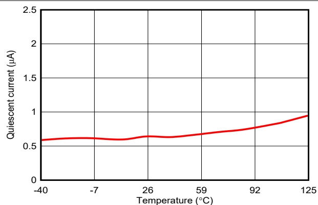
FIG 7-24. Quiescent Current vs Free-Air Temperature
