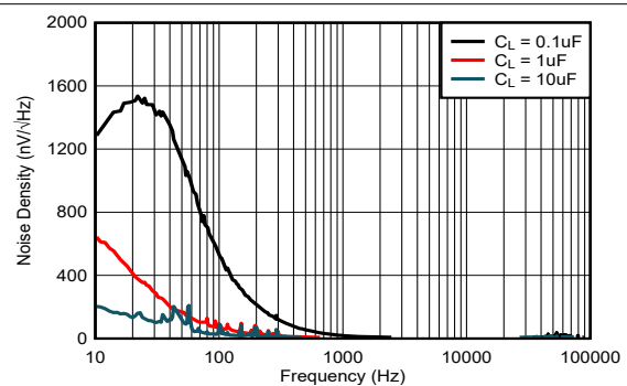
✎ 8-13. Noise Spectrum 10 Hz to 100 kHz ( V_{REF} = 5\text{ V} )
