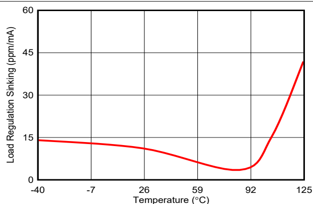
7-12. Load Regulation (Sinking 5 mA) vs Free-Air Temperature
