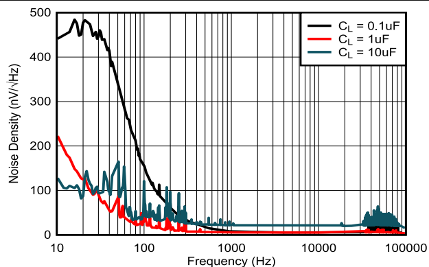
7-8. Noise Density vs Frequency ( V_{REF} = 1.25\text{ V} , I_L = 0\text{ mA} )
