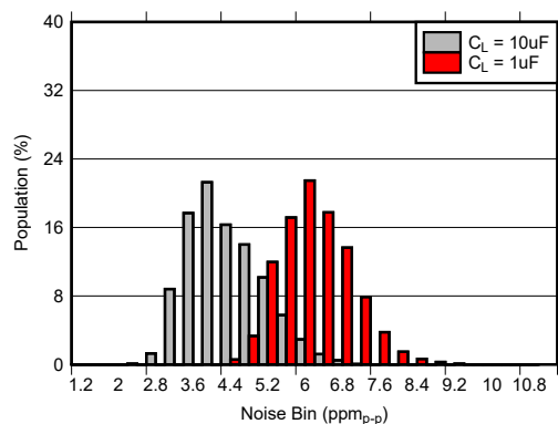
7-7. 0.1 Hz to 10 Hz Noise Distribution ( V_{REF} = 5\text{ V} , C_{NR} = \text{Open} , I_L = 0\text{ mA} )
