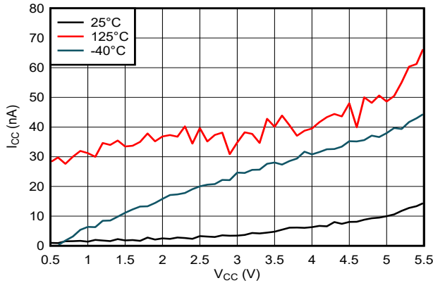
7-3. Supply Current Across Supply Voltage
