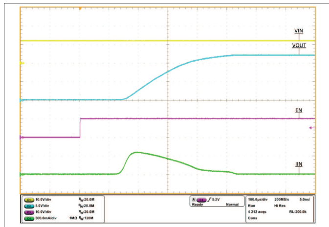
Figure 28. Output Voltage Ramp and Inrush Current at Start Up, C_{dvdt} = \text{Open}
