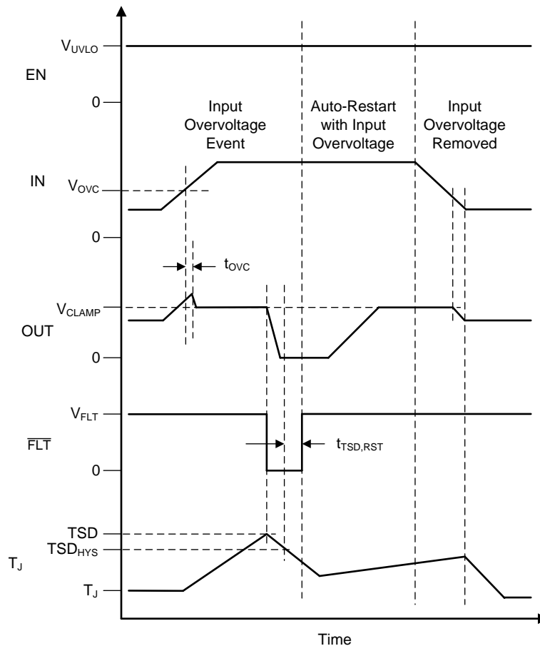
FIG 49. TPS2595xx Overvoltage Clamp Response (Auto-Retry)
