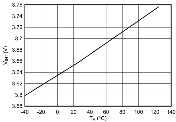
7-15. ITIMER Pin Internal Pullup Voltage Across Temperature
