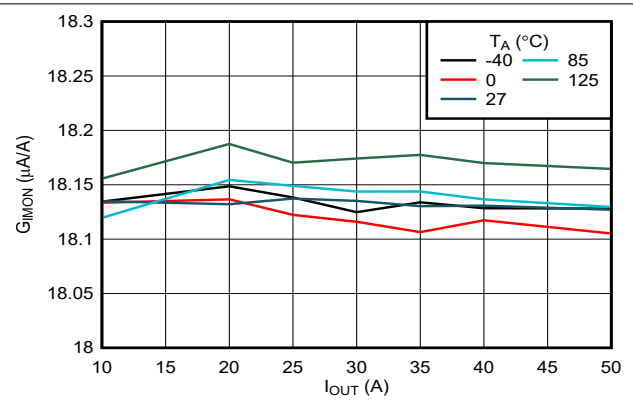
7-8. IMON Gain Across Load and Temperature
