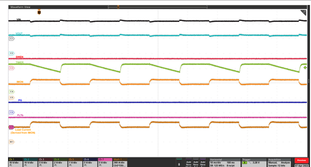
9-9. Transient Overload: V_{IN} = 12 V, C_{TIMER} = 22 nF, C_{LOAD} = 55 mF, R_{IMON} = 167 \Omega , R_{IREF} = 40.2 k \Omega , and Load Current Stepped from 300 A to 400 A then 300 A within 10 ms
