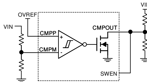
8-11. Fast Overvoltage Protection with Adjustable Threshold Using Internal Comparator
