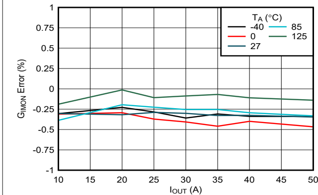
7-9. IMON Gain Accuracy Across Load and Temperature
