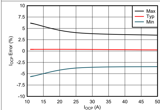
7-11. Steady-State Overcurrent Protection Threshold (Circuit-Breaker) Accuracy
