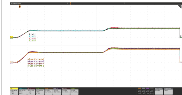
9-12. Circuit-Breaker Response (Current distribution among five devices in parallel): V_{IN} = 12\text{ V} , C_{ITIMER} = 22\text{ nF} , C_{LOAD} = 55\text{ mF} , R_{IMON} = 167\ \Omega , R_{IREF} = 40.2\text{ k}\Omega , and Load Current Stepped up From 300 A to 475 A for > 20 ms
