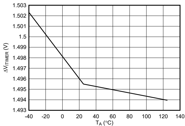
7-17. ITIMER Pin Discharge Differential Voltage Threshold Across Temperature
