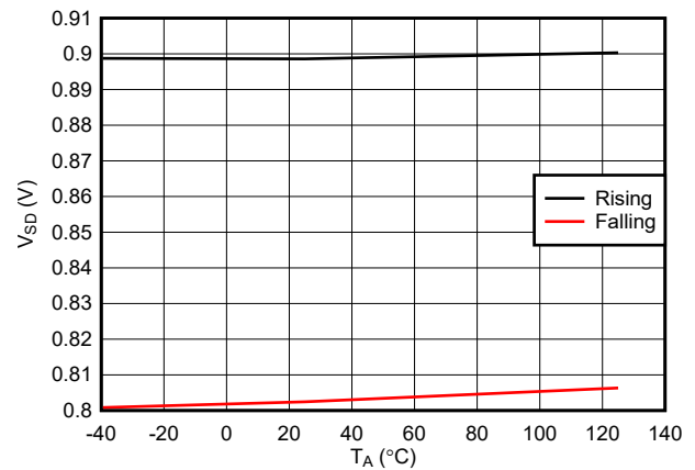
7-6. EN/UVLO Based Shutdown Falling Threshold Across Temperature
