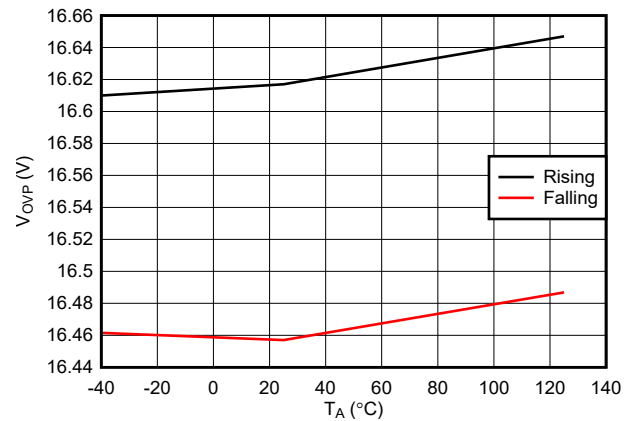
7-4. Overvoltage Protection Threshold Across Temperature
