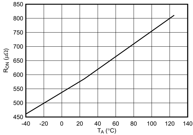
7-1. ON Resistance Across Temperature
