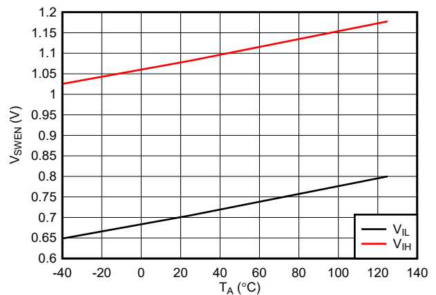
7-18. SWEN Pin Logic Thresholds Across Temperature
