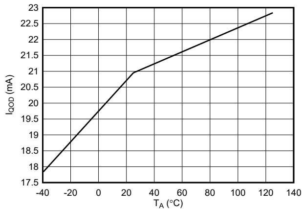
7-21. QOD Sink Current Across Temperature
