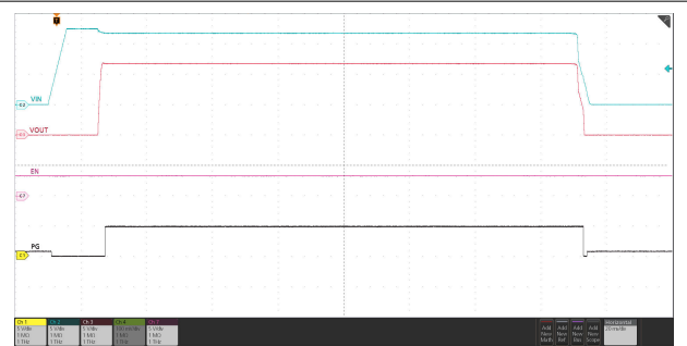
7-24. Power Up and Down Sequencing Using Input Supply
