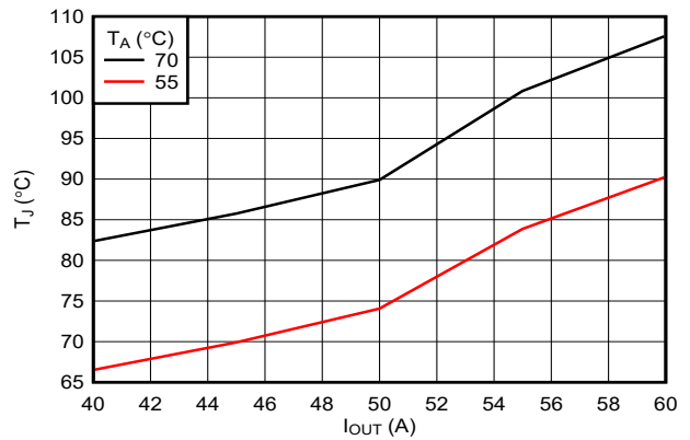
7-22. Junction Temperature vs Load Current (No Air-Flow)
