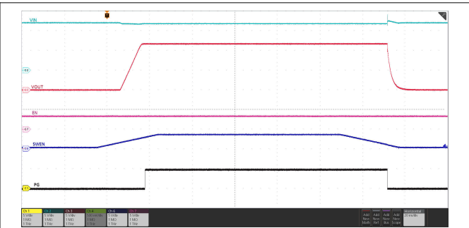
7-26. Power Up and Down Sequencing Using SWEN Pin
