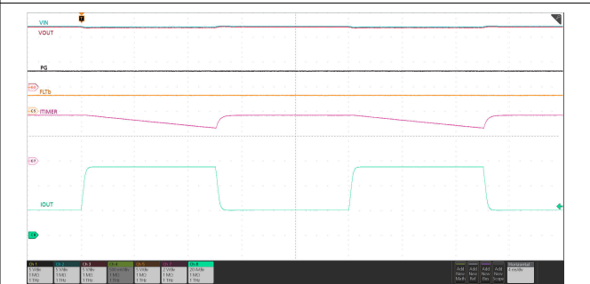
7-28. Inrush Current Control with Capacitive and Resistive Load
