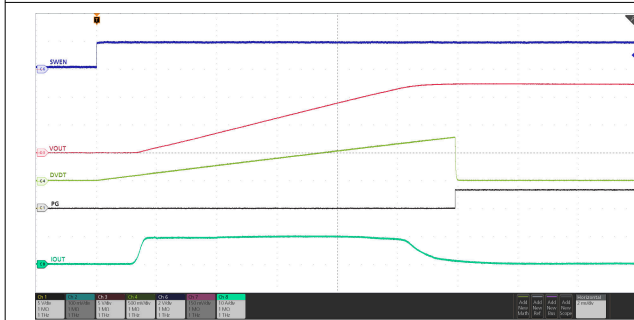
7-27. Inrush Current Control with Capacitive Load
