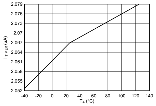
7-16. ITIMER Pin Discharge Current Across Temperature
