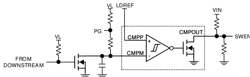
8-12. Load Handshake or Detect Timer Using Internal Comparator
