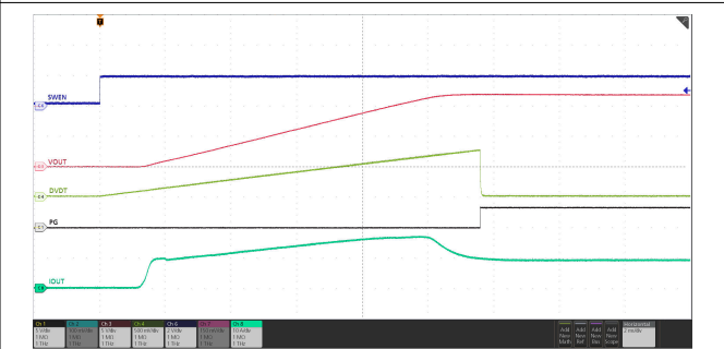
7-26. Power Up and Down Sequencing Using SWEN Pin
