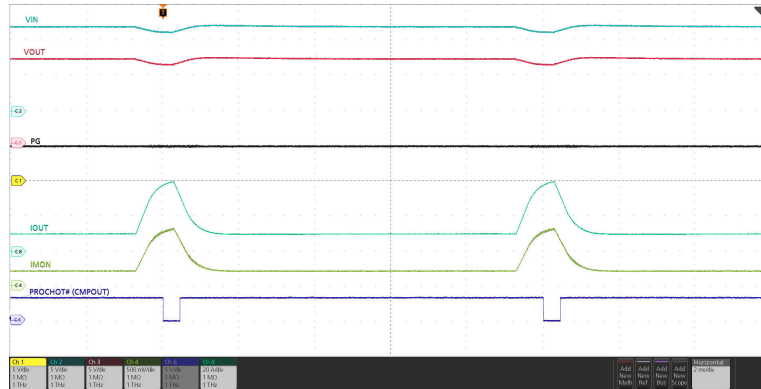
8-10. PROCHOT# Response Using Internal Comparator
