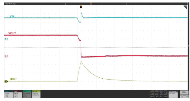
9-13. Output Hot-Short Response: V_{IN} = 12\text{ V} , R_{IMON} = 167\ \Omega , R_{IREF} = 40.2\text{ k}\Omega , and OUT Shorted to GND
