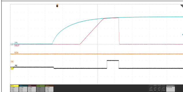
7-29. Input Overvoltage Protection Response
