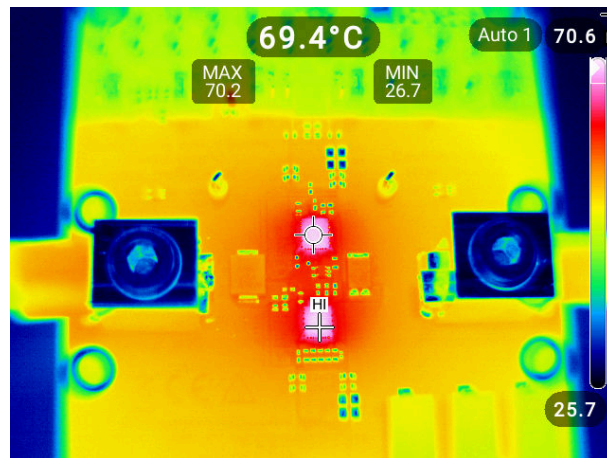
9-14. Two (2) TPS25985x eFuses in Parallel: Temperature Rise with 100-A DC Current at Room Temperature (No Air-Flow)
