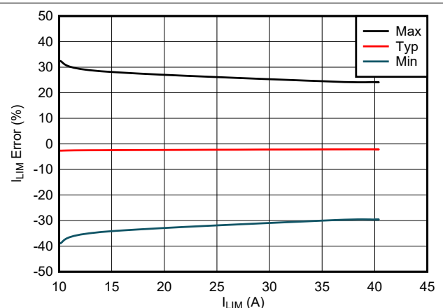
7-12. Start-up Overcurrent Protection Threshold (Current Limit) Accuracy
