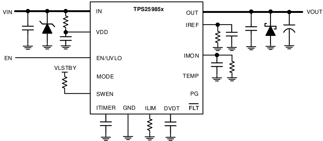
10-1. Circuit Implementation with Optional Protection Components
