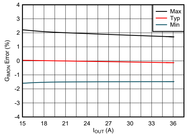
7-10. IMON Gain Accuracy Across Process and Temperature Corners
