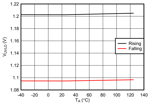
7-5. EN/UVLO Thresholds Across Temperature
