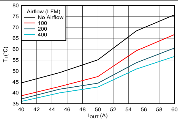
7-23. Junction Temperature vs Load Current (T A = 25°C, With Air-Flow)
