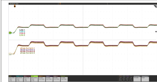
9-10. Transient Overload (Current distribution among five devices in parallel): V_{IN} = 12\text{ V} , C_{ITIMER} = 22\text{ nF} , C_{LOAD} = 55\text{ mF} , R_{IMON} = 167\ \Omega , R_{IREF} = 40.2\text{ k}\Omega , and Load Current Stepped from 300 A to 450 A then 300 A within 8.5 ms
