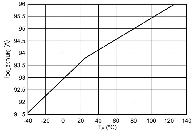
7-14. Backup Overcurrent Protection Threshold (Steady-State) Accuracy
