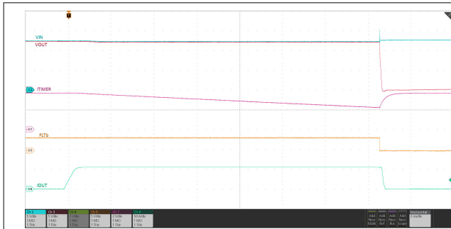
7-31. Overcurrent Protection Response (Circuit-Breaker)
