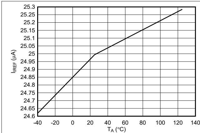
7-7. IREF Charging Current Across Temperature
