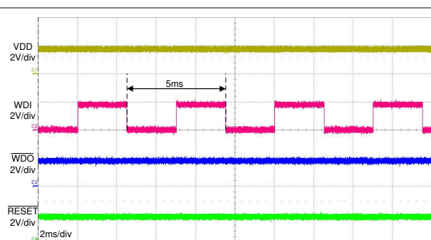
Figure 8-6. Typical WDI Signal
