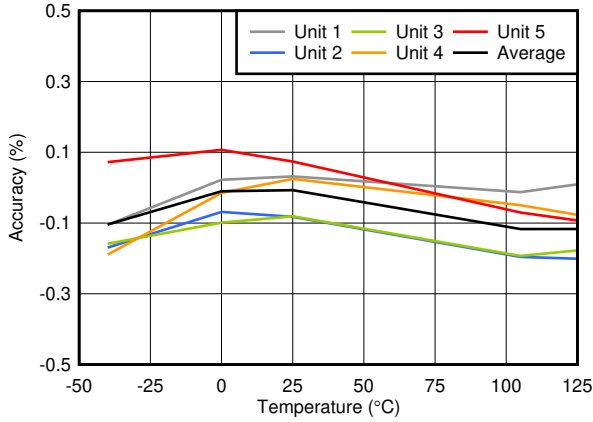
6-9. V_{ITN} Accuracy vs Temperature
