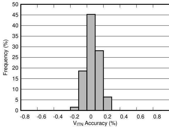
6-11. V_{ITN} Accuracy Histogram
