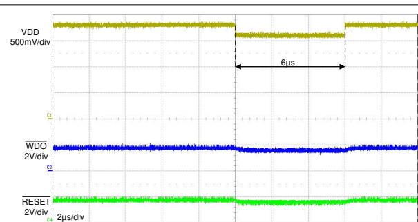
Figure 8-8. High-to-Low Glitch Immunity
