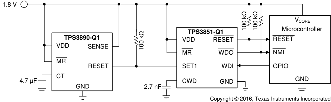
8-3. Monitoring the Supply Voltage and Watchdog Supervision of a Microcontroller
