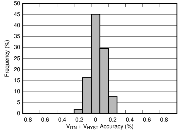
6-10. V_{ITN} + V_{HYST} Accuracy Histogram
