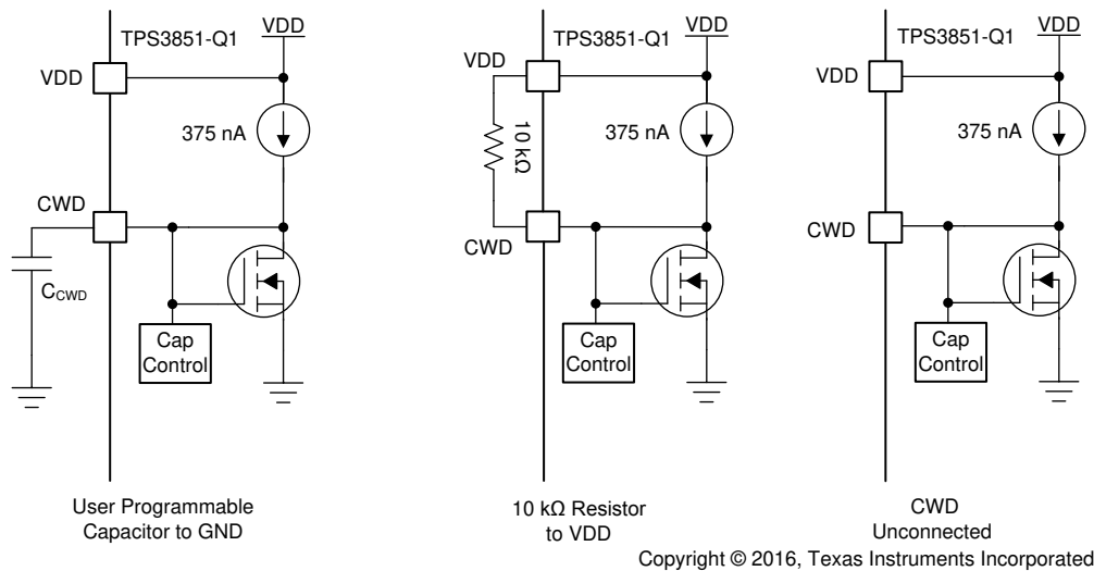
図 8-1. CWD Charging Circuit
