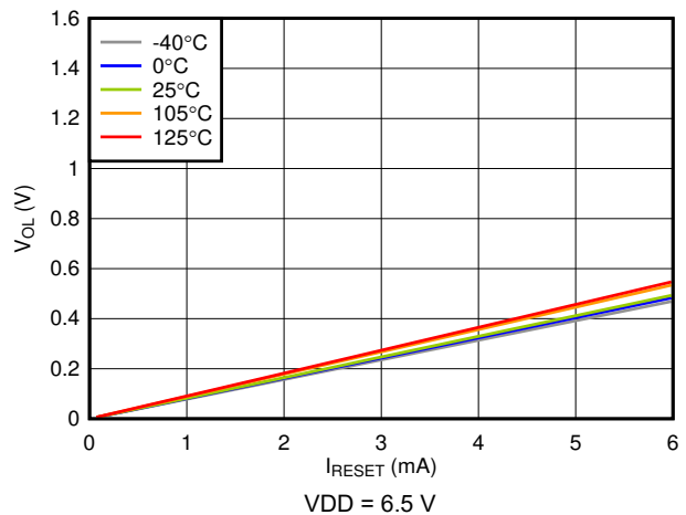
6-14. Low-Level RESET Voltage vs RESET Current
