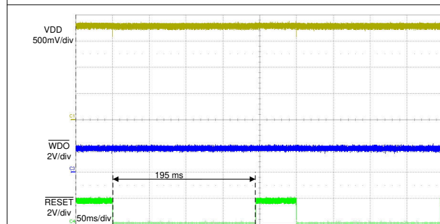
Figure 8-7. Typical \overline{\text{RESET}} Delay
