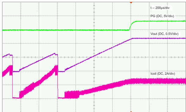
9-18. Output Short-Circuit Protection, Load = 0.47 \Omega , Recovery
