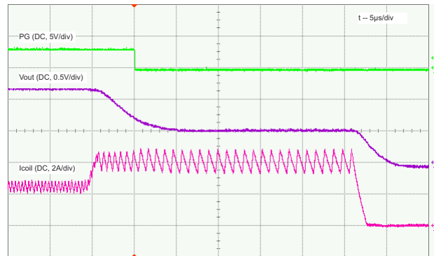
9-19. Output Short-Circuit Protection, Load = 0.47 \Omega , HICCUP Zoom In
