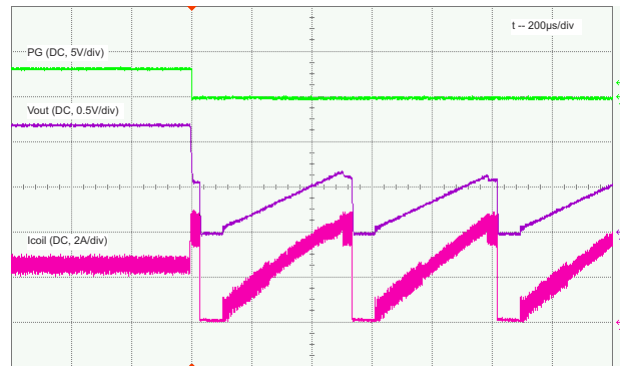
9-17. Output Short-Circuit Protection, Load = 0.47 \Omega , Entry
