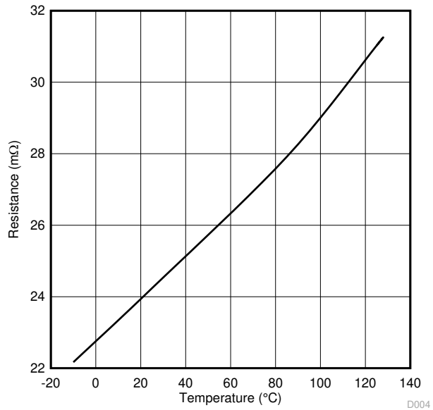
图 6-1. PPHVx Rdson vs Junction Temperature D004
