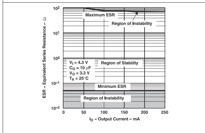
5-56. Typical Region of Stability ESR vs Output Current (Legacy Chip)
