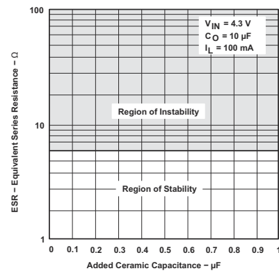
5-47. TPS76933-Q1 Typical Regions of Stability ESR vs Added Ceramic Capacitance (Legacy Chip)
