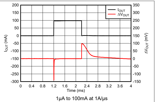
图 5-44. TPS76933-Q1 Load Transient Response (New Chip)
