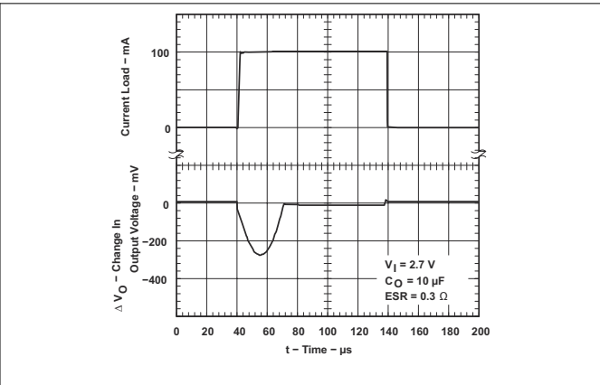
Figure 5-38. TPS76915-Q1 Load Transient Response (Legacy Chip)
