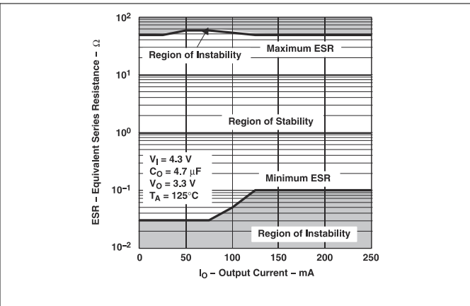
5-53. Typical Region of Stability ESR vs Output Current (Legacy Chip)
