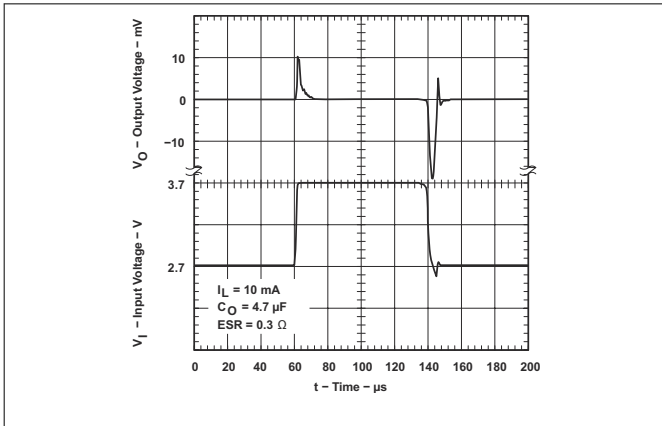
Figure 5-37. TPS76915-Q1 Line Transient Response (Legacy Chip)
