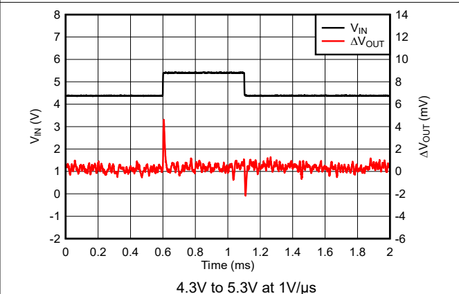
Figure 5-40. TPS76933-Q1 Line Transient Response (New Chip)
