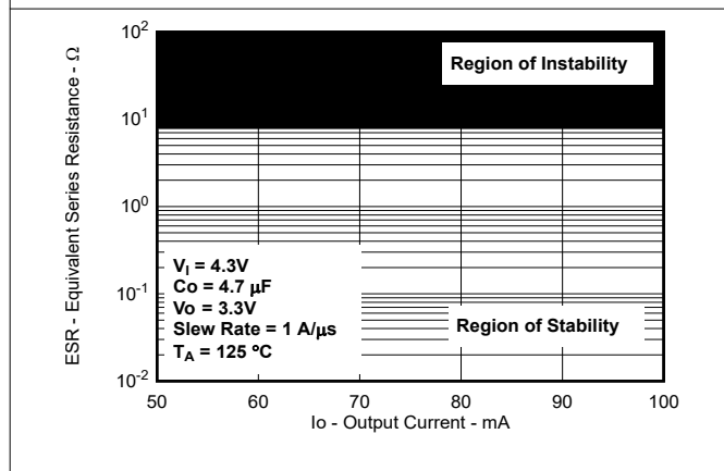
5-54. Typical Region of Stability ESR vs Output Current (New Chip)
