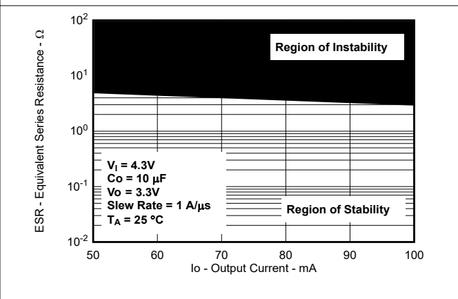
5-57. Typical Region of Stability ESR vs Output Current (New Chip)
