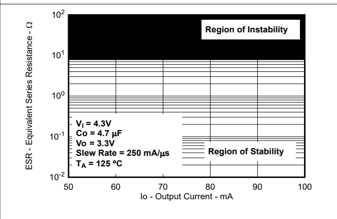
5-55. Typical Region of Stability ESR vs Output Current (New Chip)
