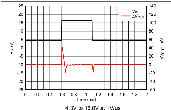
Figure 5-41. TPS76933-Q1 Line Transient Response (New Chip)
