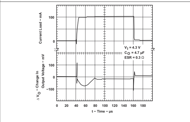
Figure 5-42. TPS76933-Q1 Load Transient Response (Legacy Chip)
