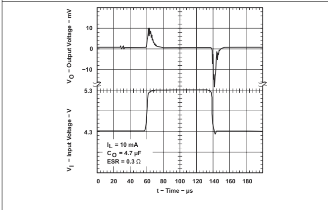
Figure 5-39. TPS76933-Q1 Line Transient Response (Legacy Chip)
