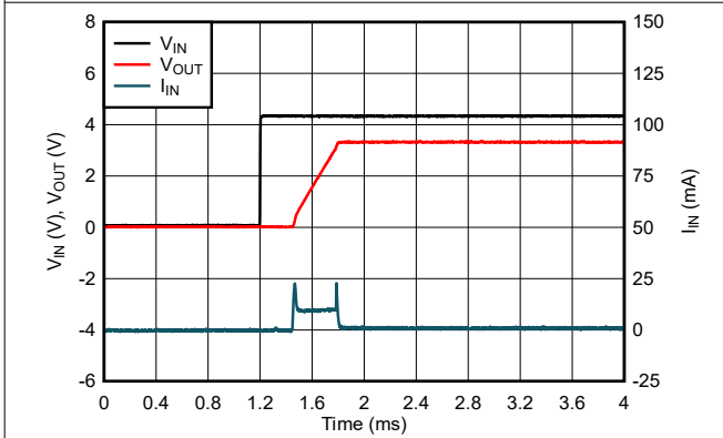
7-4. Power-Up Waveform (Legacy Chip)
