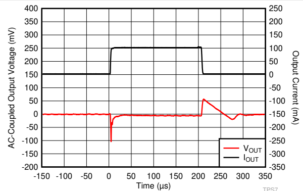
6-14. I_{OUT} Transient From 1 mA to 100 mA
