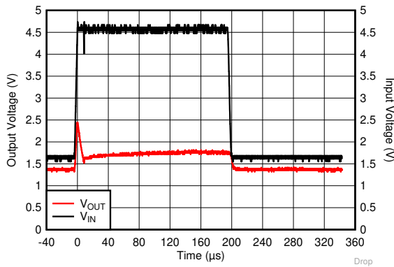
6-25. V_{IN} Transient From 1.5 V to 4.5 V
