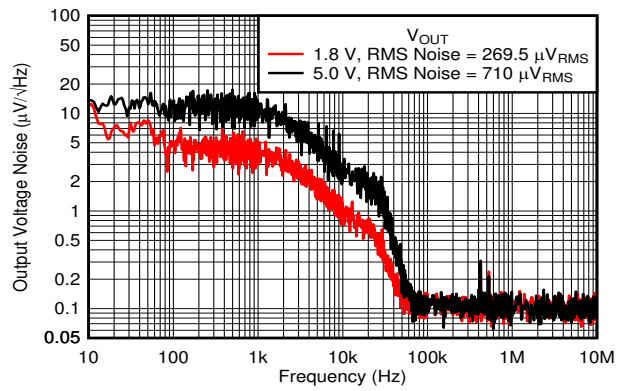
6-48. Output Noise vs Frequency and V_{OUT} V_{IN} = V_{OUT} + 1.0\text{ V} , I_{OUT} = 1\text{ mA} , C_{OUT} = 1\text{ }\mu\text{F} V_{OUT} = 1.8\text{ V} , RMS Noise = 269.5\text{ }\mu\text{V}_{RMS} V_{OUT} = 5.0\text{ V} , RMS Noise = 710\text{ }\mu\text{V}_{RMS}
