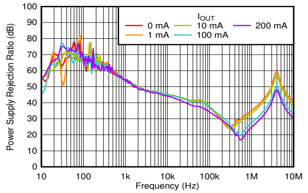
6-44. PSRR vs Frequency and I_{OUT} V_{IN} = 2.8\text{ V} , V_{OUT} = 1.8\text{ V} , C_{OUT} = 1\text{ }\mu\text{F}
