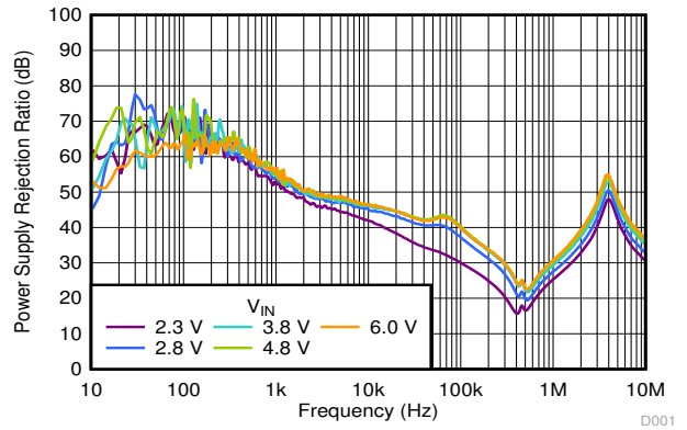
6-46. PSRR vs Frequency and V_{IN} V_{OUT} = 1.8\text{ V} , I_{OUT} = 100\text{ mA} , C_{OUT} = 1\text{ }\mu\text{F}
