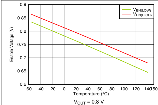
6-39. EN High and Low Threshold vs Temperature
