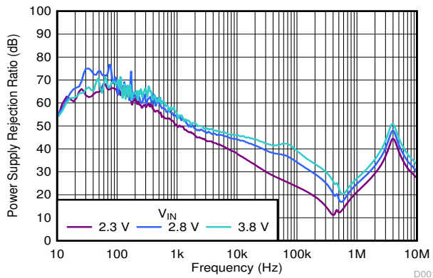
6-47. PSRR vs Frequency and V_{IN} V_{OUT} = 1.8\text{ V} , I_{OUT} = 200\text{ mA} , C_{OUT} = 1\text{ }\mu\text{F}
