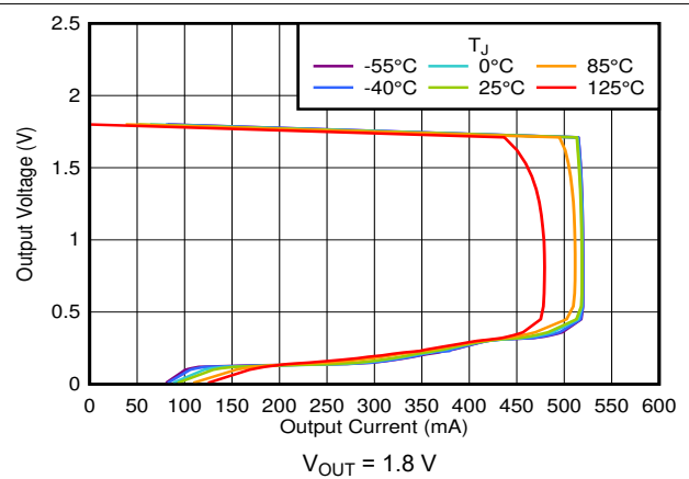
6-38. Foldback Current Limit vs I_{OUT} and Temperature
