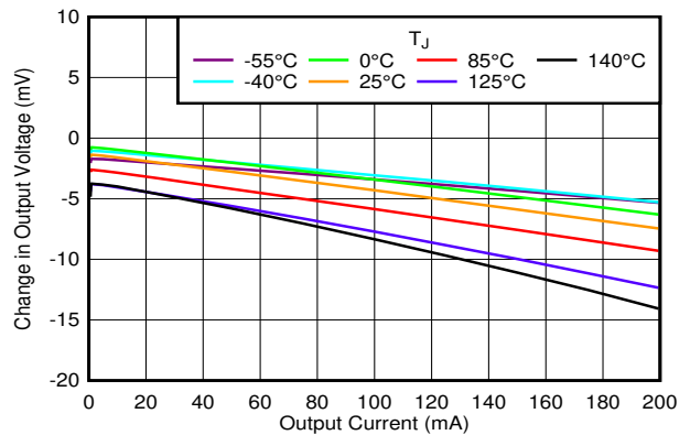
6-32. Load Regulation vs V_{IN} and Temperature
