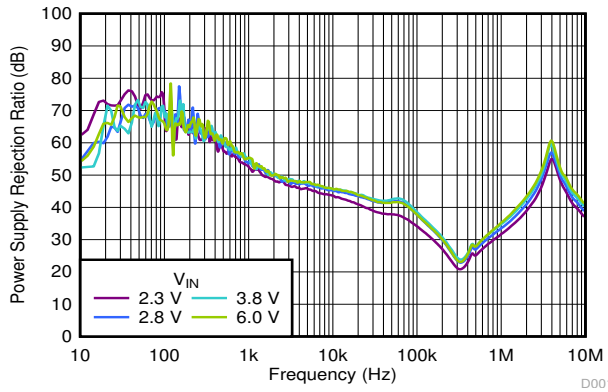
6-45. PSRR vs Frequency and V_{IN} V_{OUT} = 1.8\text{ V} , I_{OUT} = 10\text{ mA} , C_{OUT} = 1\text{ }\mu\text{F}
