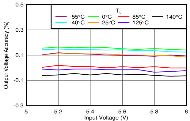
6-28. Output Accuracy vs Temperature
