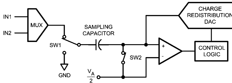
FIGURE 1. ADC082S051 in Track Mode
