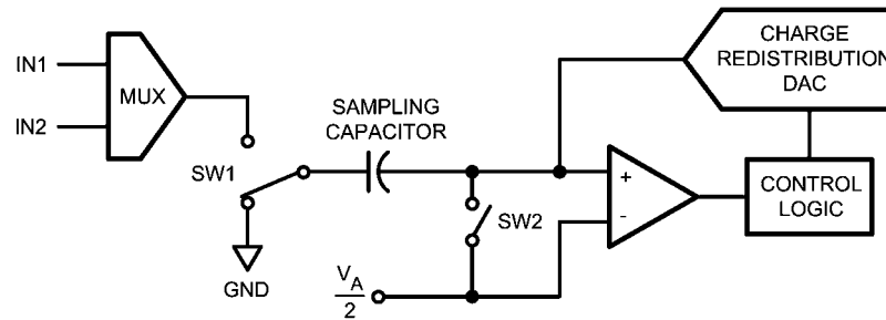
FIGURE 2. ADC082S051 in Hold Mode
