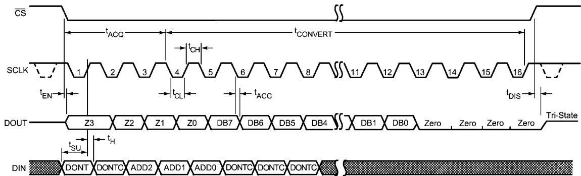
ADC082S051 Serial Timing Diagram
