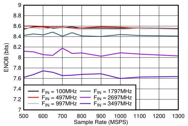
5-24. ENOB vs Sample Rate
