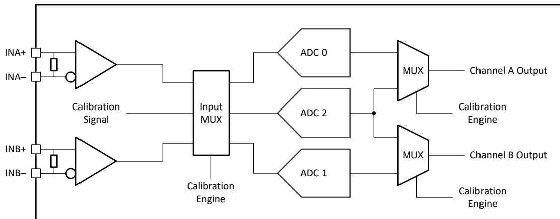
6-16. DualChannel Calibration System Block Diagram
