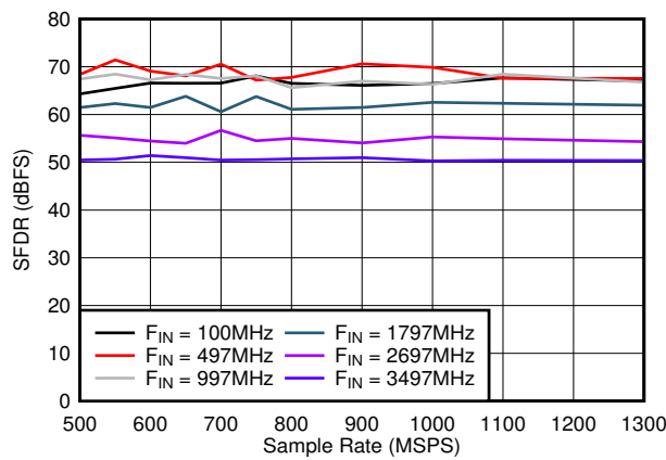
5-21. SFDR vs Sample Rate
