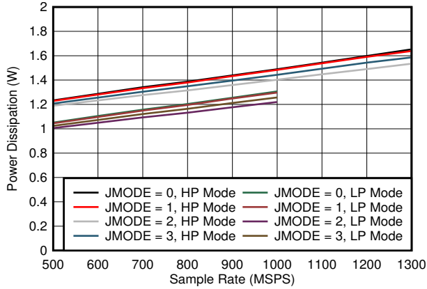
5-91. Dual Channel, Power Dissipation vs FS for JMODES 0 - 3
