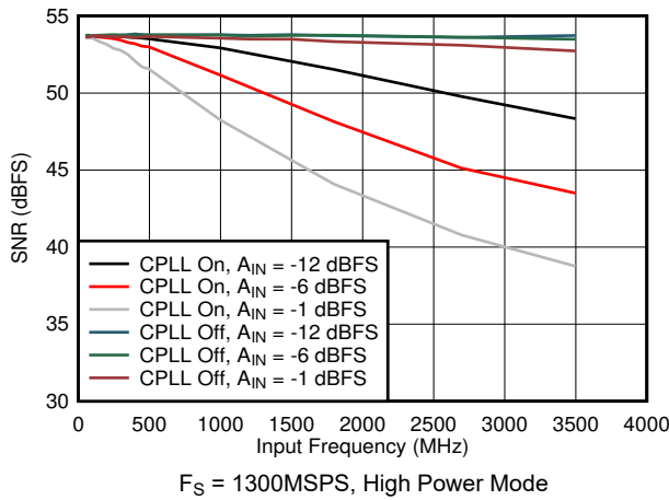
5-69. SNR vs Input Frequency, CPLL and Input Amplitude
