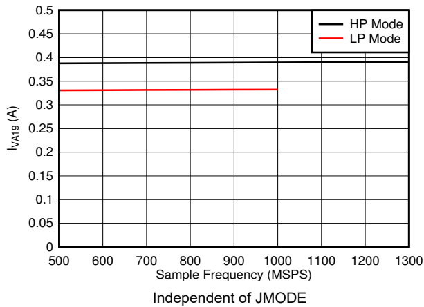
5-95. Dual Channel, I_{VA19} vs FS
