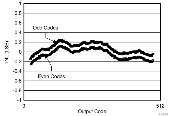
5-2. INL vs Code
