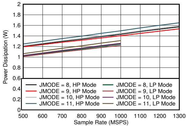
5-93. Dual Channel, Power Dissipation vs FS for JMODES 8 - 11
