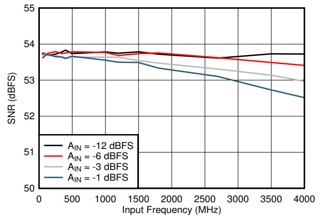
图 5-16. SNR vs Input Frequency
