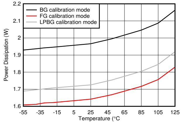
5-124. Dual Channel, Power Dissipation vs Temperature
