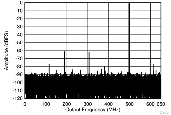
図 5-8. Single Tone FFT at 1797 MHz and -1 dBFS
