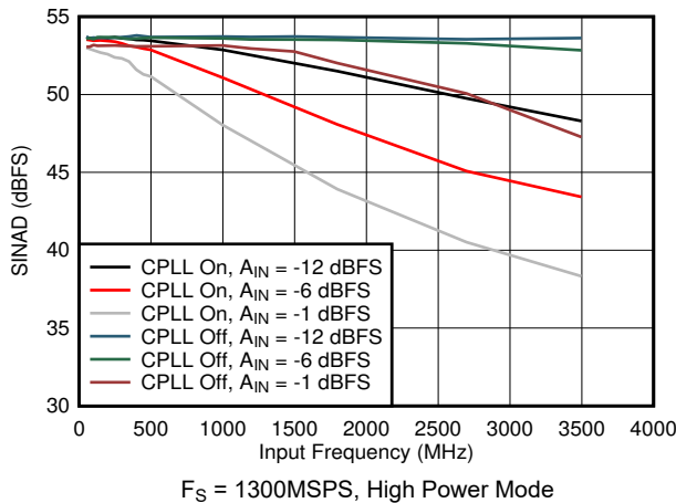
5-71. SINAD vs Input Frequency, CPLL and Input Amplitude
