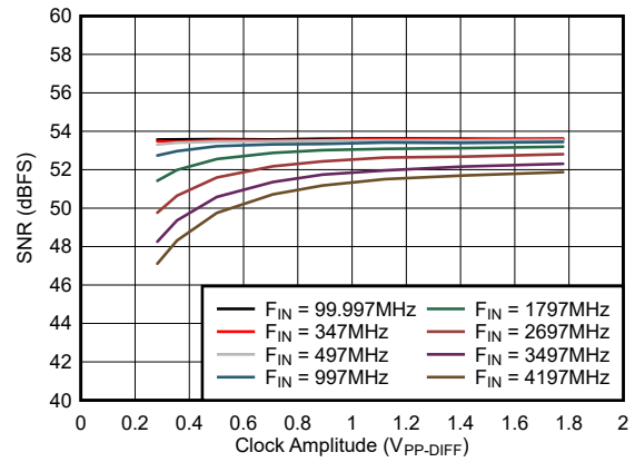
5-34. SNR vs Clock Amplitude
