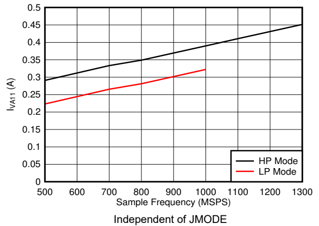
5-96. Dual Channel, I_{VA11} vs FS
