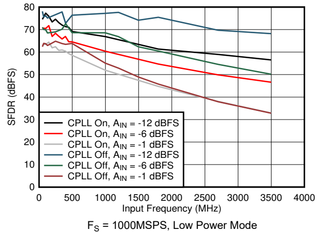
5-76. SFDR vs Input Frequency, CPLL and Input Amplitude
