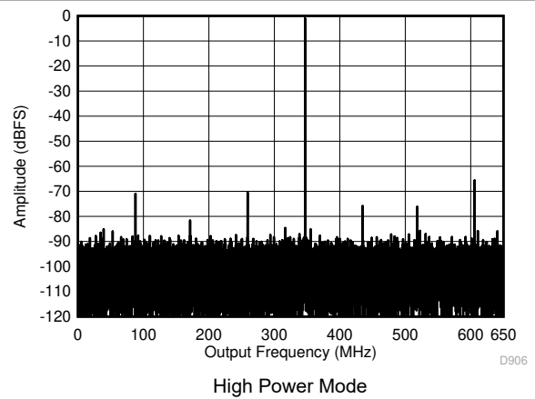
5-4. Single Tone FFT at 347 MHz and -1 dBFS
