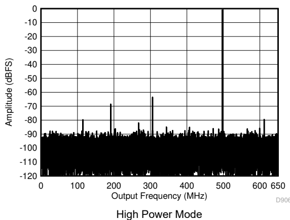
5-5. Single Tone FFT at 497 MHz and -1 dBFS
