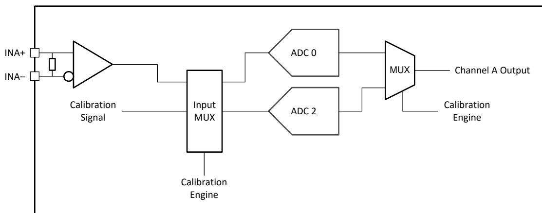
6-17. Single Channel Calibration System Block Diagram
