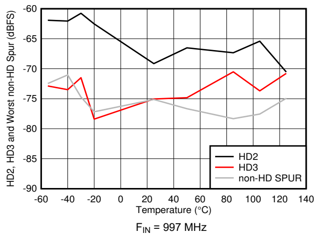
5-36. HD2, HD3 and worst non-HD Spur vs Temperature
