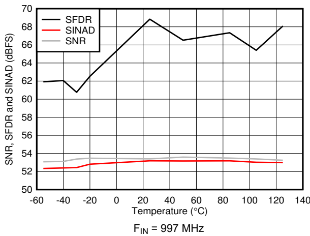
5-35. SNR, SFDR and SINAD vs Temperature
