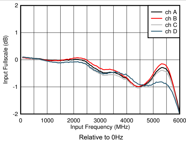
5-3. Input Fullscale vs Input Frequency
