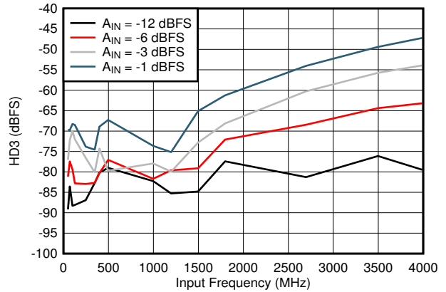
5-20. HD3 vs Input Frequency
