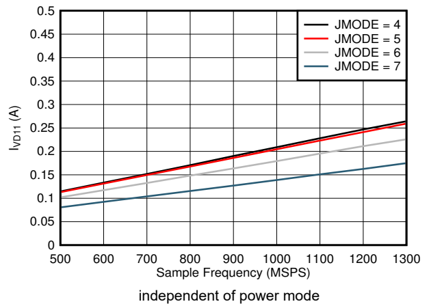
5-108. Single Channel, I_{VD11} vs FS and JMODE 4 - 7
