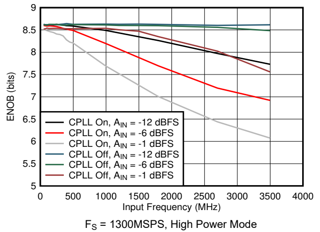
5-72. ENOB vs Input Frequency, CPLL and Input Amplitude
