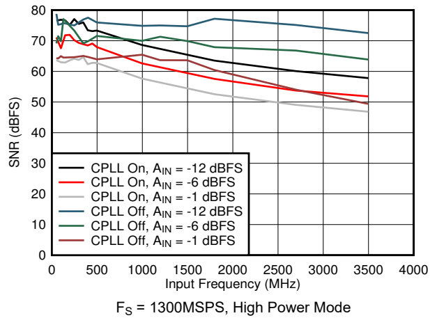
5-70. SFDR vs Input Frequency, CPLL and Input Amplitude
