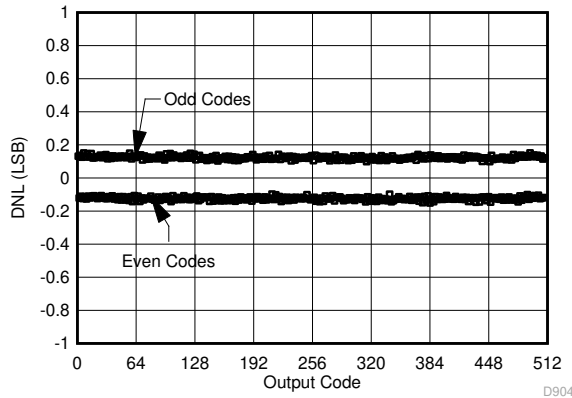
5-1. DNL vs Code
