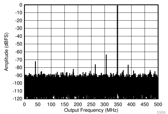
図 5-10. Single Tone FFT at 3497 MHz and -1 dBFS
