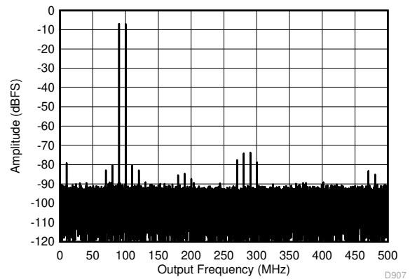
5-52. Two Tone FFT at 1798 MHz Center
