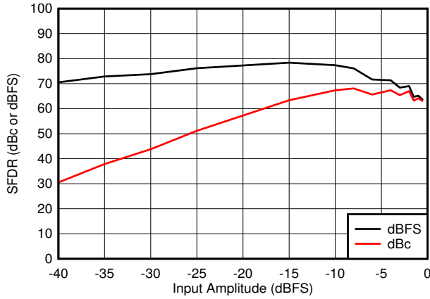
5-31. SFDR vs Input Amplitude
