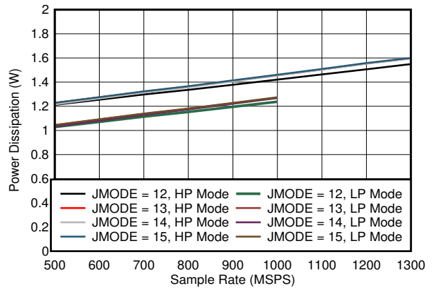
5-94. Dual Channel, Power Dissipation vs FS for JMODES 12 - 15
