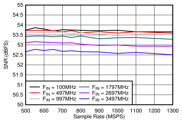
5-22. SNR vs Sample Rate
