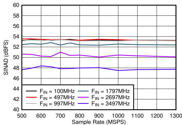
5-23. SINAD vs Sample Rate
