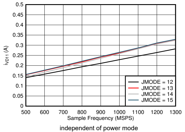
5-100. Dual Channel, I_{VD11} vs FS and JMODE 12 - 15
