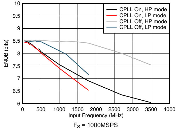
5-68. ENOB vs Input Frequency and CPLL
