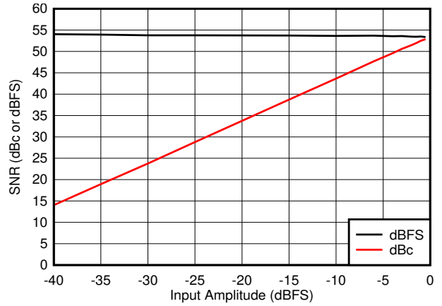
5-32. SNR vs Input Amplitude
