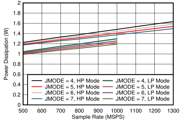
5-92. Dual Channel, Power Dissipation vs FS for JMODES 4 - 7
