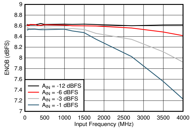
图 5-18. ENOB vs Input Frequency
