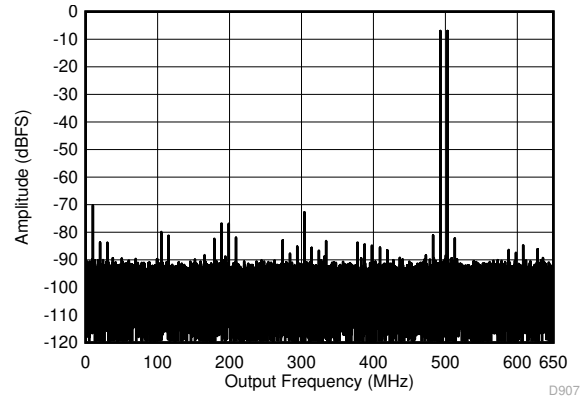
5-50. Two Tone FFT at 498 MHz Center
