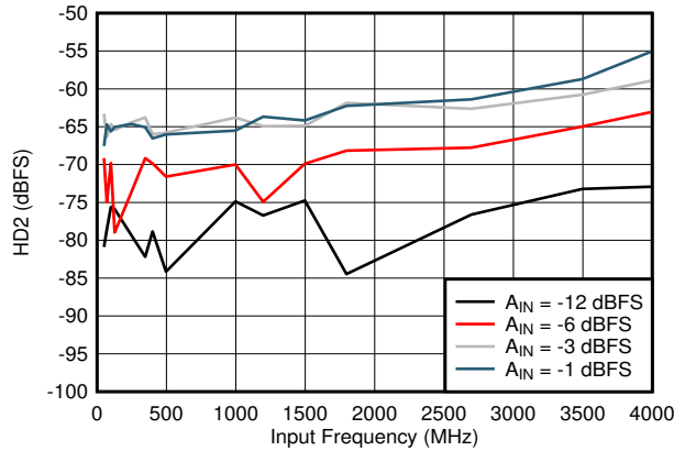
5-19. HD2 vs Input Frequency
