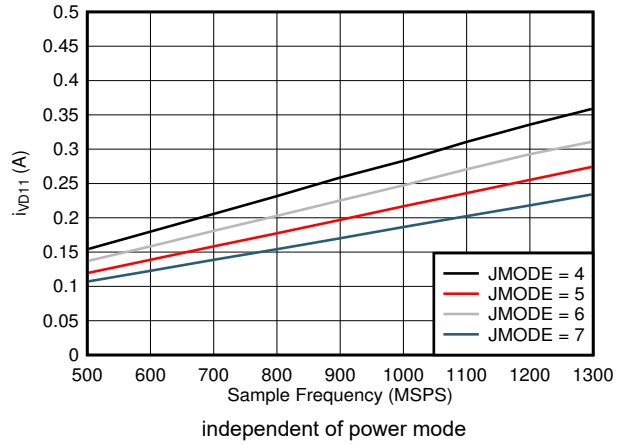
5-98. Dual Channel, I_{VD11} vs FS and JMODE 4 - 7
