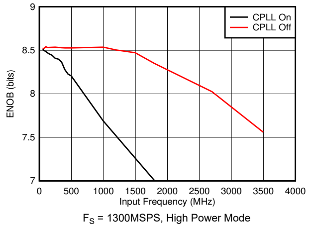
7-64. ENOB vs Input Frequency and CPLL
