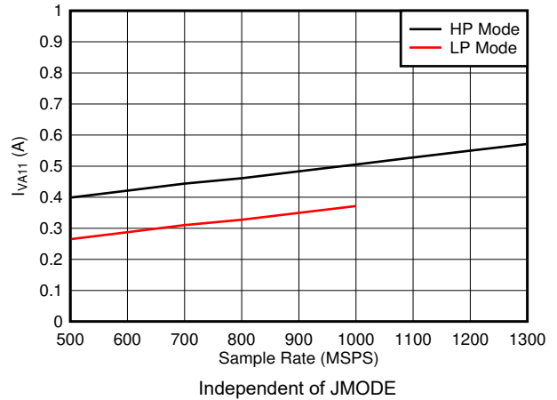
7-86. Quad Channel, I_{VA11} vs FS
