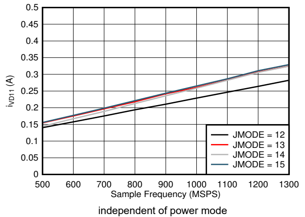
7-100. Dual Channel, I_{VD11} vs FS and JMODE 12 - 15
