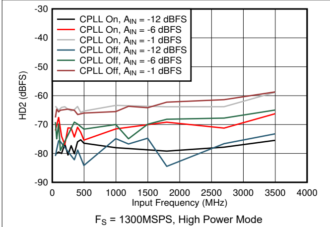
7-73. HD2 vs Input Frequency, CPLL and Input Amplitude
