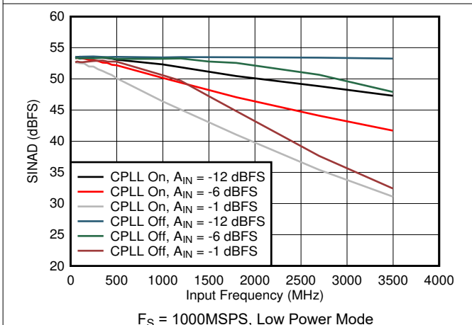
7-77. SINAD vs Input Frequency, CPLL and Input Amplitude
