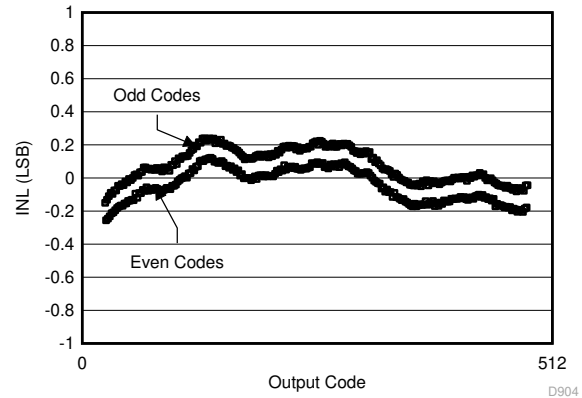
7-2. INL vs Code
