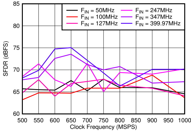
7-25. SFDR vs Sample Rate
