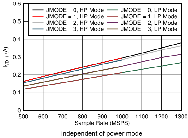
7-97. Dual Channel, I_{VD11} vs FS and JMODE 0 - 3
