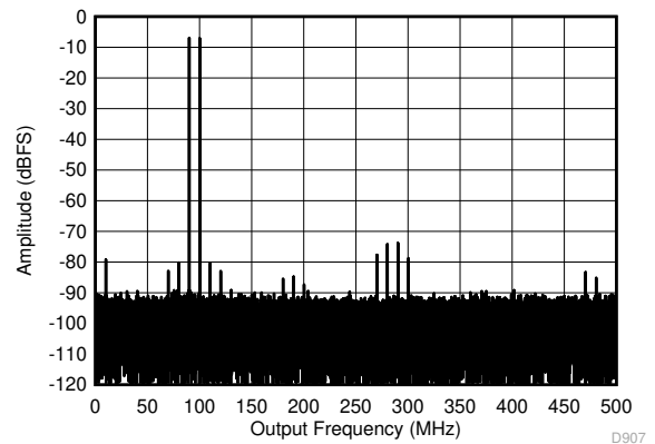
7-52. Two Tone FFT at 1798 MHz Center
