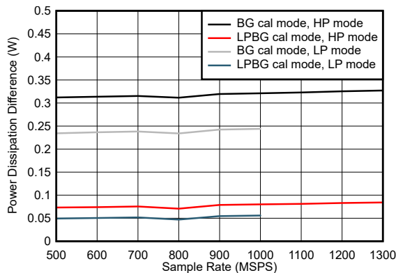
7-111. Quad Channel, Power Dissipation Change with Calibration Mode
