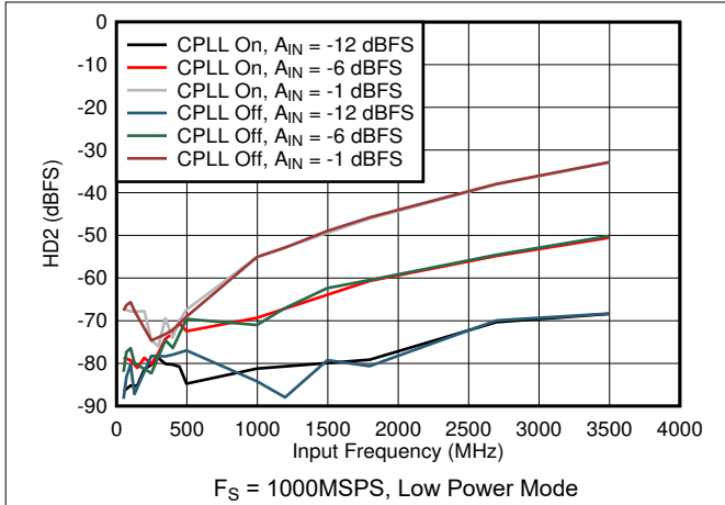
7-79. HD2 vs Input Frequency, CPLL and Input Amplitude
