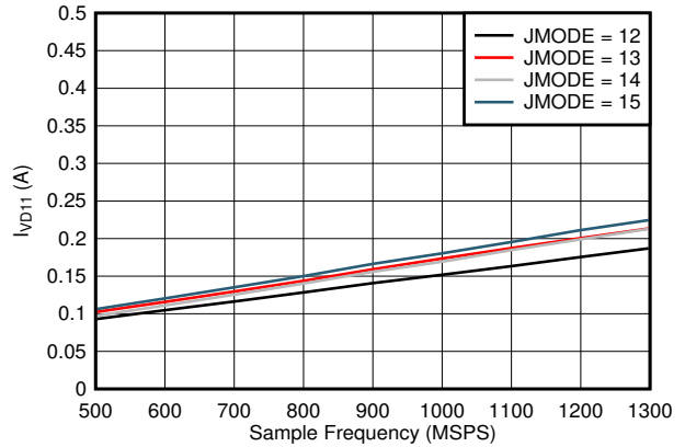
7-110. Single Channel, I_{VD11} vs FS and JMODE 12 - 15
