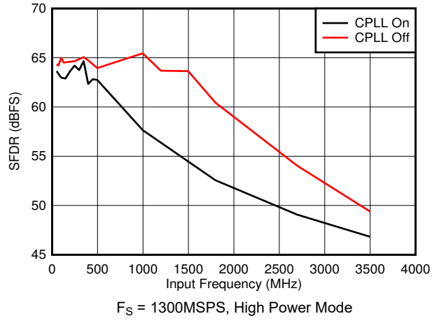
7-62. SFDR vs Input Frequency and CPLL
