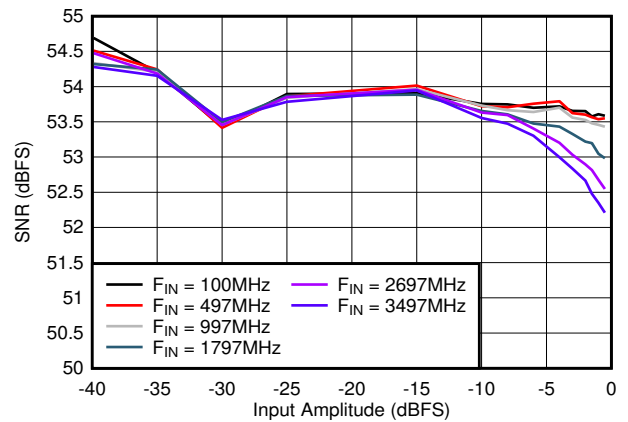
7-30. SNR vs Input Amplitude
