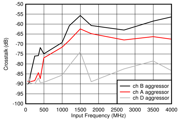
7-60. Crosstalk to Channel B vs F_{IN}
