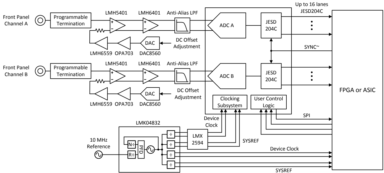
9-3. Typical Configuration for Reconfigurable Oscilloscope
