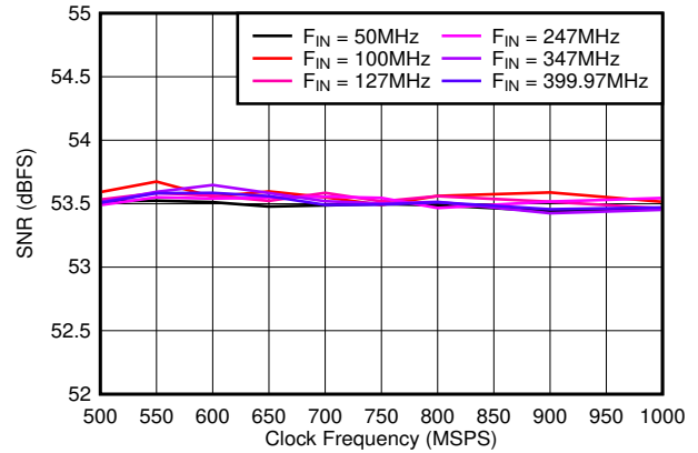
7-26. SNR vs Sample Rate
