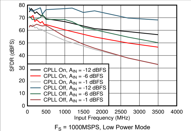
7-76. SFDR vs Input Frequency, CPLL and Input Amplitude
