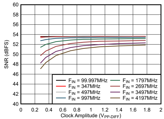
7-34. SNR vs Clock Amplitude
