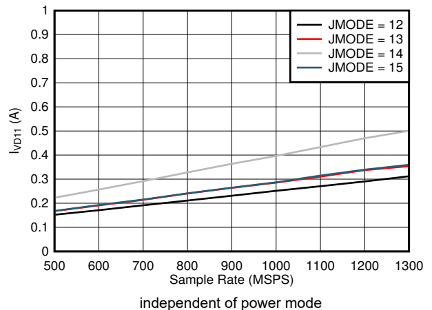
7-90. Quad Channel, I_{VD11} vs FS and JMODE 12 - 15
