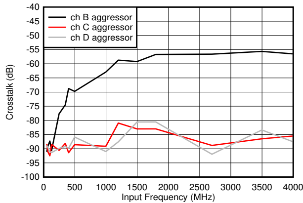
7-59. Crosstalk to Channel A vs F_{IN}
