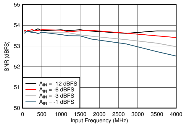
7-16. SNR vs Input Frequency
