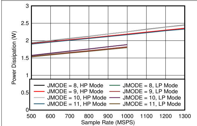
7-83. Quad Channel, Power Dissipation vs FS for JMODES 8 - 11
