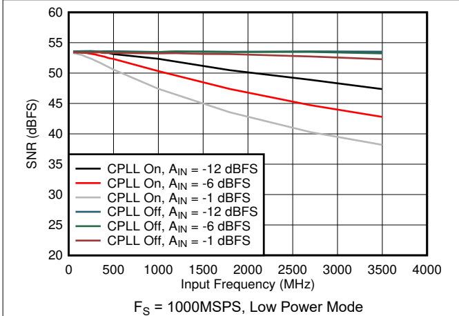
7-75. SNR vs Input Frequency, CPLL and Input Amplitude
