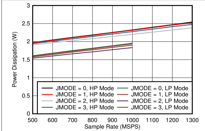
7-81. Quad Channel, Power Dissipation vs FS for JMODES 0 - 3
