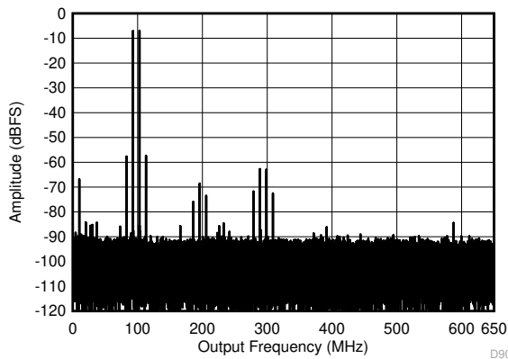
7-51. Two Tone FFT at 998 MHz Center
