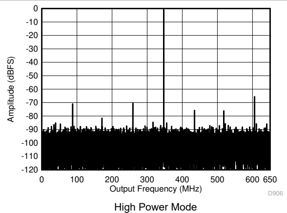
7-4. Single Tone FFT at 347 MHz and -1 dBFS
