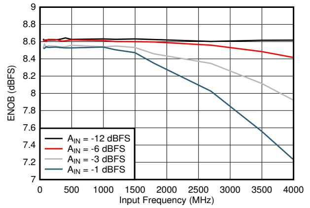
7-18. ENOB vs Input Frequency
