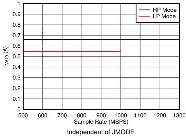
7-85. Quad Channel, I_{VA19} vs FS
