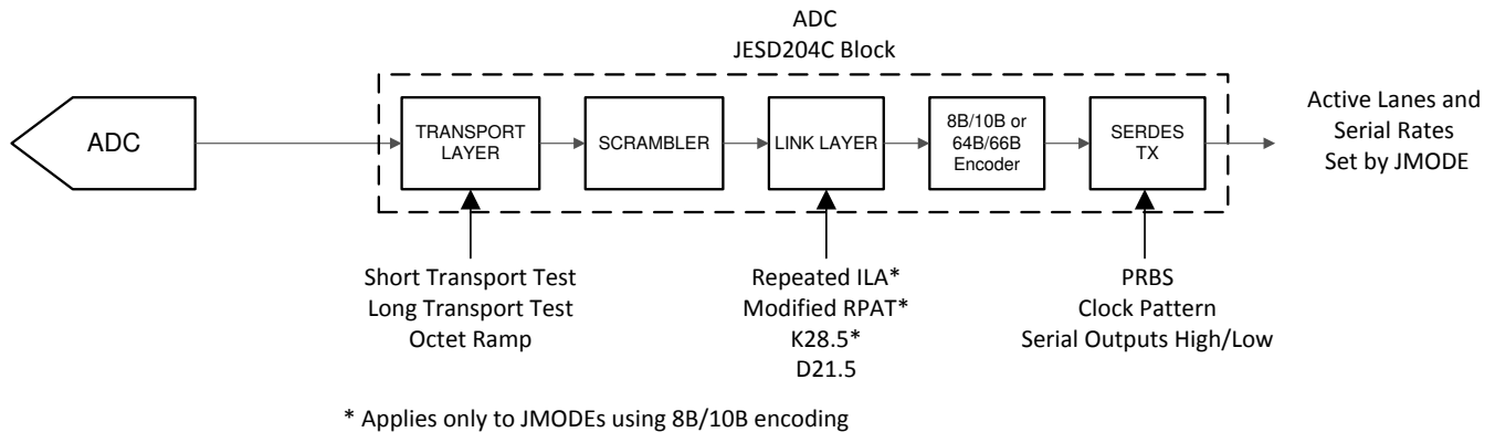
8-14. Test Mode Insertion Points
