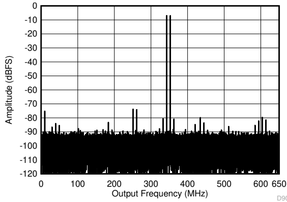
7-49. Two Tone FFT at 348 MHz Center
