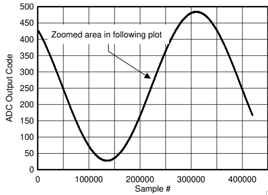
7-127. Background Calibration Core Transition (AC Signal)
