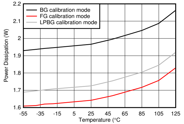
7-124. Dual Channel, Power Dissipation vs Temperature
