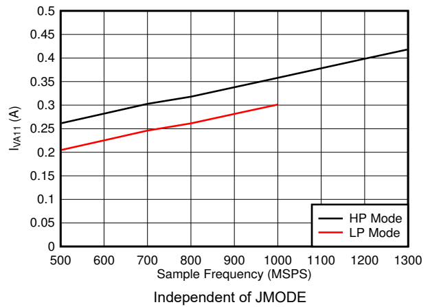
7-106. Single Channel, I_{VA11} vs FS
