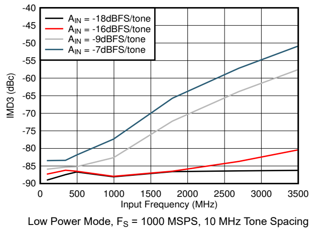
7-58. IMD3 vs Input Frequency
