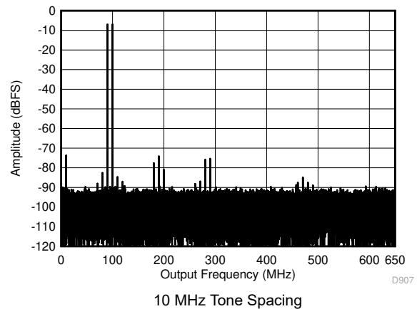
7-48. Two Tone FFT at 95.07 MHz Center
