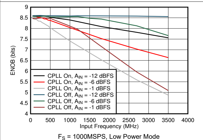
7-78. ENOB vs Input Frequency, CPLL and Input Amplitude
