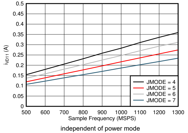
7-98. Dual Channel, I_{VD11} vs FS and JMODE 4 - 7
