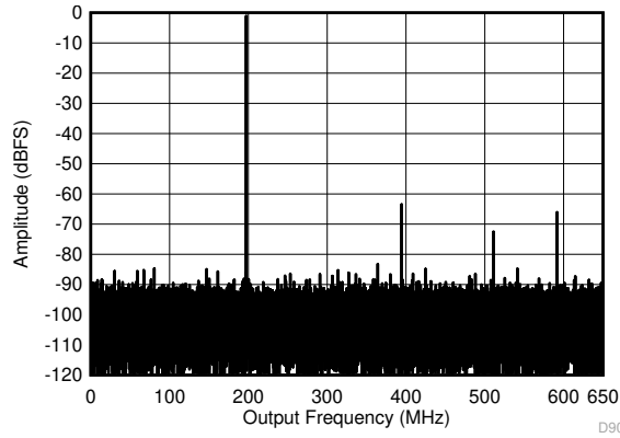
7-7. Single Tone FFT at 1497 MHz and -1 dBFS
