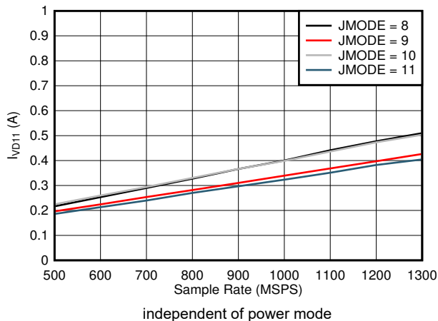
7-89. Quad Channel, I_{VD11} vs FS and JMODE 8 - 11
