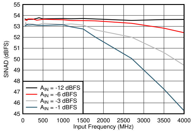
7-17. SINAD vs Input Frequency
