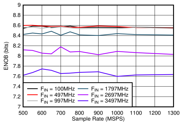
7-24. ENOB vs Sample Rate
