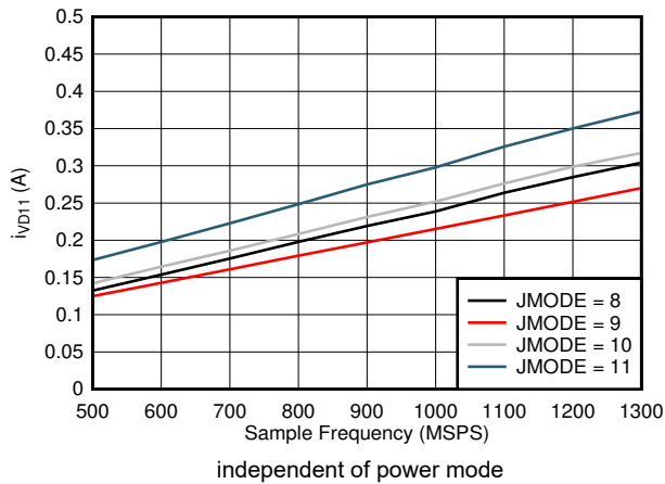
7-99. Dual Channel, I_{VD11} vs FS and JMODE 8 - 11
