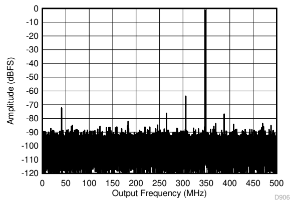
7-10. Single Tone FFT at 3497 MHz and -1 dBFS
