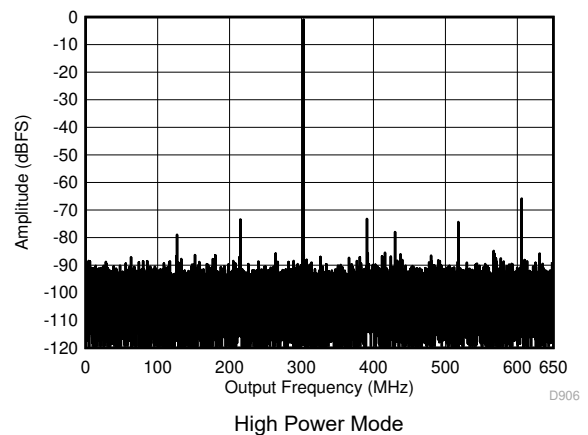
7-6. Single Tone FFT at 997 MHz and -1 dBFS
