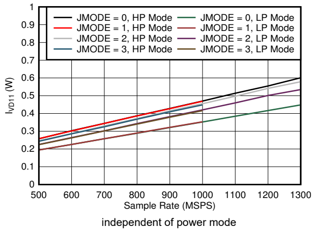
7-87. Quad Channel, I_{VD11} vs FS and JMODE 0 - 3
