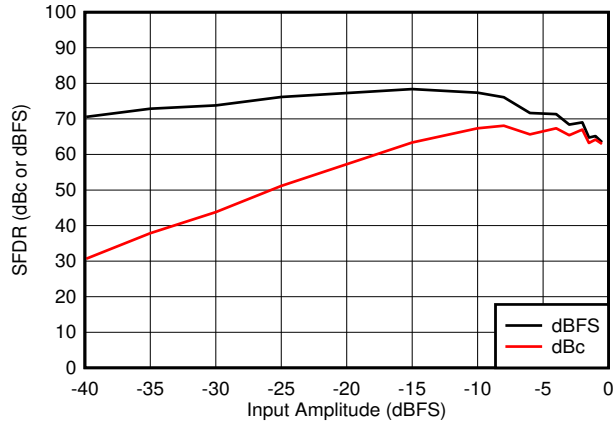
7-31. SFDR vs Input Amplitude
