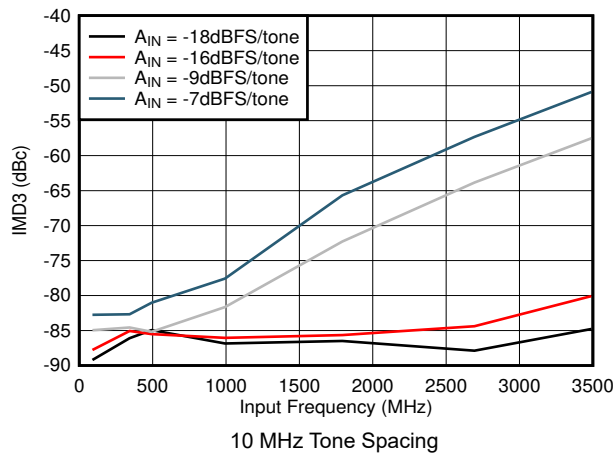
7-57. IMD3 vs Input Frequency
