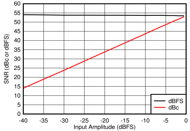
7-32. SNR vs Input Amplitude
