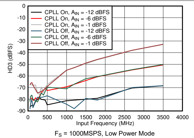
7-80. HD3 vs Input Frequency, CPLL and Input Amplitude
