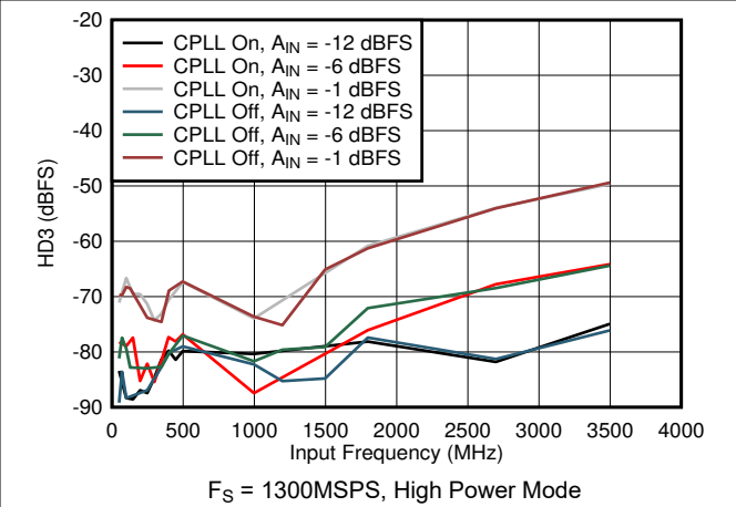
7-74. HD3 vs Input Frequency, CPLL and Input Amplitude
