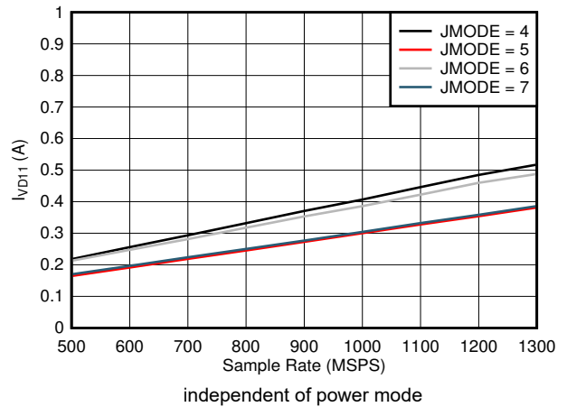
7-88. Quad Channel, I_{VD11} vs FS and JMODE 4 - 7
