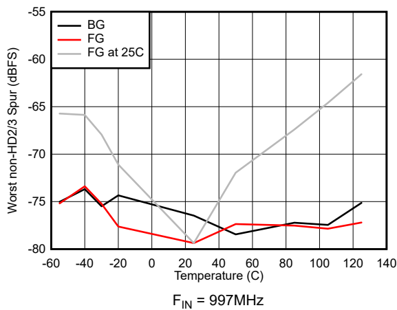
7-39. Worst non-HD2/3 Spur vs Temperature
