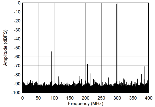
7-8. Single Tone FFT at 2697 MHz and -1dBFS
