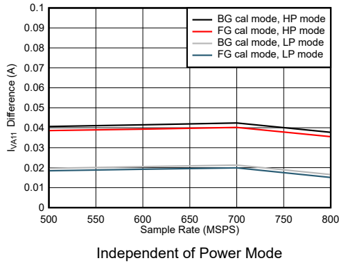
7-109. Single Channel, I_{VA11} Change with Calibration Mode
