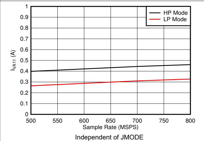
7-76. Quad Channel, I_{VA11} vs F_S
