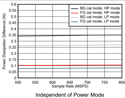
7-101. Quad Channel, Power Dissipation Change with Calibration Mode
