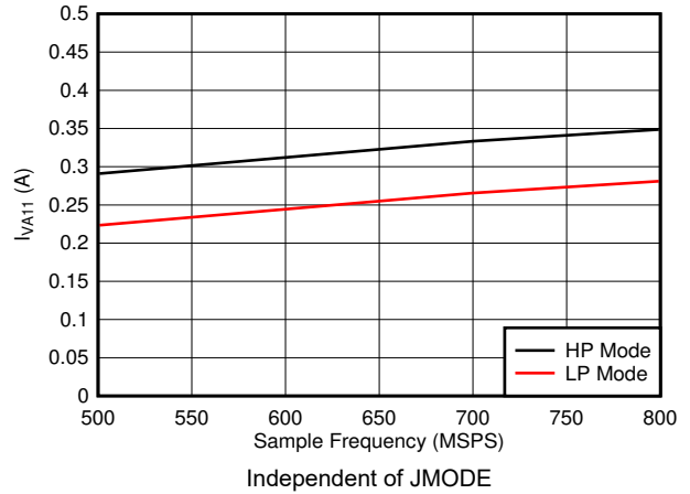
7-86. Dual Channel, I_{VA11} vs F_S
