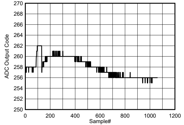
7-116. Background Core Transition (DC midscale input)
