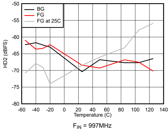
7-37. HD2 vs Temperature
