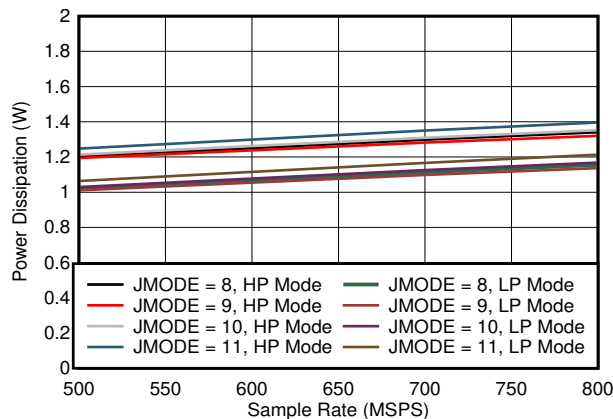
7-83. Dual Channel, Power Dissipation vs F_S for JMODES 8 - 11
