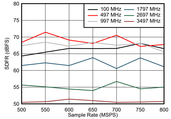
7-20. SFDR vs Sample Rate
