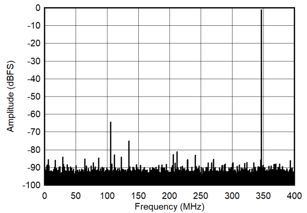
7-4. Single Tone FFT at 347 MHz and -1dBFS
