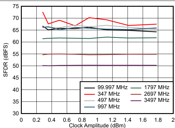
7-33. SFDR vs Clock Amplitude
