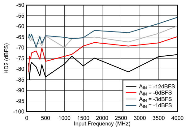
7-18. HD2 vs Input Frequency
