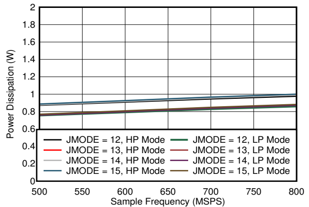
Fig 7-94. Single Channel, Power Dissipation vs F_S for JMODES 12 - 15
