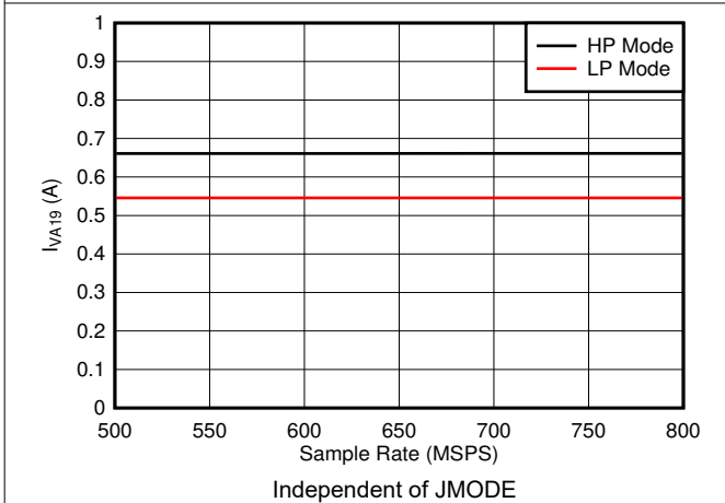
7-75. Quad Channel, I_{VA19} vs F_S
