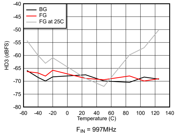
7-38. HD3 vs Temperature
