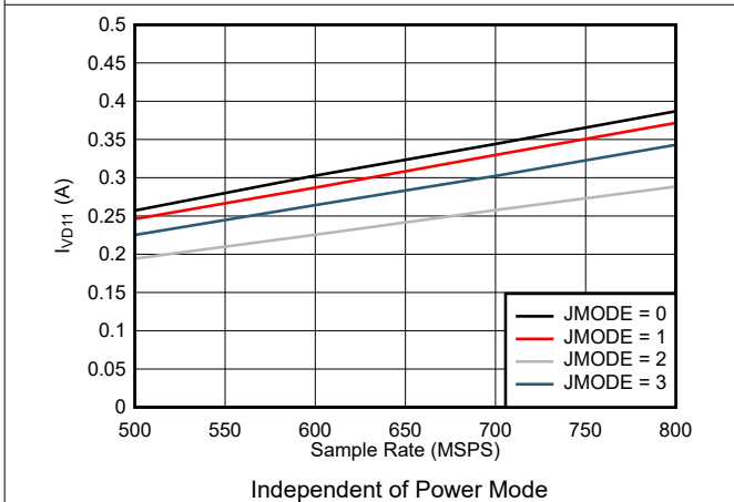
7-77. Quad Channel, I_{VD11} vs F_S for JMODES 0 - 3
