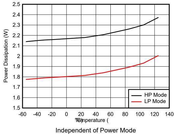
7-113. Quad Channel, Power Dissipation vs Temperature
