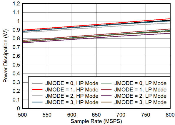
Fig 7-91. Single Channel, Power Dissipation vs F_S for JMODES 0 - 3
