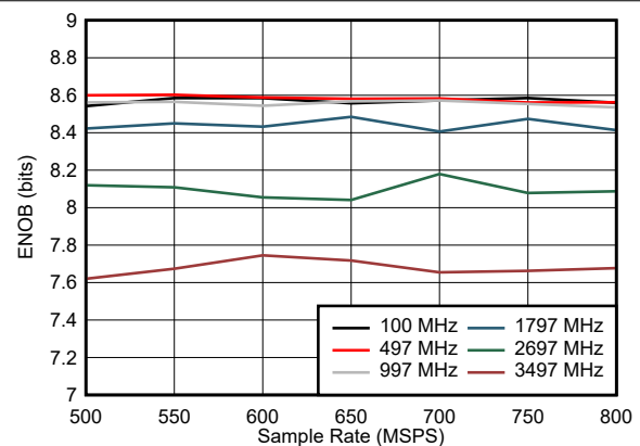
7-23. ENOB vs Sample Rate
