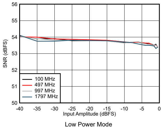
7-31. SNR vs Input Amplitude
