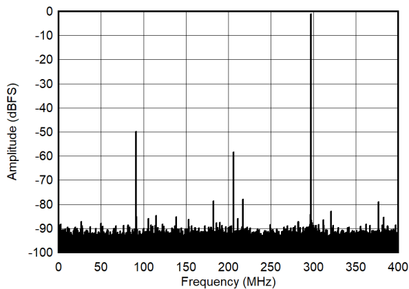
7-9. Single Tone FFT at 3497 MHz and -1dBFS
