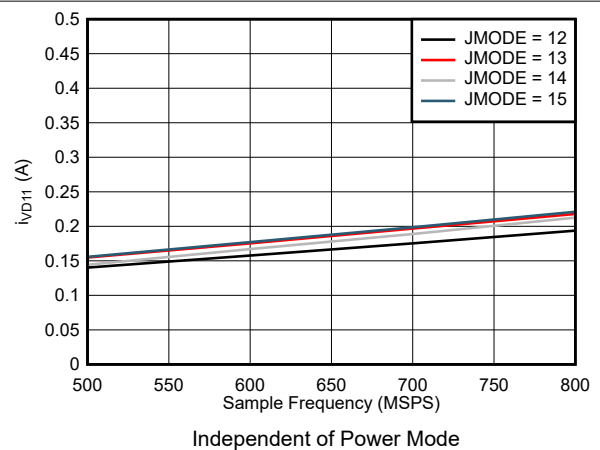
7-90. Dual Channel, I_{VD11} vs F_S for JMODES 12 - 15
