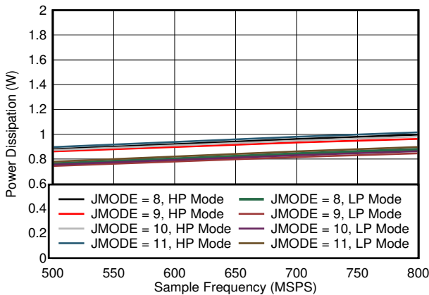
Fig 7-93. Single Channel, Power Dissipation vs F_S for JMODES 8 - 11
