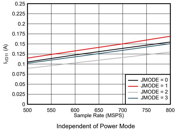
7-97. Single Channel, I_{VD11} vs F_S for JMODES 0 - 3
