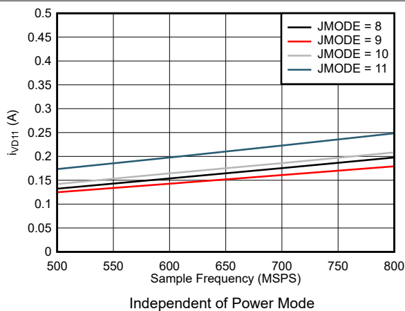
7-89. Dual Channel, I_{VD11} vs F_S for JMODES 8 - 11
