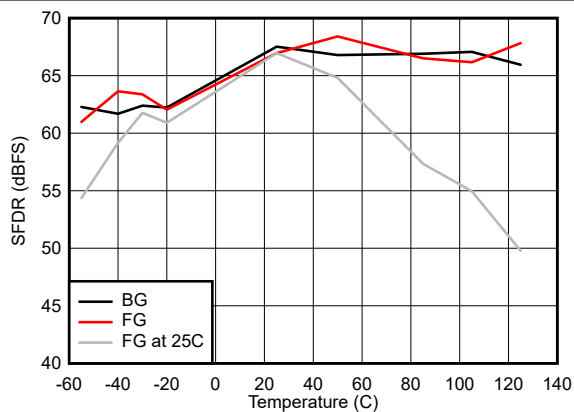
7-35. SFDR vs Temperature
