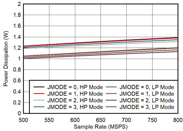
7-81. Dual Channel, Power Dissipation vs F_S for JMODES 0 - 3
