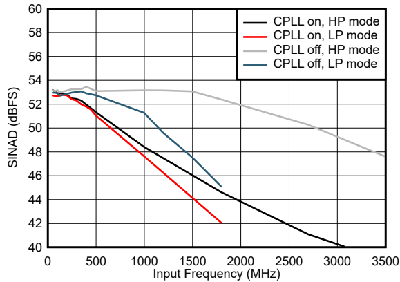
7-67. SINAD vs Input Frequency and CPLL and Power Mode
