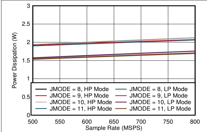
7-73. Quad Channel, Power Dissipation vs F_S for JMODES 8 - 11
