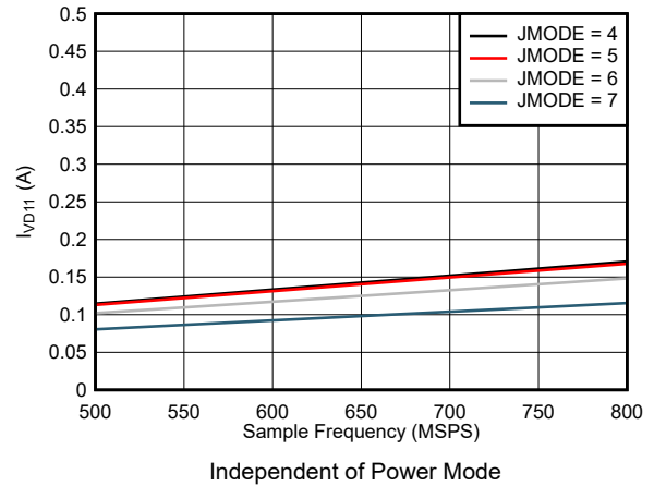
7-98. Single Channel, I_{VD11} vs F_S for JMODES 4 - 7
