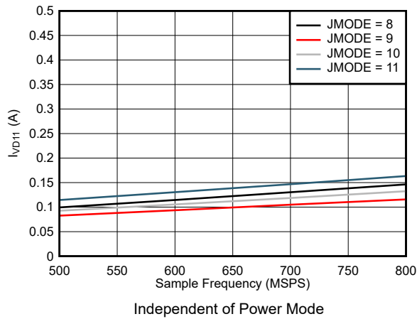
7-99. Single Channel, I_{VD11} vs F_S for JMODES 8 - 11
