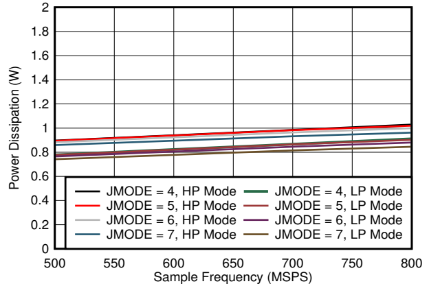
Fig 7-92. Single Channel, Power Dissipation vs F_S for JMODES 4 - 7
