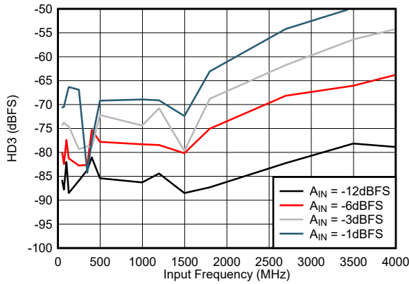
7-19. HD3 vs Input Frequency
