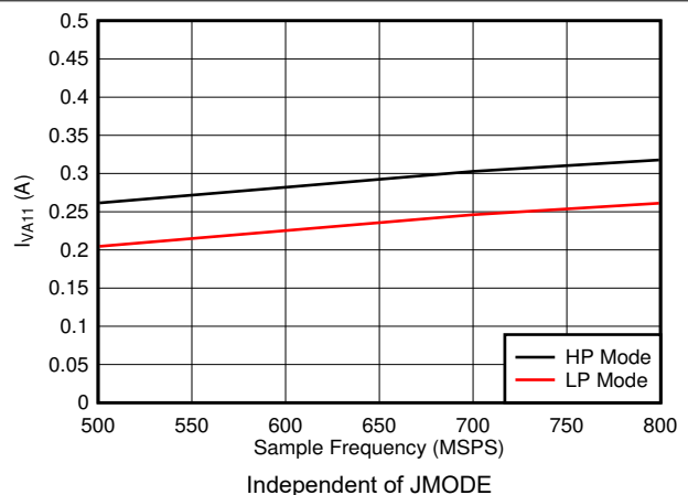
Fig 7-96. Single Channel, I_{VA11} vs F_S
