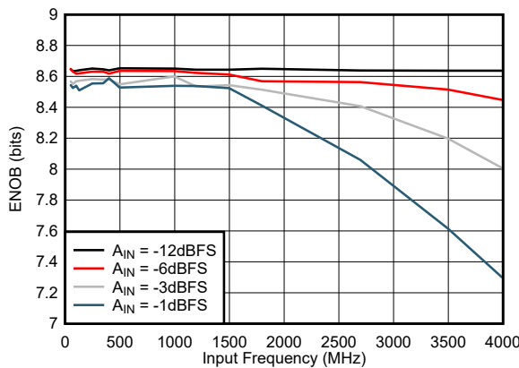
7-17. ENOB vs Input Frequency
