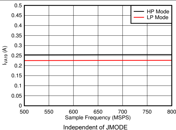
Fig 7-95. Single Channel, I_{VA19} vs F_S
