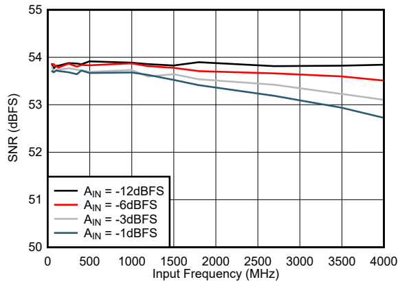
7-15. SNR vs Input Frequency
