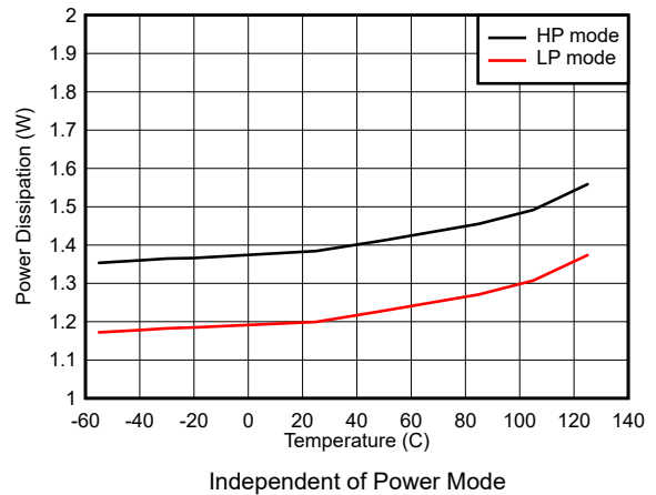
7-114. Dual Channel, Power Dissipation vs Temperature
