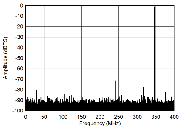
7-11. Single Tone FFT at 347MHz and -1dBFS
