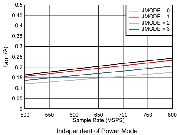
7-87. Dual Channel, I_{VD11} vs F_S for JMODES 0 - 3
