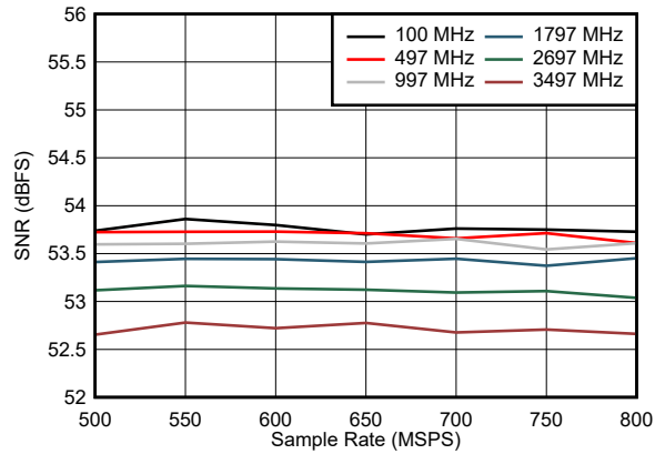
7-21. SNR vs Sample Rate
