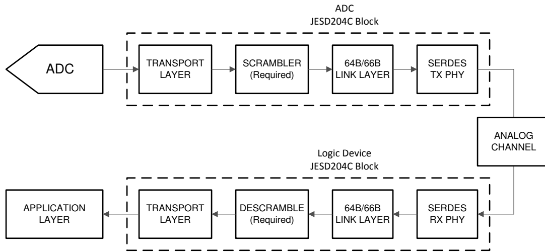
图 8-8. Simplified 64B/66B Encoded JESD204C Interface Diagram
