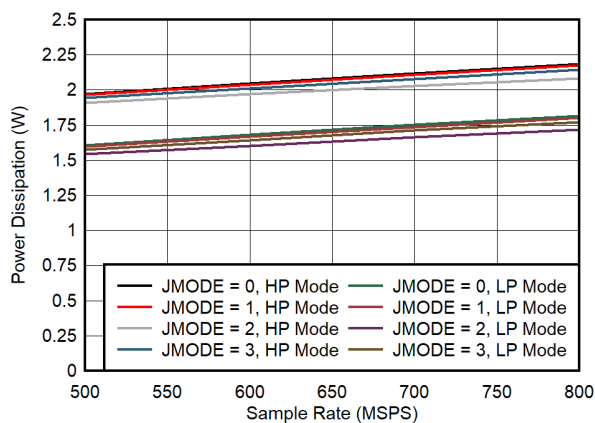
7-71. Quad Channel, Power Dissipation vs F_S for JMODES 0 - 3
