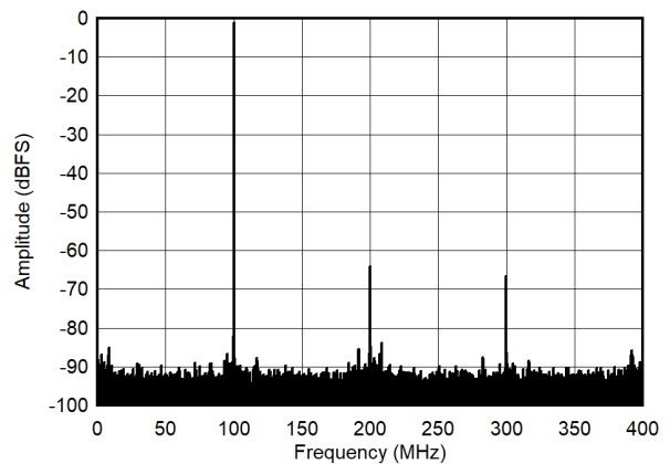
7-10. Single Tone FFT at 100MHz and -1dBFS
