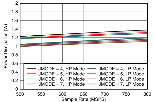
7-82. Dual Channel, Power Dissipation vs F_S for JMODES 4 - 7
