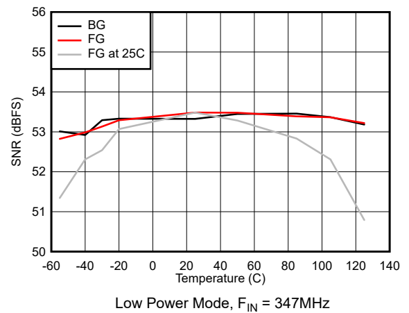
7-40. SNR vs Temperature
