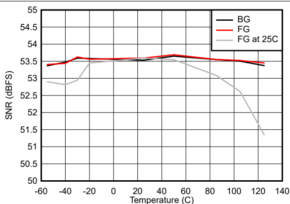
7-34. SNR vs Temperature
