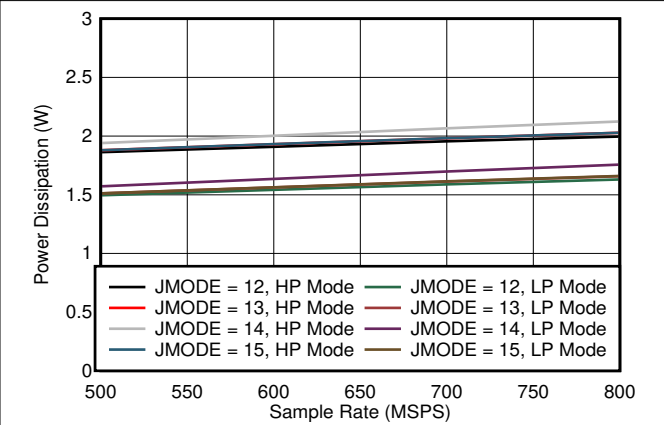
7-74. Quad Channel, Power Dissipation vs F_S for JMODES 12 - 15
