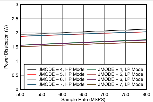
7-72. Quad Channel, Power Dissipation vs F_S for JMODES 4 - 7
