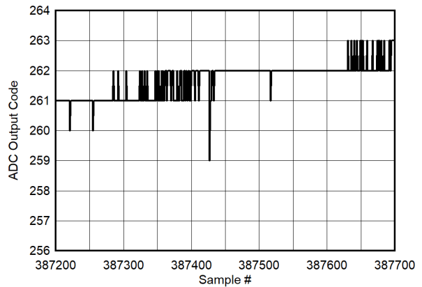
7-118. Background Core Transition (AC Signal Zoomed)
