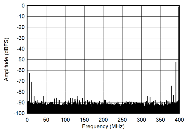
7-12. Single Tone FFT at 1197MHz and -1dBFS
