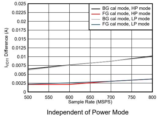
7-112. Single Channel, I_{VD11} Change with Calibration Mode
