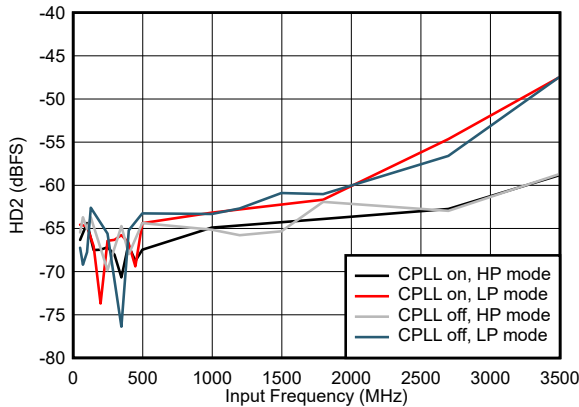
7-69. HD2 vs Input Frequency and CPLL and Power Mode
