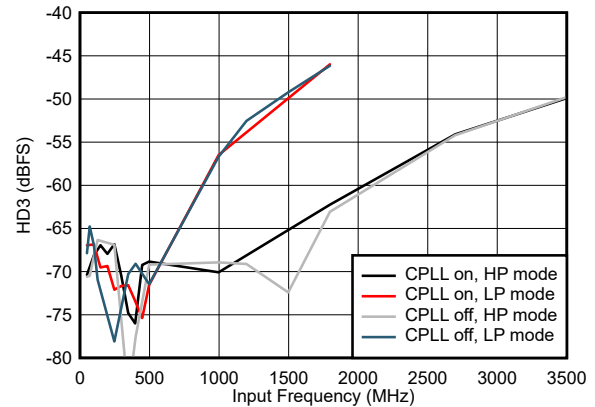
7-70. HD3 vs Input Frequency and CPLL and Power Mode
