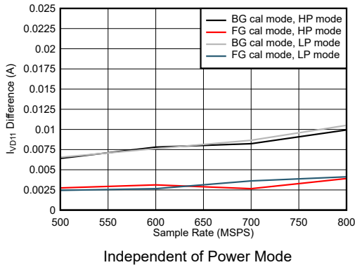
7-111. Dual Channel, I_{VD11} Change with Calibration Mode
