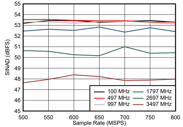
7-22. SINAD vs Sample Rate
