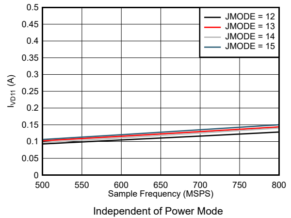
7-100. Single Channel, I_{VD11} vs F_S for JMODES 12 - 15
