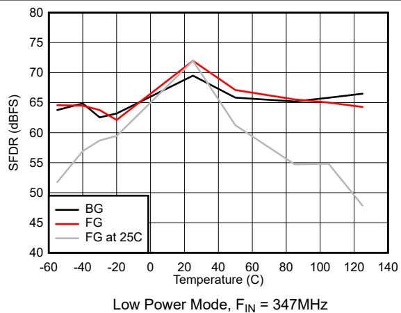
7-41. SFDR vs Temperature
