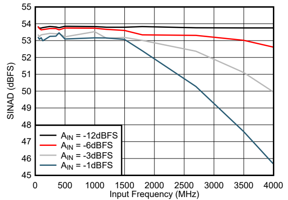
7-16. SINAD vs Input Frequency
