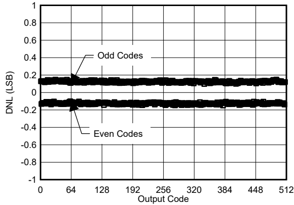
7-1. DNL vs Code
