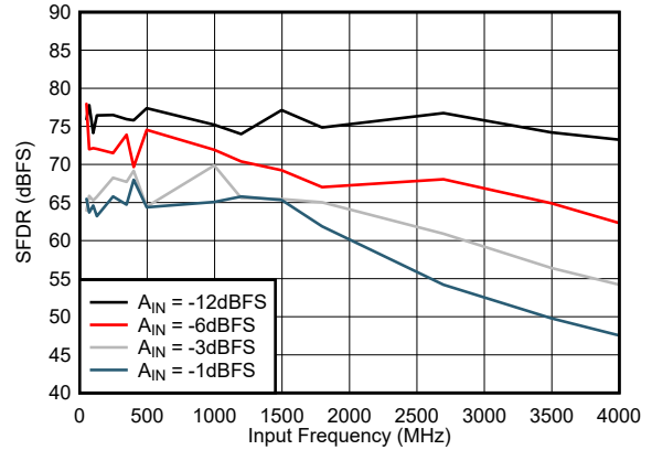
7-14. SFDR vs Input Frequency
