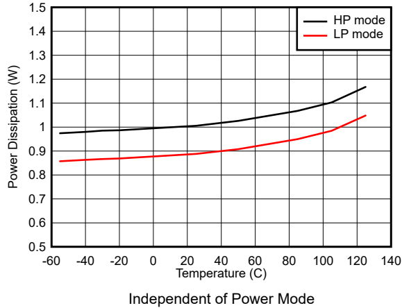
7-115. Single Channel, Power Dissipation vs Temperature
