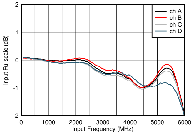
7-3. Input Fullscale vs Input Frequency
