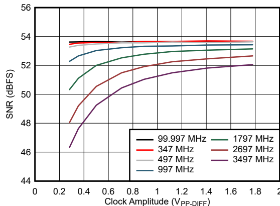
7-32. SNR vs Clock Amplitude
