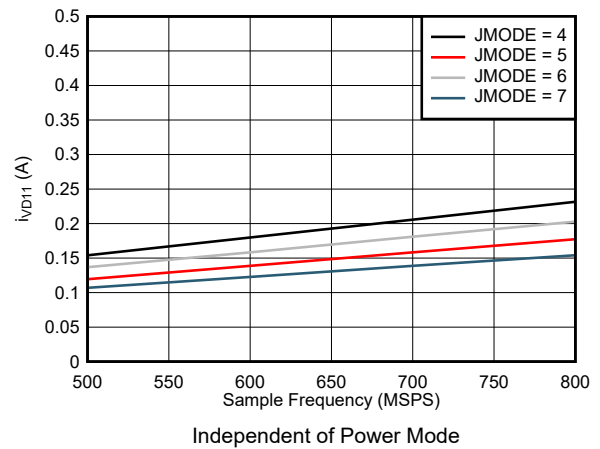
7-88. Dual Channel, I_{VD11} vs F_S for JMODES 4 - 7
