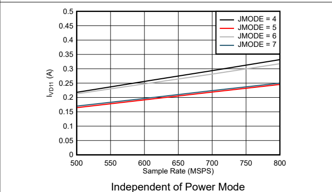
7-78. Quad Channel, I_{VD11} vs F_S for JMODES 4 - 7
