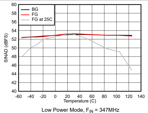
7-42. SINAD vs Temperature
