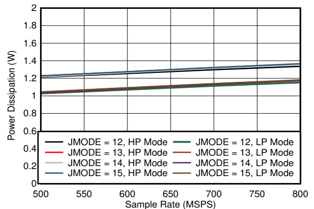
7-84. Dual Channel, Power Dissipation vs F_S for JMODES 12 - 15
