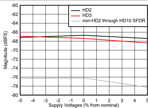
F_{IN} = 347 MHz
