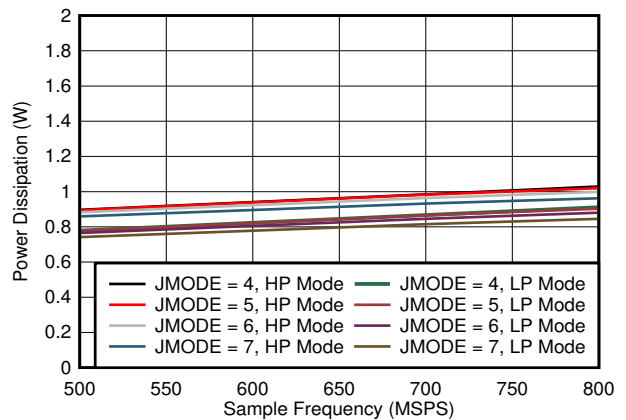
5-92. Single Channel, Power Dissipation vs F_S for JMODES 4 - 7
