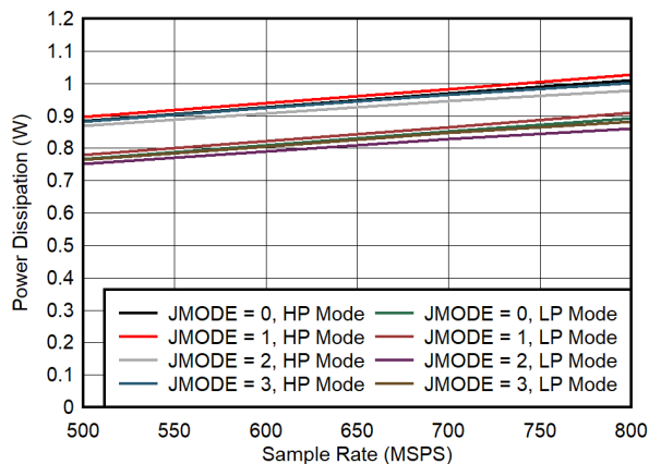
5-91. Single Channel, Power Dissipation vs F_S for JMODES 0 - 3
