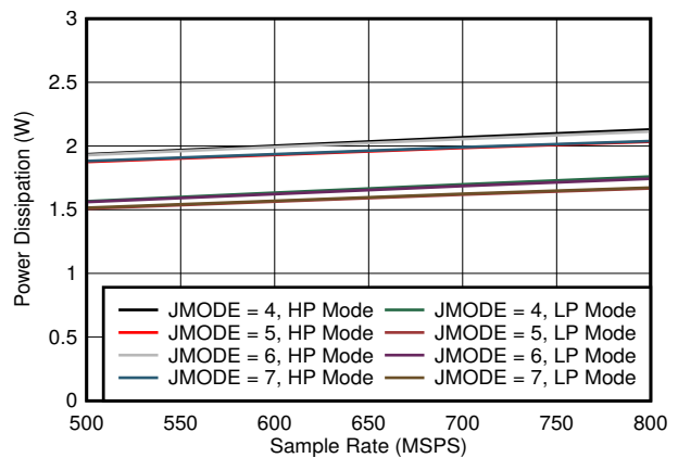
5-72. Quad Channel, Power Dissipation vs F_S for JMODES 4 - 7
