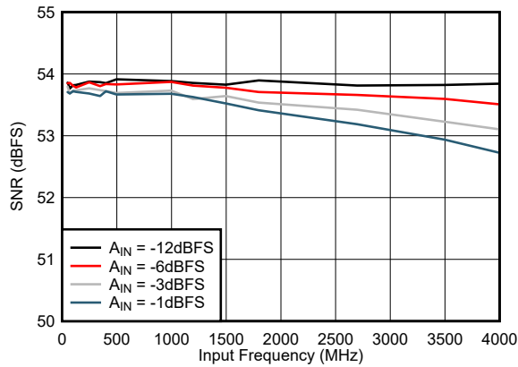
5-15. SNR vs Input Frequency
