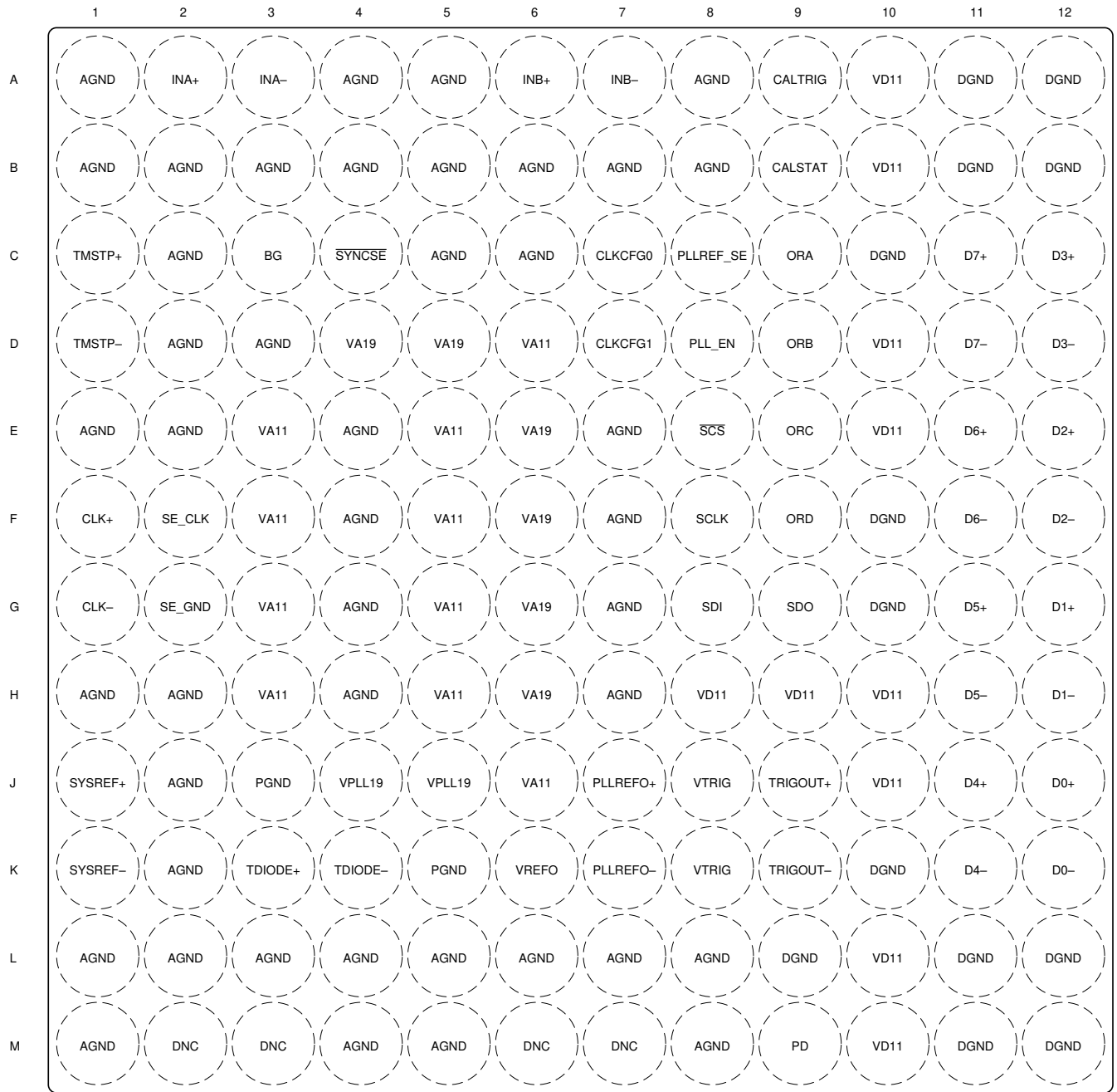
4-2. Dual Channel AAV Package, 144-Ball Flip Chip BGA (Top View)
