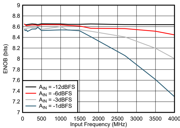
5-17. ENOB vs Input Frequency
