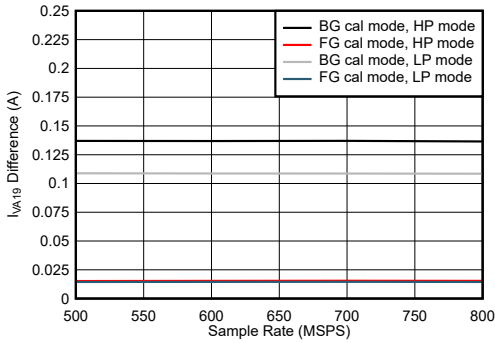
5-105. Dual Channel, I_{VA19} Change with Calibration Mode
