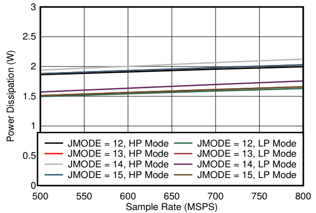
5-74. Quad Channel, Power Dissipation vs F_S for JMODES 12 - 15
