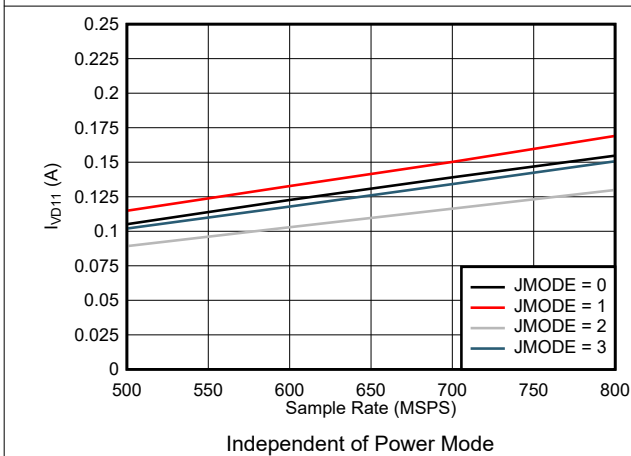
图 5-97. Single Channel, I_{VD11} vs F_S for JMODES 0 - 3
