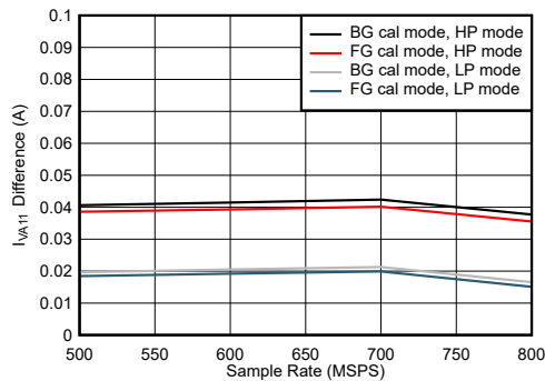
5-107. Quad Channel, I_{VA11} Change with Calibration Mode
