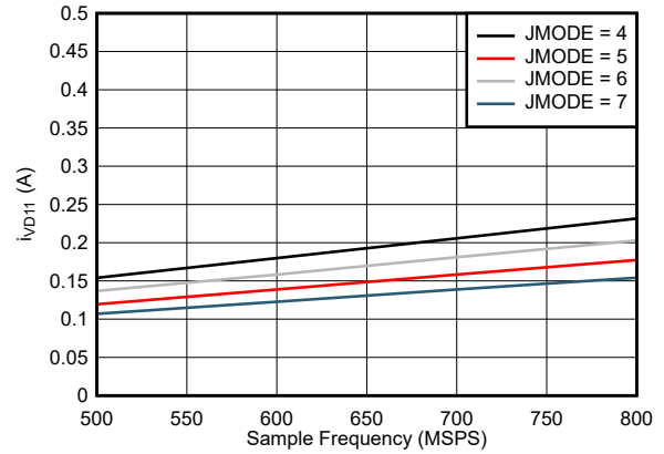
5-88. Dual Channel, I_{VD11} vs F_S for JMODES 4 - 7
