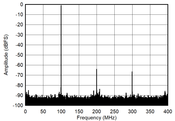
图 5-10. Single Tone FFT at 100MHz and -1dBFS Low Power Mode
