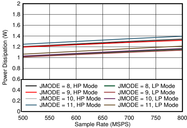
5-83. Dual Channel, Power Dissipation vs F_S for JMODES 8 - 11
