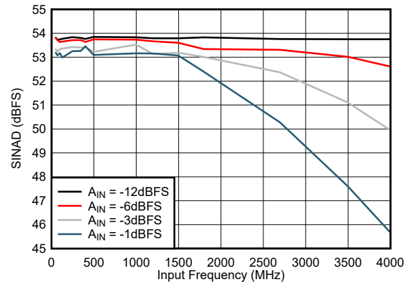
5-16. SINAD vs Input Frequency
