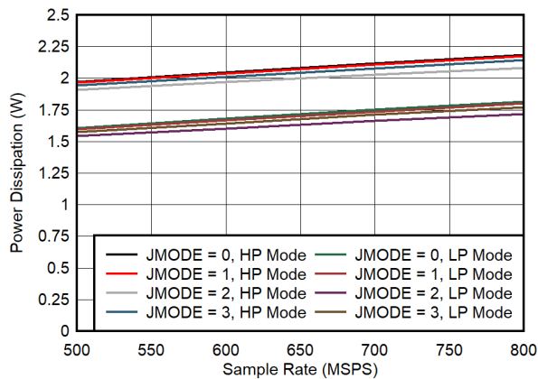
5-71. Quad Channel, Power Dissipation vs F_S for JMODES 0 - 3
