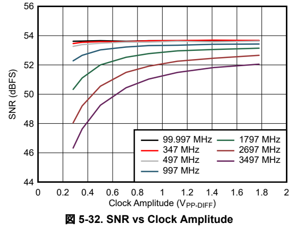
Figure 5-32. SNR vs Clock Amplitude
