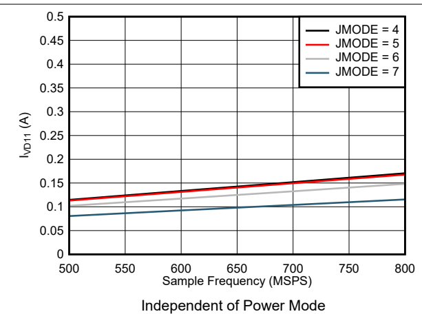
图 5-98. Single Channel, I_{VD11} vs F_S for JMODES 4 - 7
