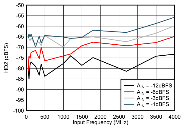
5-18. HD2 vs Input Frequency
