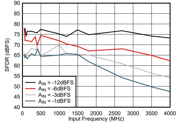
5-14. SFDR vs Input Frequency
