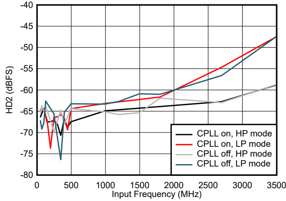
5-69. HD2 vs Input Frequency and CPLL and Power Mode
