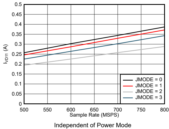
5-77. Quad Channel, I_{VD11} vs F_S for JMODES 0 - 3
