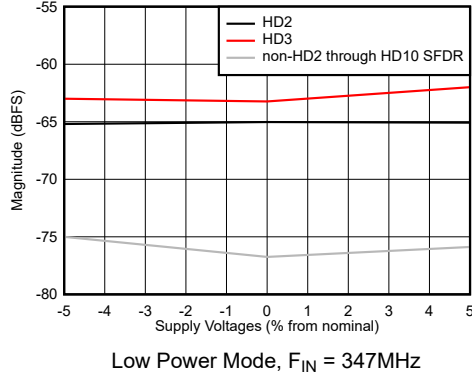
图 5-49. HD2, HD3 and Worst non-HD2/3 Spur vs Supply Voltage
