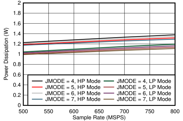
5-82. Dual Channel, Power Dissipation vs F_S for JMODES 4 - 7
