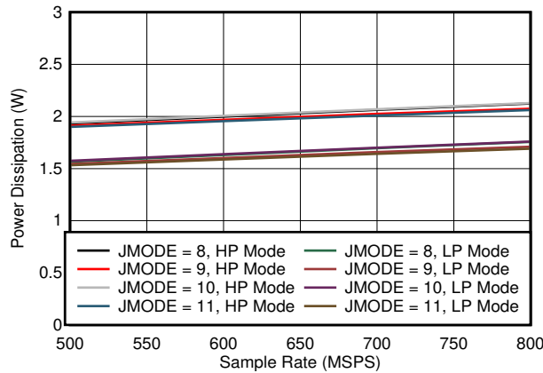
5-73. Quad Channel, Power Dissipation vs F_S for JMODES 8 - 11
