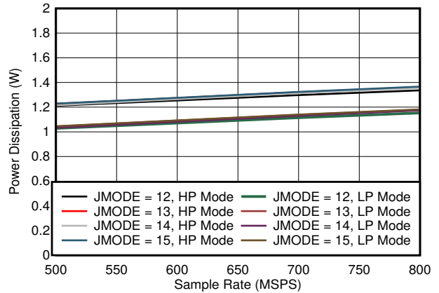
5-84. Dual Channel, Power Dissipation vs F_S for JMODES 12 - 15
