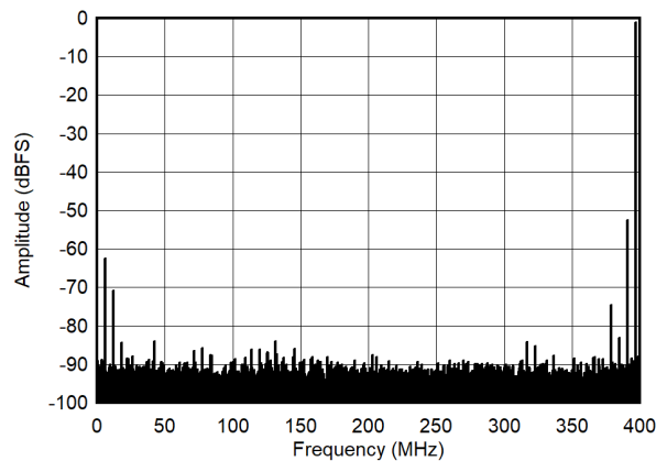
图 5-12. Single Tone FFT at 1197MHz and -1dBFS Low Power Mode
