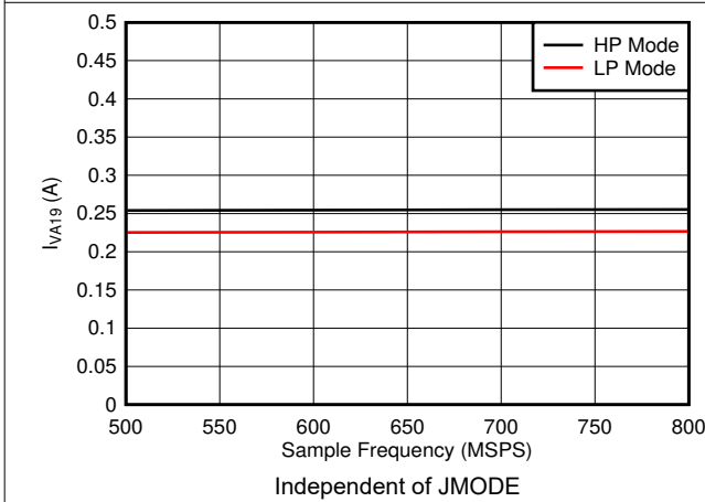
图 5-95. Single Channel, I_{VA19} vs F_S
