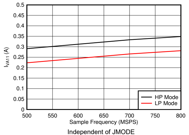
5-86. Dual Channel, I_{VA11} vs F_S
