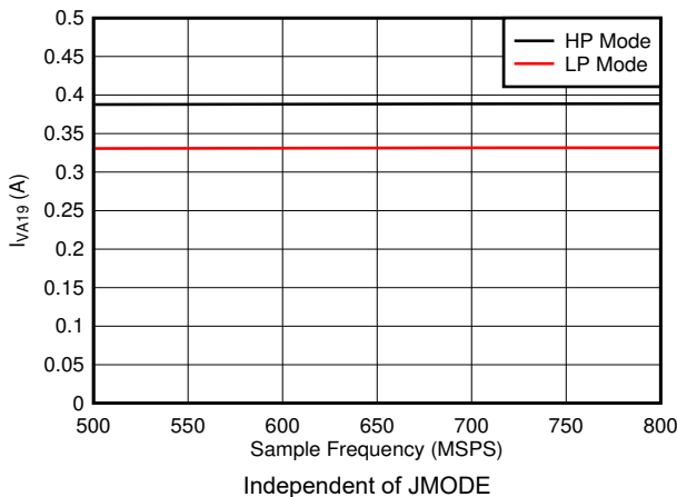
5-85. Dual Channel, I_{VA19} vs F_S
