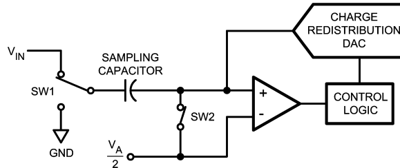
FIGURE 3. ADC101S051 in Track Mode
