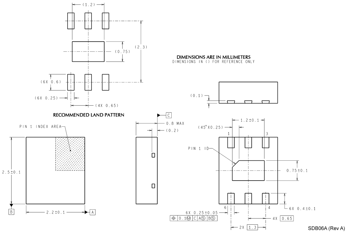
6-Lead LLP Order Number ADC101S051CISD or ADC101S051CISDX NS Package Number SDB06A 単位は millimeters
