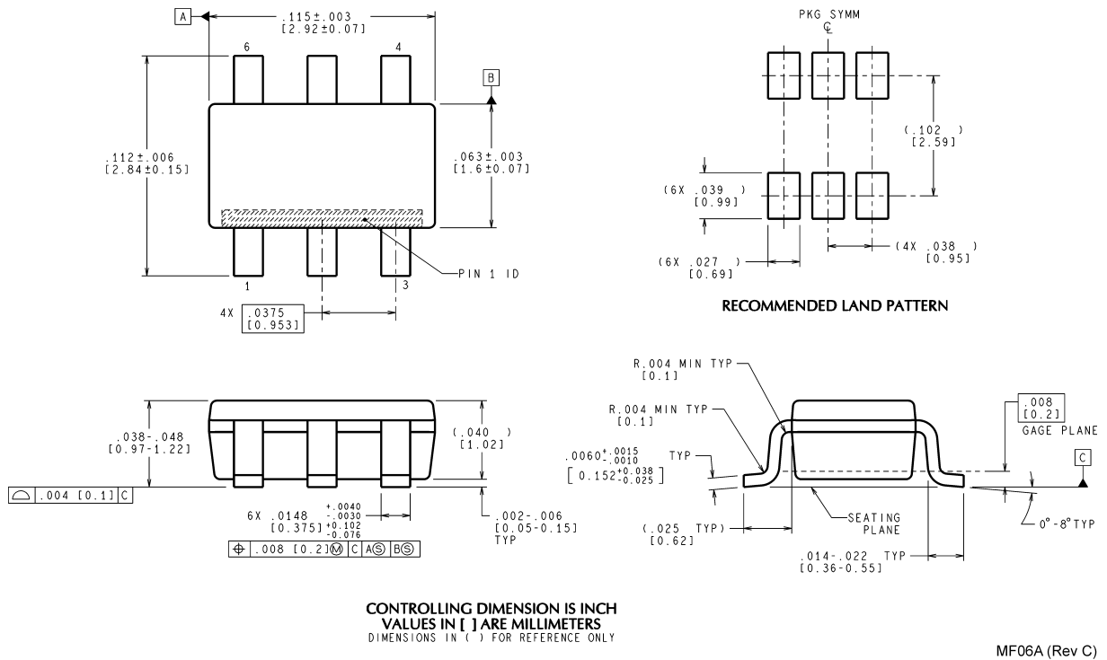
6-Lead SOT-23 Order Number ADC101S051CIMF, ADC101S051CIMFX NS Package Number MF06A
