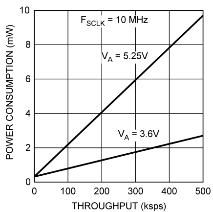
Power Consumption vs. Throughput, f_{\text{SCLK}} = 10\text{ MHz}
