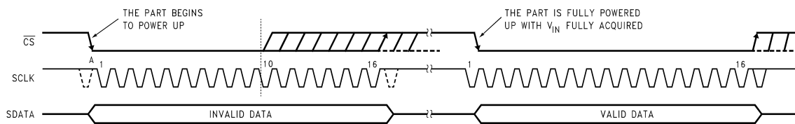
FIGURE 9. Entering Normal Mode
