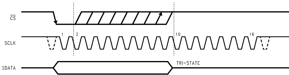
FIGURE 8. Entering Shutdown Mode
