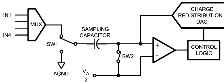
FIGURE 1. ADC104S021 in Track Mode
