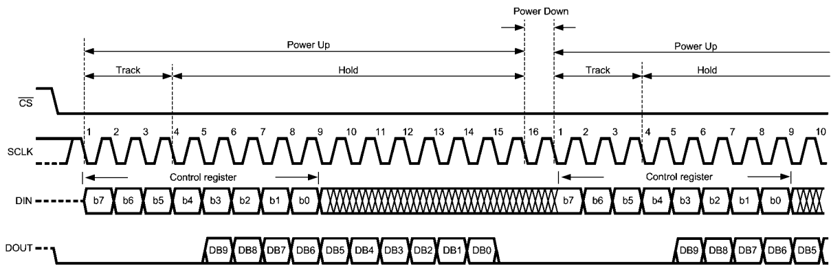
ADC104S021 Operational Timing Diagram
