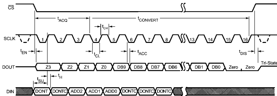
ADC104S021 Serial Timing Diagram
