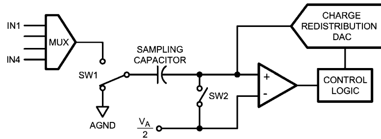
FIGURE 2. ADC104S021 in Hold Mode
