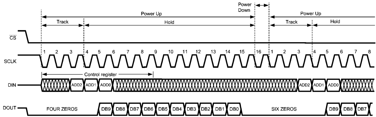
FIGURE 1. ADC108S102 Operational Timing Diagram
