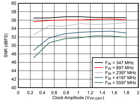
6-88. DES Mode: SNR vs Clock Amplitude
