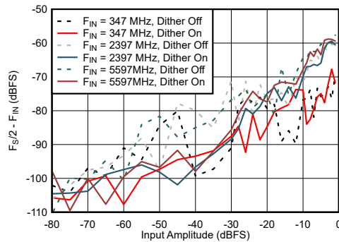
6-64. DES Mode: F_{S/2} - F_{IN} vs Input Amplitude and Dither
