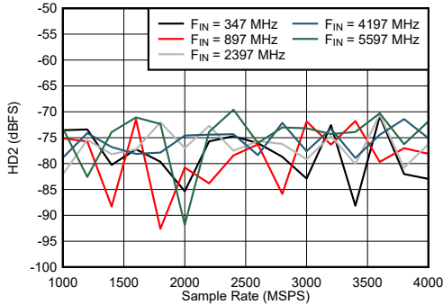
6-49. Dual Channel Mode: HD2 vs Sample Rate and Input Frequency
