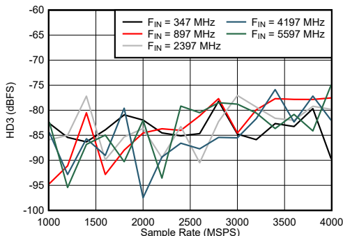
6-51. Dual Channel Mode: HD3 vs Sample Rate and Input Frequency
