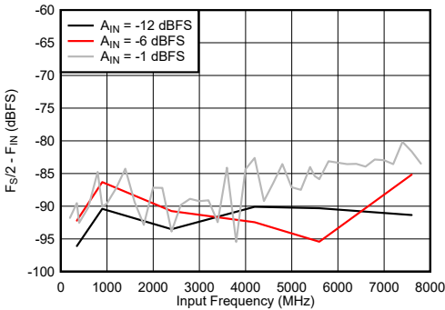
6-87. Dual Channel Mode: F_S/2 - F_{IN} vs Input Frequency
