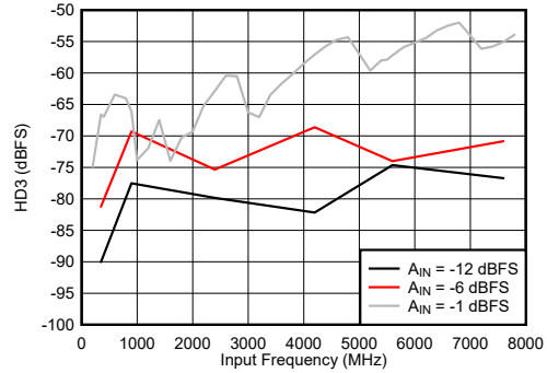
6-86. Dual Channel Mode: HD3 vs Input Frequency
