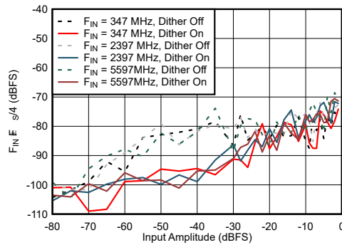
6-66. DES Mode: F_{IN} \pm F_{S/4} vs Input Amplitude and Dither
