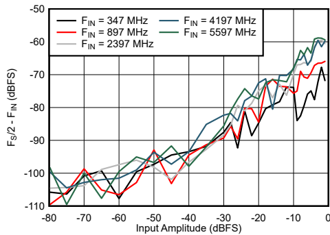
6-63. DES Mode: F_{S/2} - F_{IN} vs Input Amplitude and Frequency
