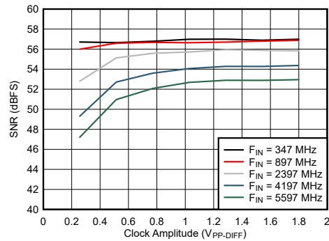
6-90. Dual Channel Mode: SNR vs Clock Amplitude
