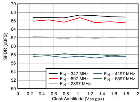
6-89. DES Mode: SFDR vs Clock Amplitude
