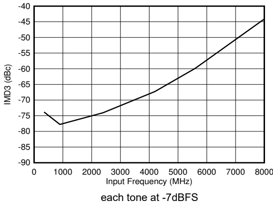
5-99. DES Mode: IMD3 vs Input Frequency
