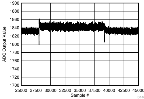
5-145. Background Calibration Core Transition (DC Signal - zoomed)
