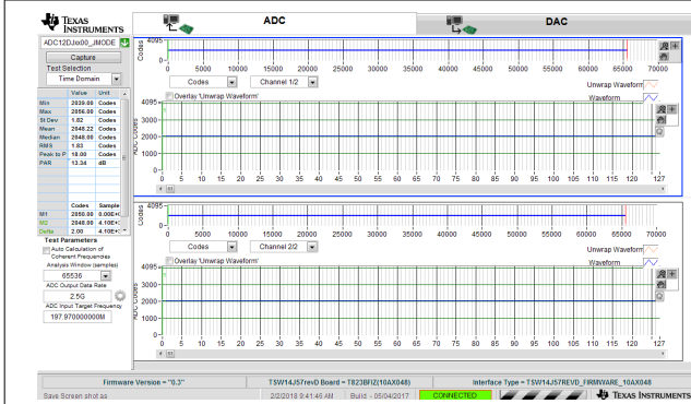
図 7-10. Idle-Channel Noise (No Input) for 2.5-GSPS, Dual-Channel Oscilloscope
