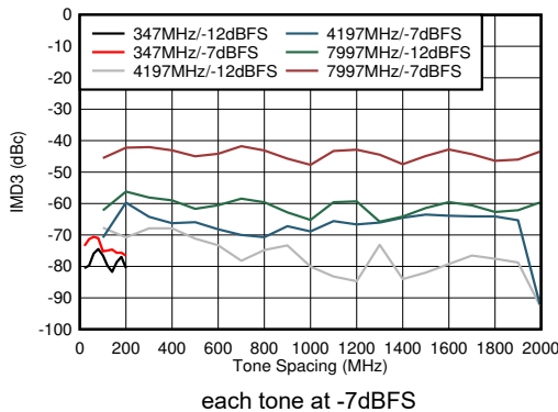
5-101. DES Mode: IMD3 vs Tone Spacing
