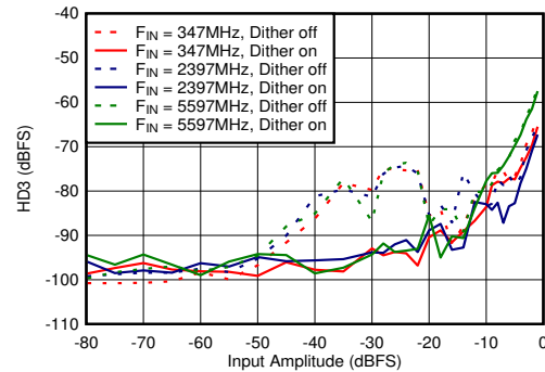
5-64. DES Mode: HD3 vs Input Amplitude and Dither
