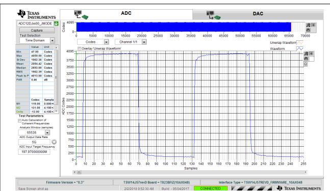
7-7. 40-MHz, Square-Wave Time Domain for 5-GSPS, Single-Channel Oscilloscope
