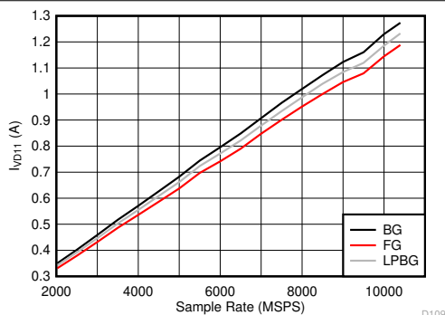
5-123. DES Mode: I_{VD11} vs Sample Rate
