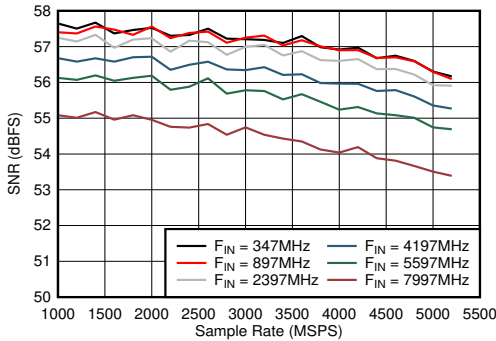
图 5-45. Dual Channel Mode: SNR vs Sample Rate and Input Frequency A_{IN} = -6\text{ dBFS}
