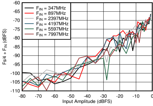
图 5-67. DES Mode: F_s/4 + F_{IN} vs Input Amplitude and Frequency
