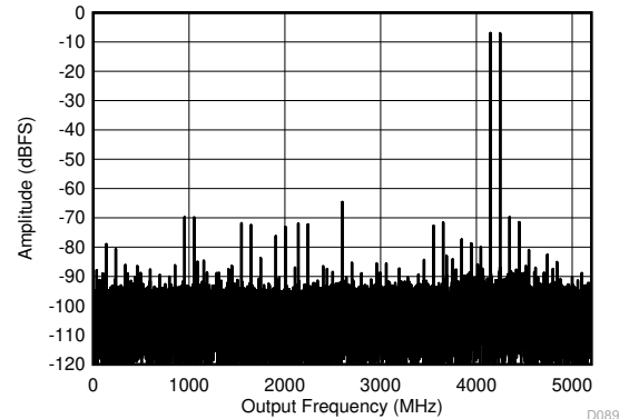
5-14. DES Mode: Two Tone FFT at 4197 MHz
