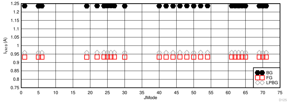
5-109. DES Mode: I_{VA19} vs JMODE at 10.4GSPS
