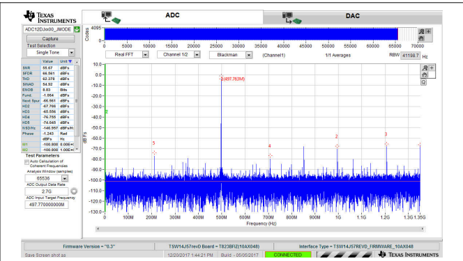
7-3. FFT for 497.77-MHz Input Signal, 2.7 GSPS, JMODE2
