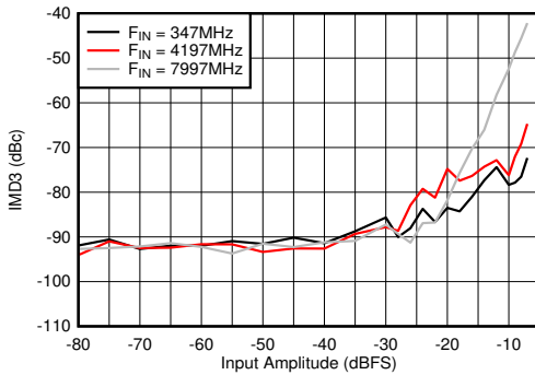
5-105. Dual Channel Mode: IMD3 vs Input Amplitude
