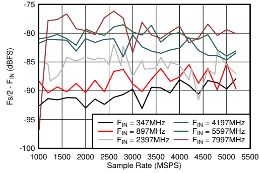
5-56. Dual Channel Mode: F_s/2 - F_{IN} vs Sample Rate and Input Frequency
