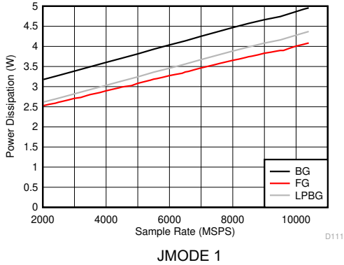
Figure 5-127. DES Mode: Power Dissipation vs Sample Rate
