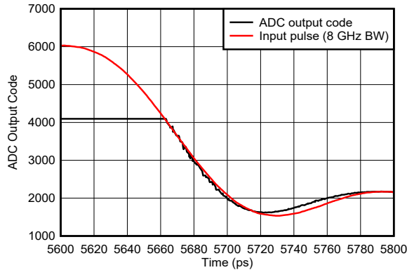
5-147. Pulse Overdrive Recovery Zoomed
