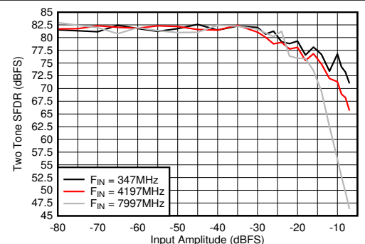
5-108. Dual Channel Mode: Two Tone SFDR vs Input Amplitude
