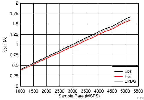
5-134. Dual Channel Mode: I_{VD11} vs Sample Rate
