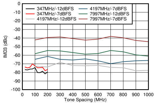
5-106. Dual Channel Mode: IMD3 vs Tone Spacing
