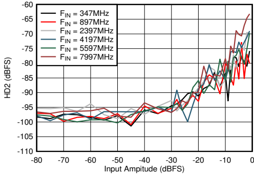
5-61. DES Mode: HD2 vs Input Amplitude and Frequency
