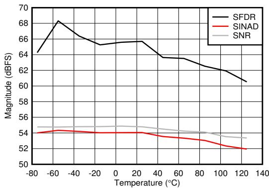
FIG 5-89. Dual Channel Mode: SNR, SINAD and SFDR vs Temperature
