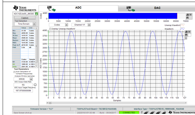
7-8. 200-MHz, Sine-Wave Time Domain for 5-GSPS, Single-Channel Oscilloscope
