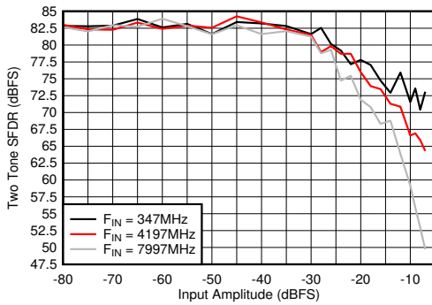
5-103. DES Mode: Two Tone SFDR vs Input Amplitude
