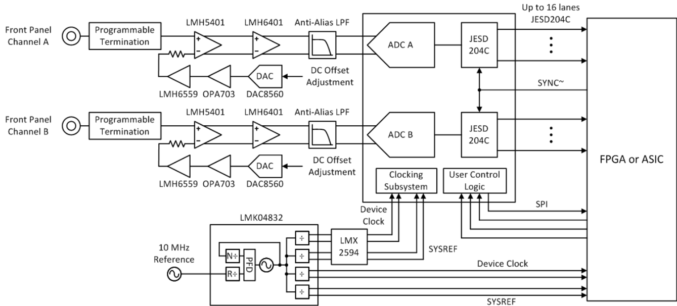
FIG 7-5. Typical Configuration for Reconfigurable Oscilloscope
