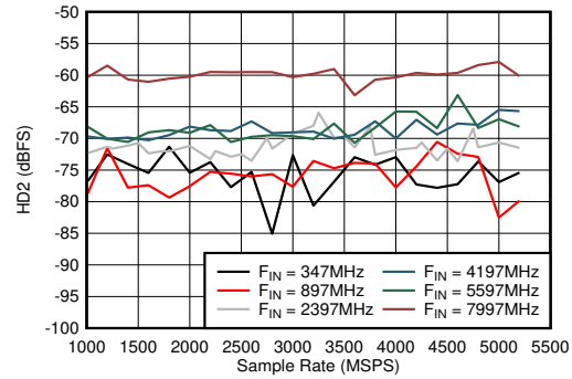
5-50. Dual Channel Mode: HD2 vs Sample Rate and Input Frequency
