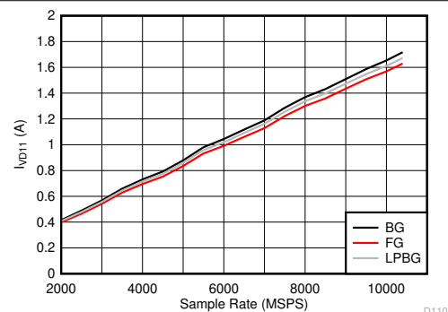
5-126. DES Mode: I_{VD11} vs Sample Rate
