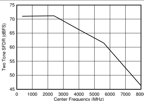
5-107. Dual Channel Mode: Two Tone SFDR vs Input Frequency
