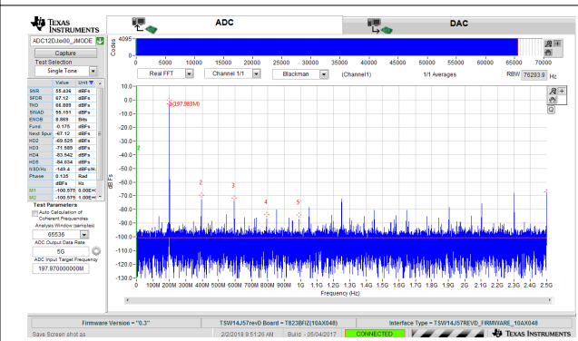
7-9. 200-MHz, Sine-Wave Frequency Domain (FFT) for 5-GSPS, Single-Channel Oscilloscope
