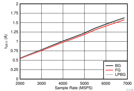
5-122. DES Mode: I_{VA11} vs Sample Rate
