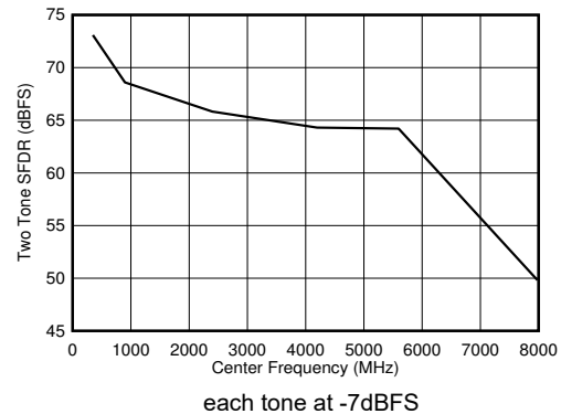
5-102. DES Mode: Two Tone SFDR vs Input Frequency
