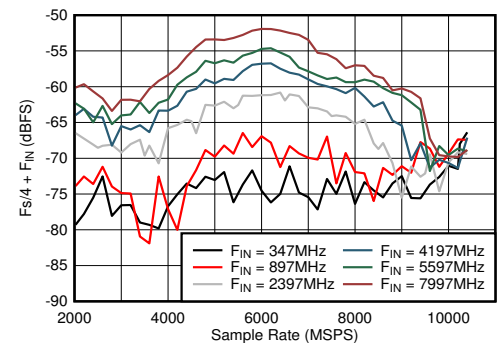
Figure 5-42. DES Mode: F_s/4 + F_{IN} vs Sample Rate and Input Frequency
