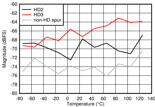
5-87. DES Mode: HD2, HD3 and Worst non-HD Spur vs Temperature
