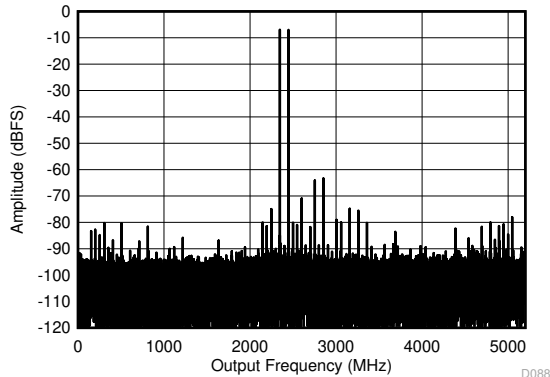
5-13. DES Mode: Two Tone FFT at 2397 MHz
