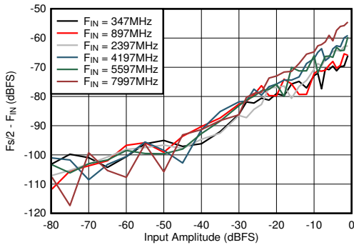
5-65. DES Mode: F_s/2 - F_{\text{IN}} vs Input Amplitude and Frequency
