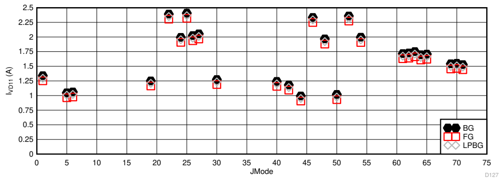
5-110. DES Mode: I_{VA11} vs JMODE at 10.4GSPS
