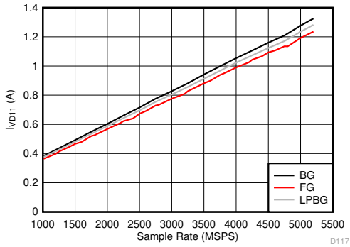
5-133. Dual Channel Mode: I_{VD11} vs Sample Rate
