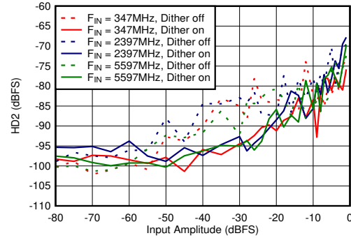
5-62. DES Mode: HD2 vs Input Amplitude and Dither
