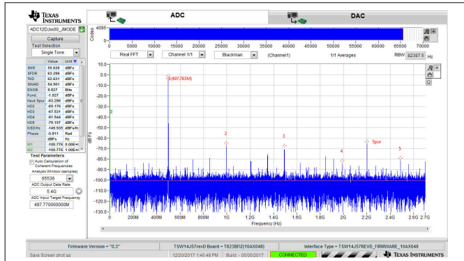
7-2. FFT for 497.77-MHz Input Signal, 5.4 GSPS, JMODE0
