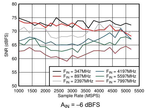
图 5-48. Dual Channel Mode: SFDR vs Sample Rate and Input Frequency A_{IN} = -6\text{ dBFS}
