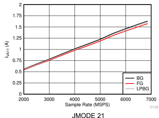
5-124. DES Mode: I_{VD11} vs Sample Rate
