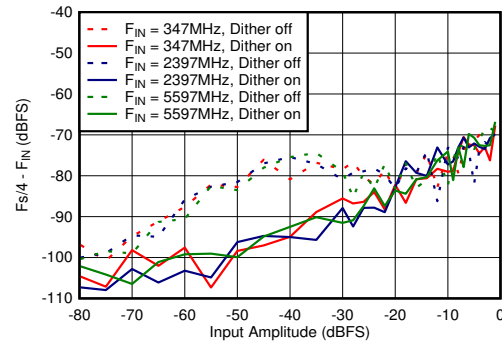
图 5-70. DES Mode: F_s/4 - F_{IN} vs Input Amplitude and Dither
