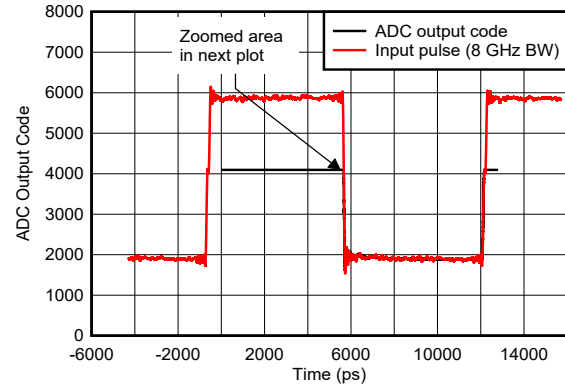
5-146. Pulse Overdrive Recovery
