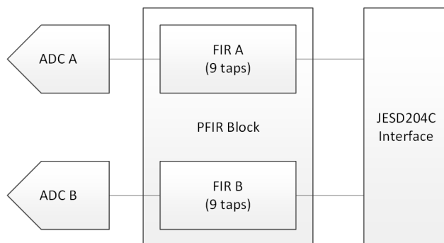
図 6-4. Dual Channel Equalization PFIR Block Diagram
