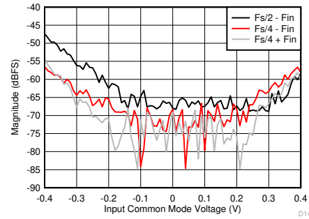
5-98. F_s/2 - F_{\text{IN}} and F_s/4 \pm F_{\text{IN}} vs Input Common Mode Voltage
