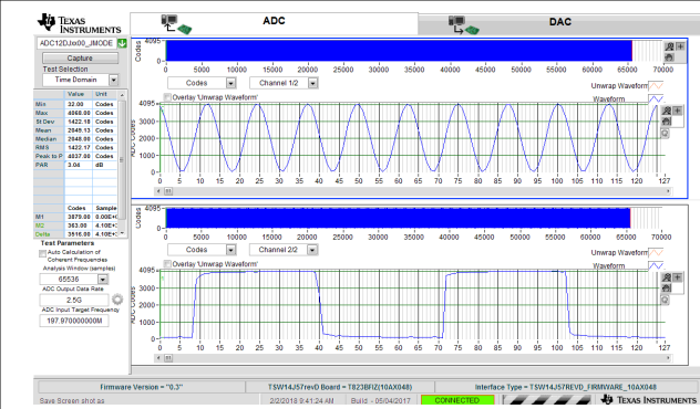
図 7-11. 200-MHz, Sine-Wave (Channel A) and 40-MHz, Square-Wave (Channel B) Time Domain for 5-GSPS, Single-Channel Oscilloscope
