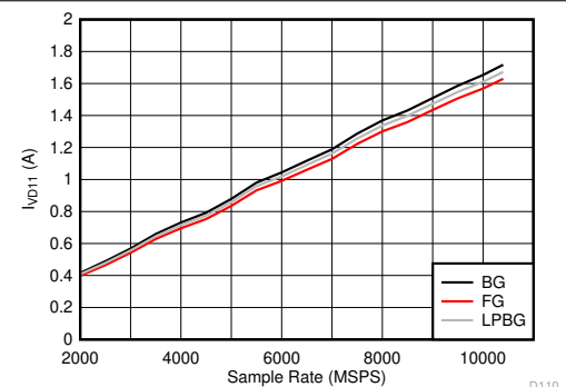
5-126. DES Mode: I_{VD11} vs Sample Rate
