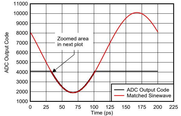
5-148. Sinewave Overdrive Recovery
