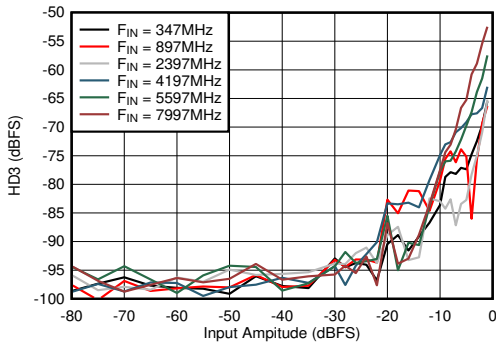
5-63. DES Mode: HD3 vs Input Amplitude and Frequency
