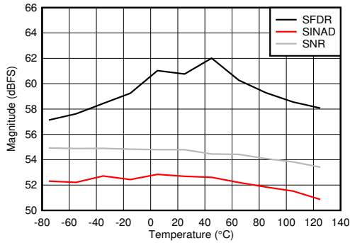
5-85. DES Mode: SNR, SINAD and SFDR vs Temperature
