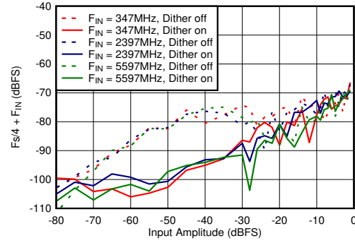
图 5-68. DES Mode: F_s/4 + F_{IN} vs Input Amplitude and Dither
