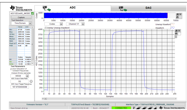
7-7. 40-MHz, Square-Wave Time Domain for 5-GSPS, Single-Channel Oscilloscope
