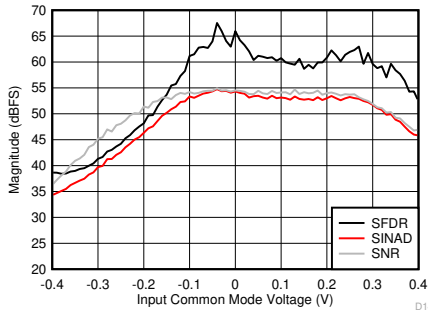
5-97. SNR, SFDR and SINAD vs Input Common Mode Voltage
