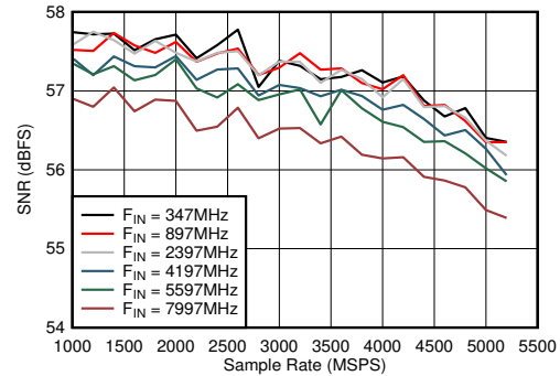
图 5-44. Dual Channel Mode: SNR vs Sample Rate and Input Frequency A_{IN} = -1\text{ dBFS}
