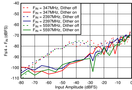
5-66. DES Mode: F_s/2 - F_{\text{IN}} vs Input Amplitude and Dither
