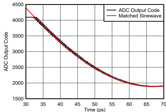
5-149. Sinewave Overdrive Recovery
