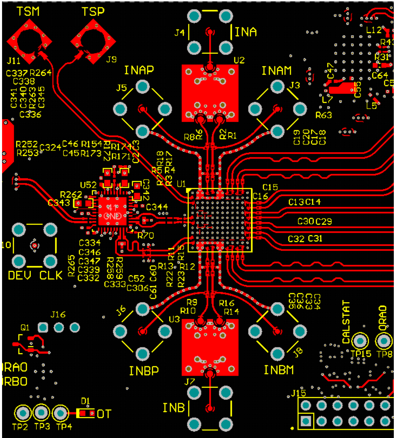
図 7-15. Top Layer Routing: Analog Inputs, CLK and SYSREF, DA0-3, DB0-3
