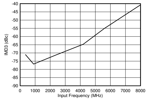
5-104. Dual Channel Mode: IMD3 vs Input Frequency
