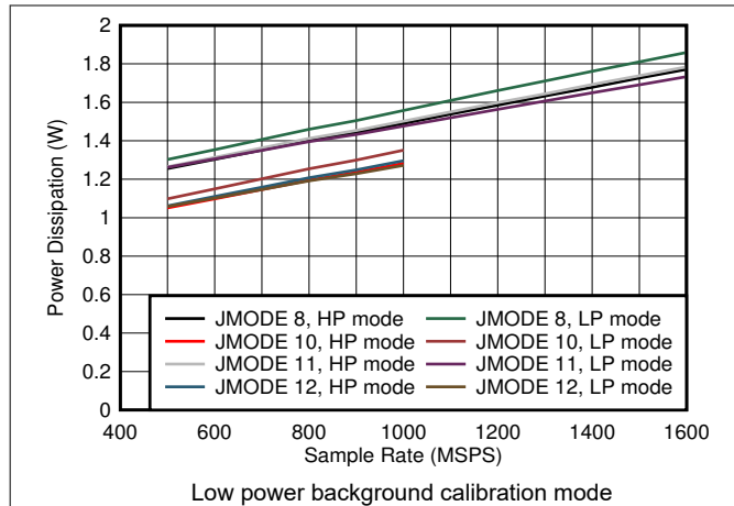
图 5-91. Dual Channel, Power Dissipation vs F_S and JMODE 8 - 12
