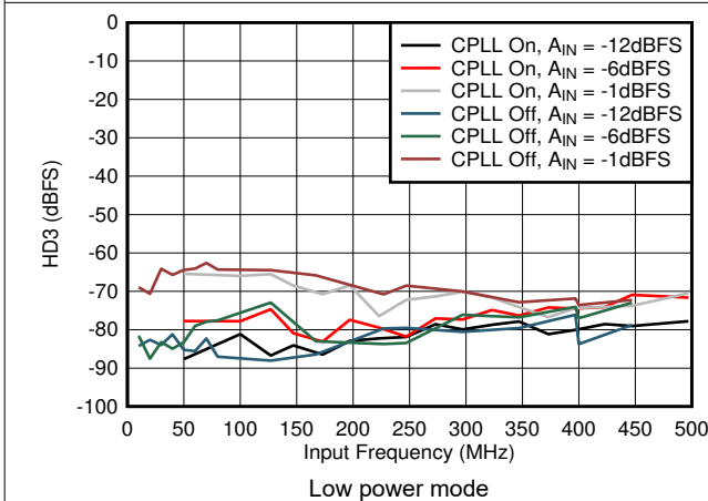
Figure 5-59. HD3 vs A_{IN} and C-PLL
