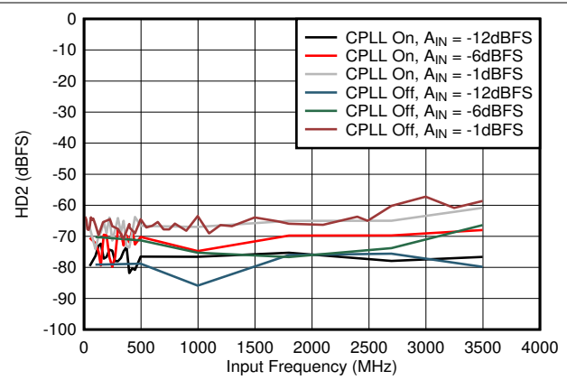
Figure 5-52. HD2 vs A_{IN} and C-PLL
