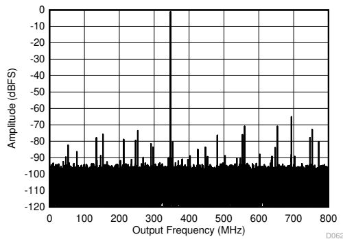
Figure 5-5. Single Tone FFT at 347 MHz and -1 dBFS High power mode, C-PLL on
