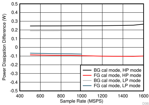
Difference to lower power background calibration, JMODE independent 5-109. Quad Channel, Power Dissipation Change with Calibration Mode
