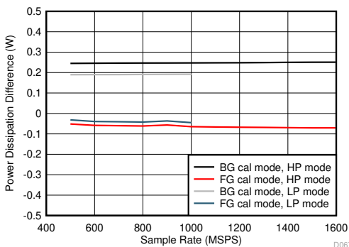
Difference to lower power background calibration, JMODE independent 5-111. Single Channel, Power Dissipation Change with Calibration Mode
