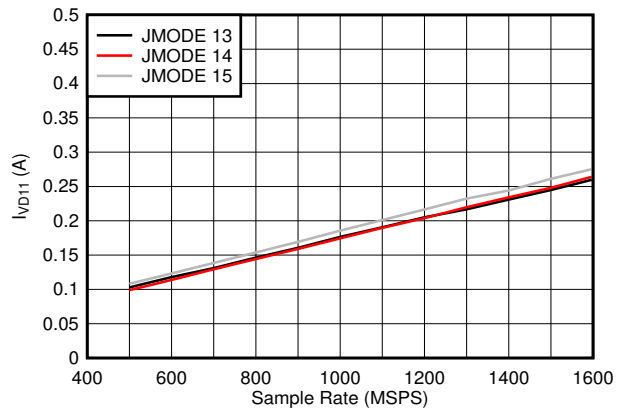
Low power background calibration mode 5-108. Single Channel, I_{VD11} vs F_S and JMODE 13 - 15
