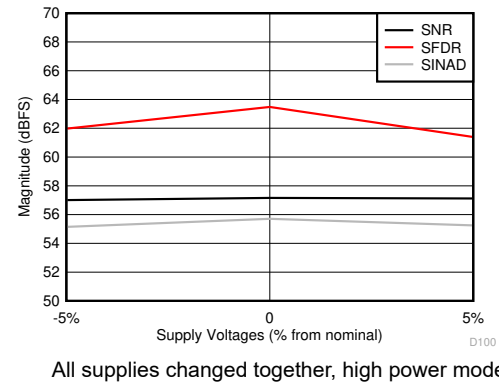
Figure 5-60. SNR, SFDR and SINAD vs Supply Voltage
