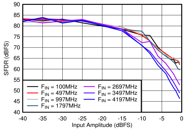
Figure 5-32. SFDR vs A_{IN}
