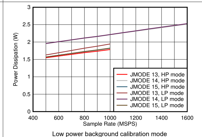
5-82. Quad Channel, Power Dissipation vs F_S and JMODE 13 - 15
