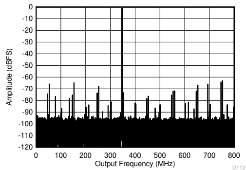
Figure 5-6. Single Tone FFT at 347 MHz and -1 dBFS High power mode, C-PLL on, Noise suppression off
