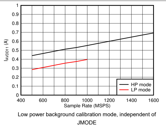
图 5-84. Quad Channel, I_{VDD11} vs F_S
