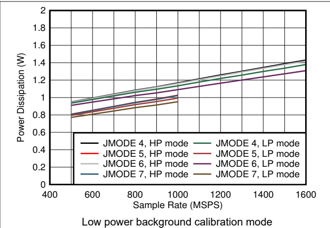
5-100. Single Channel, Power Dissipation vs F_S and JMODE 4 - 7
