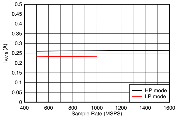
5-103. Single Channel, I_{VA19} vs F_S
