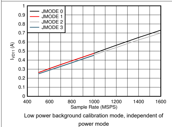
图 5-85. Quad Channel, I_{VD11} vs F_S and JMODE 0 - 3
