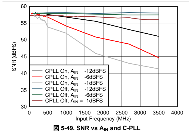
Figure 5-49. SNR vs A_{IN} and C-PLL
