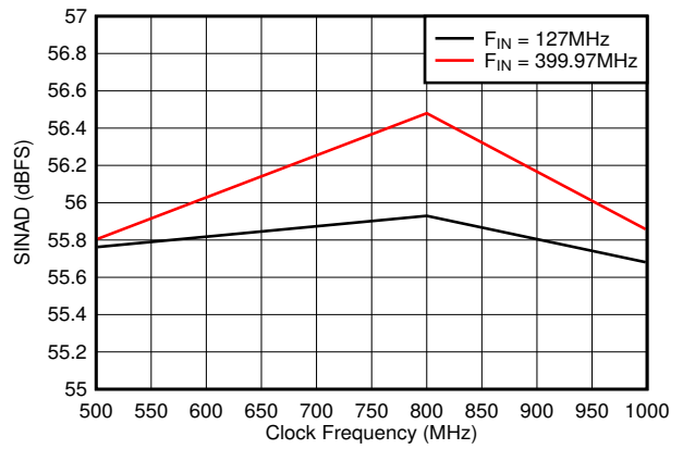
Figure 5-30. SINAD vs Sample Rate
