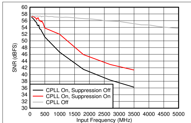
5-41. SNR vs F_{IN} and C-PLL modes
