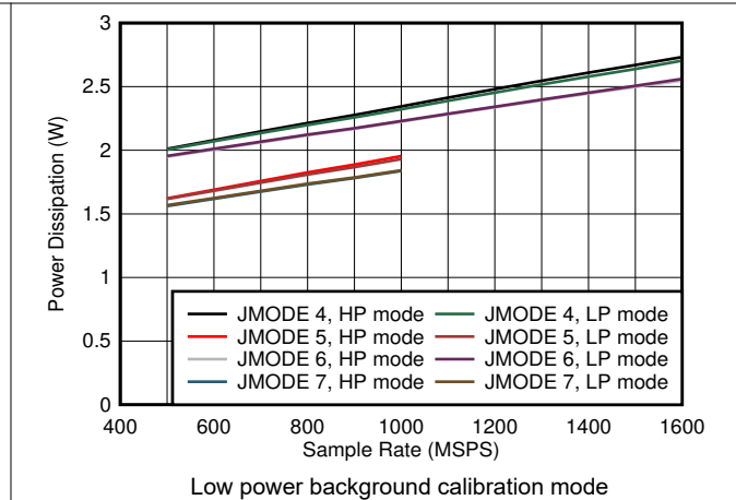
5-80. Quad Channel, Power Dissipation vs F_S and JMODE 4 - 7
