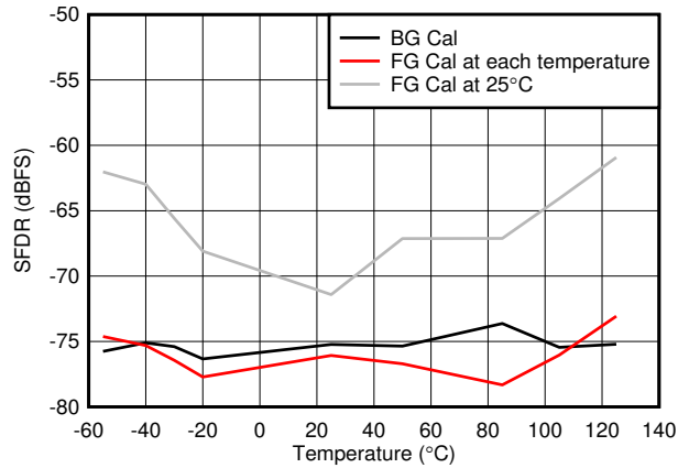
5-68. Worst Spur vs Temperature
