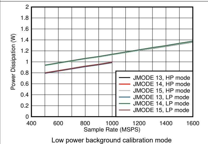
5-102. Single Channel, Power Dissipation vs F_S and JMODE 13 - 15
