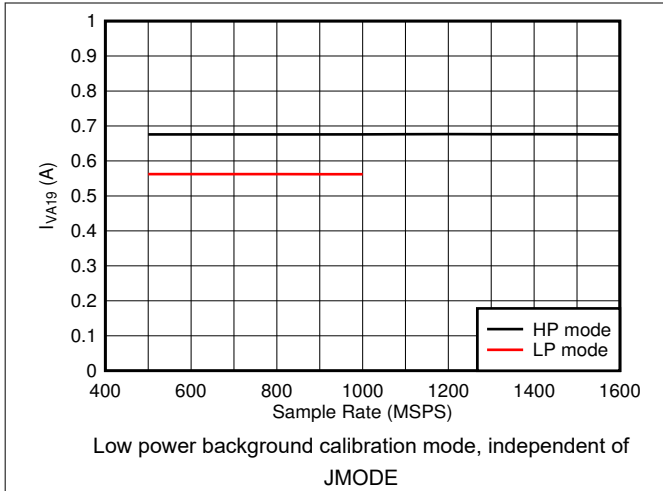
图 5-83. Quad Channel, I_{VA19} vs F_S
