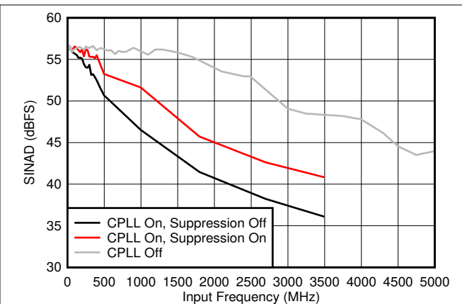
5-42. SINAD vs F_{IN} and C-PLL modes
