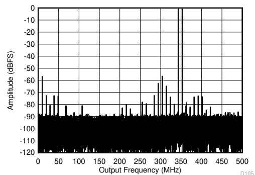
5-70. Two Tone FFT at 1798MHz
