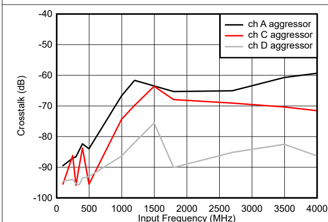
図 5-5. Crosstalk vs Input Frequency, Channel B victim
