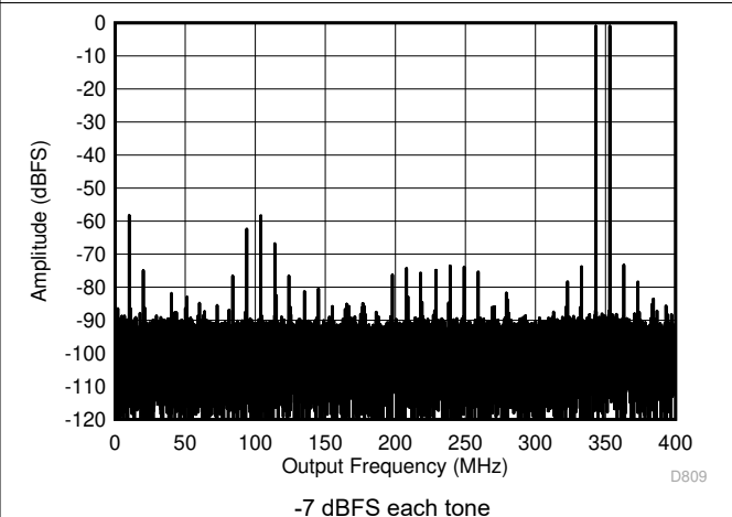
Figure 5-66. Two Tone FFT at 347 MHz
