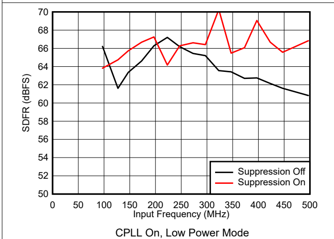
5-61. SFDR vs Input Frequency
