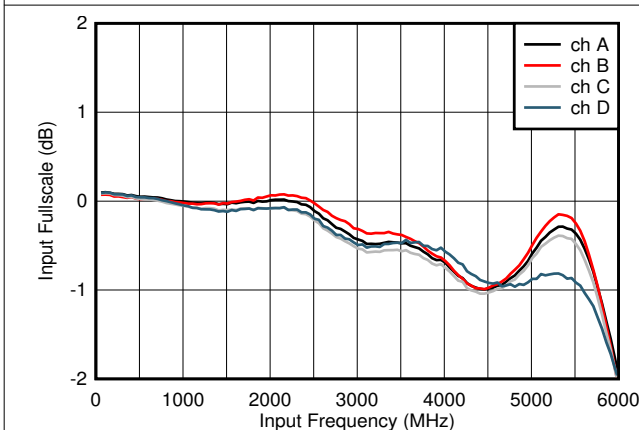
図 5-3. Input Fullscale vs Input Frequency
