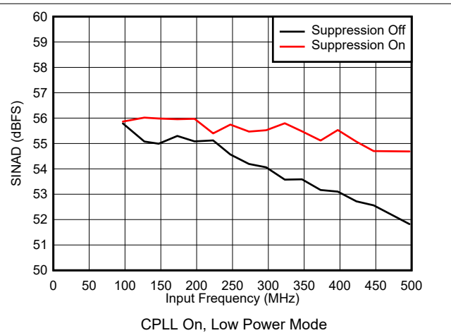
5-62. SINAD vs Input Frequency
