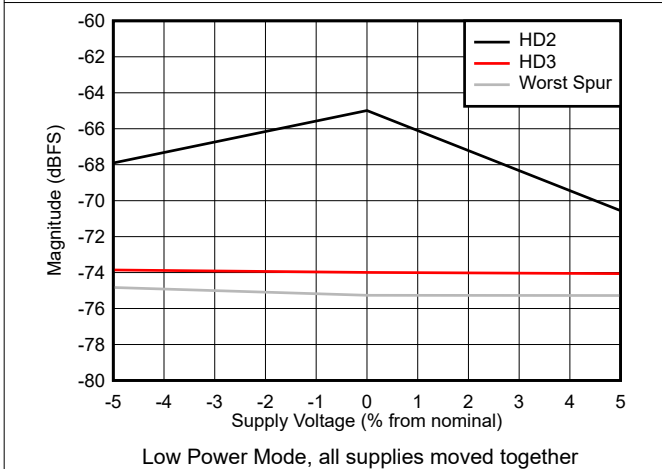
Figure 5-65. HD2, HD3 and worst non-HD vs Supply Voltage
