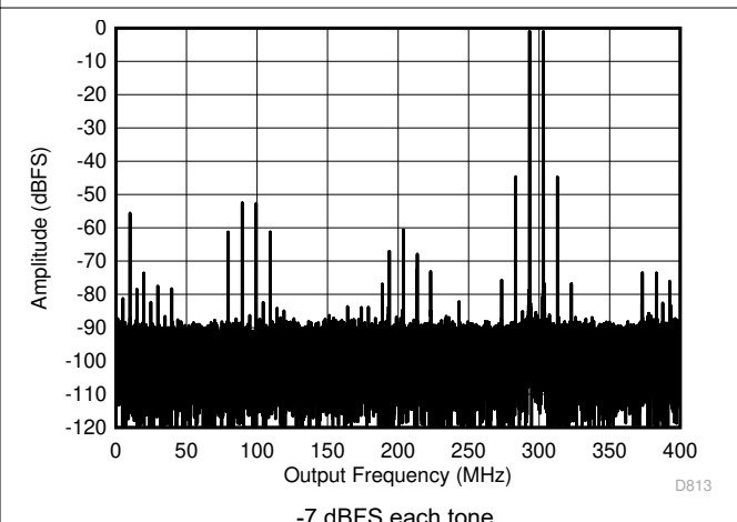
Figure 5-68. Two Tone FFT at 3498 MHz
