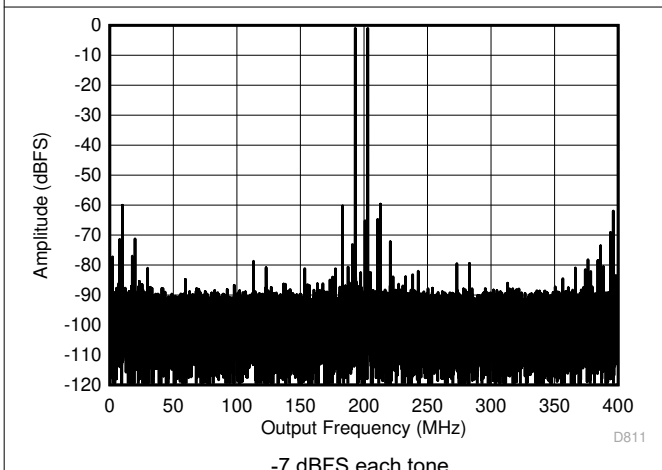
Figure 5-67. Two Tone FFT at 1798 MHz
