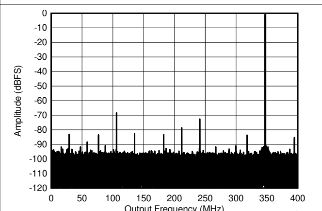
図 5-6. Single Tone FFT at 347 MHz and -1dBFS
