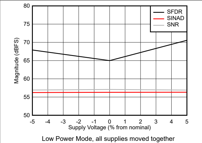
Figure 5-64. SNR, SFDR and SINAD vs Supply Voltage
