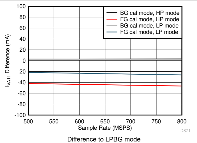
图 5-86. Quad Channel, I_{VA11} vs F_S over Modes
