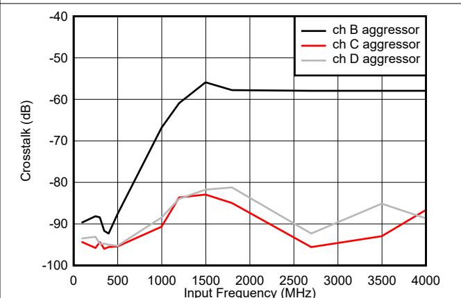
図 5-4. Crosstalk vs Input Frequency, Channel A victim
