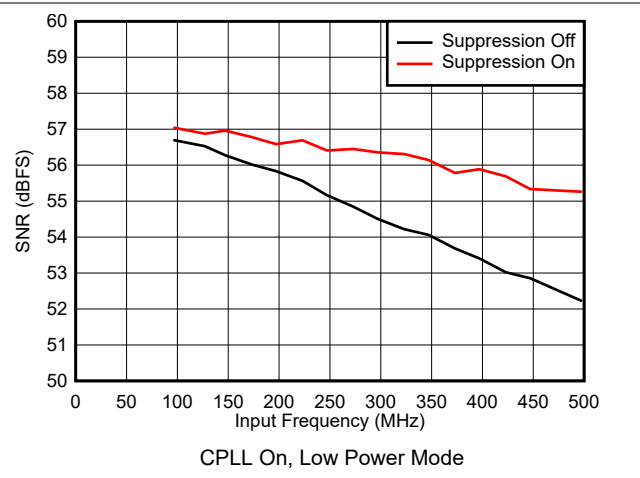
5-60. SNR vs Input Frequency
