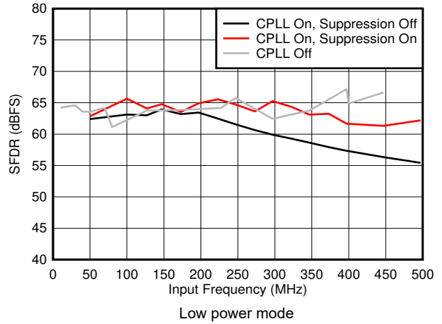
Figure 5-44. SFDR vs F_{IN} and C-PLL modes
