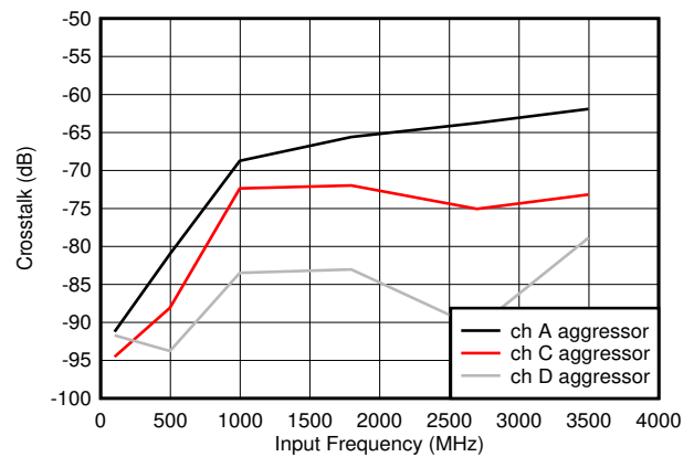
5-78. Crosstalk to Channel B vs F_{IN}
