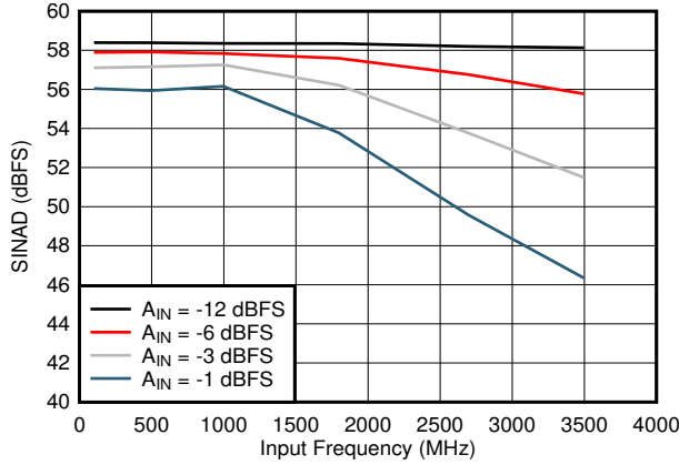
5-19. SINAD vs Input Frequency
