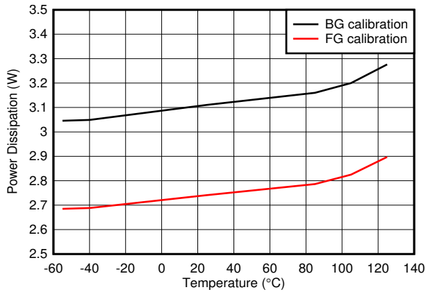
5-121. Quad Channel, Power Dissipation vs Temperature
