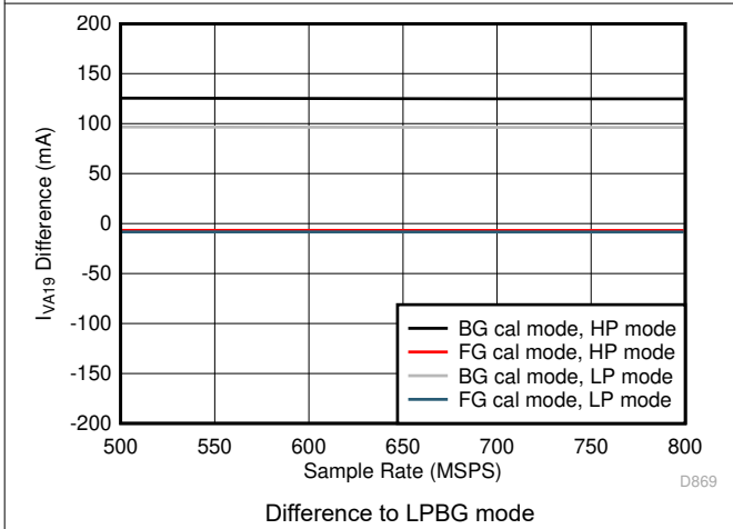
7-99. Dual Channel, I_{VA19} vs F_S over Modes
