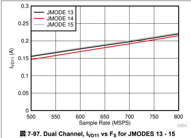
7-97. Dual Channel, I_{VD11} vs F_S for JMODES 13 - 15
