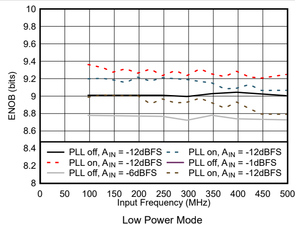
7-53. ENOB vs Input Frequency in Low Power Mode
