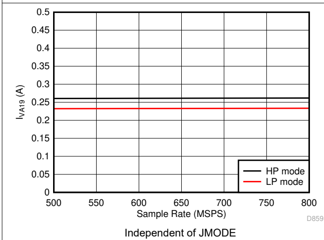
7-105. Single Channel, I_{VA19} vs F_S
