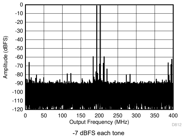
7-70. Two Tone FFT at 1798 MHz in Low Power Mode
