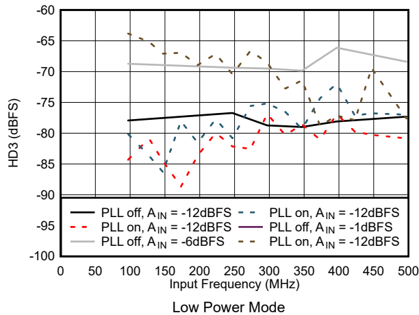
7-51. HD3 vs Input Frequency in Low Power Mode
