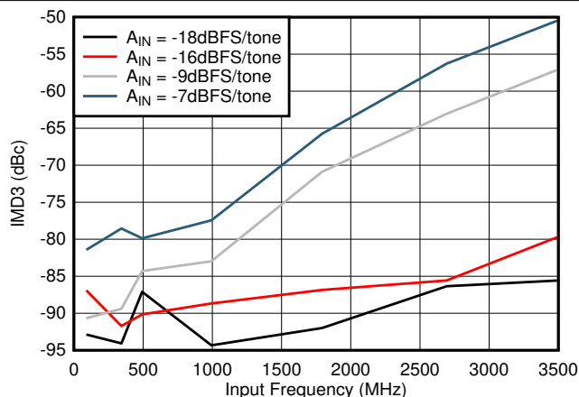
7-72. IMD3 vs Input Frequency
