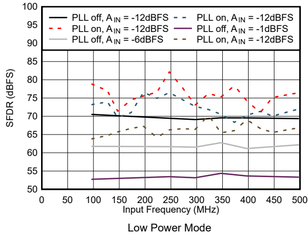
7-49. SFDR vs Input Frequency in Low Power Mode
