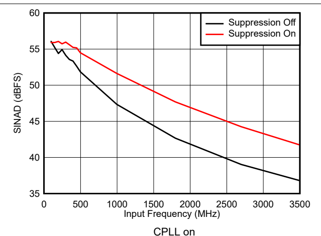
7-36. SINAD vs Input Frequency and Suppression
