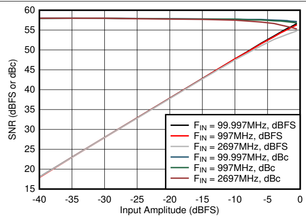
7-32. SNR vs Input Amplitude
