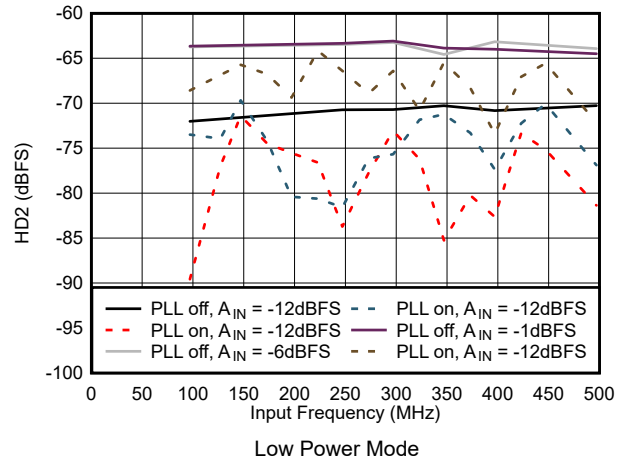
7-50. HD2 vs Input Frequency in Low Power Mode
