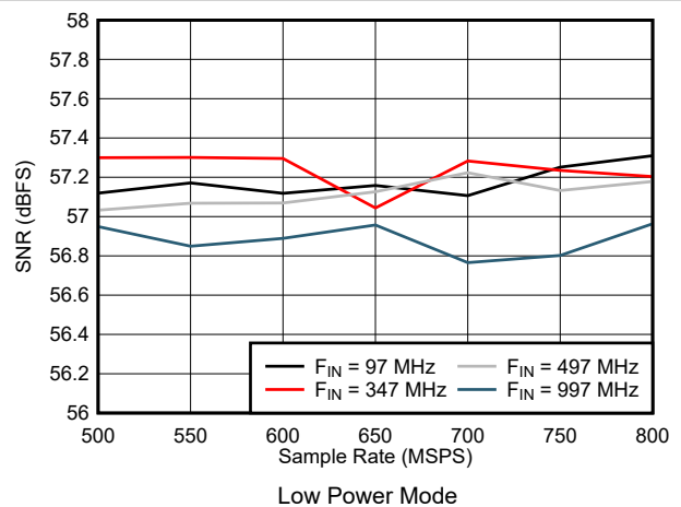
7-54. SNR vs Sample Rate in Low Power Mode
