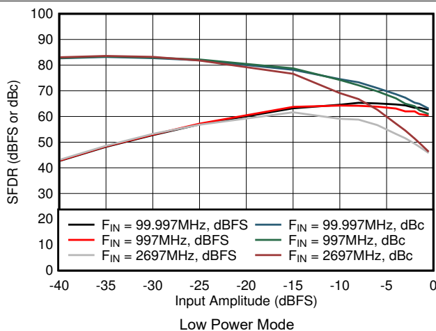
7-59. SFDR vs Input Amplitude in Low Power Mode
