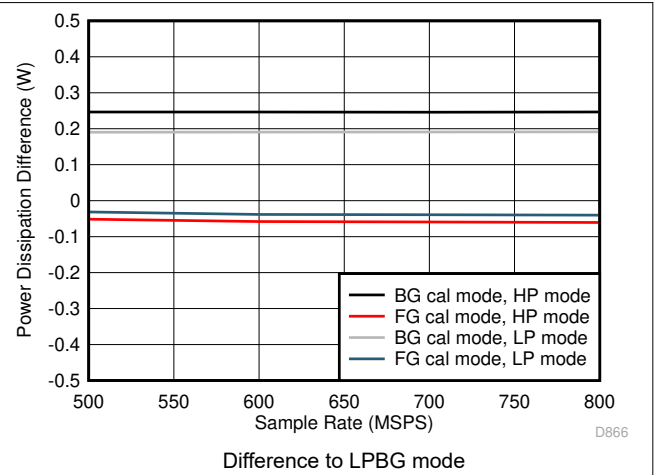
7-98. Dual Channel, Power Dissipation vs F_S over Modes
