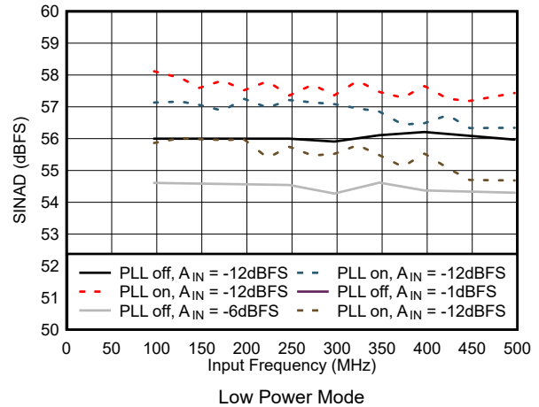
7-52. SINAD vs Input Frequency in Low Power Mode
