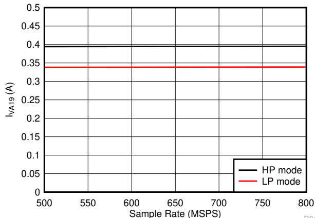
7-92. Dual Channel, I_{VA19} vs F_S Independent of JMODE
