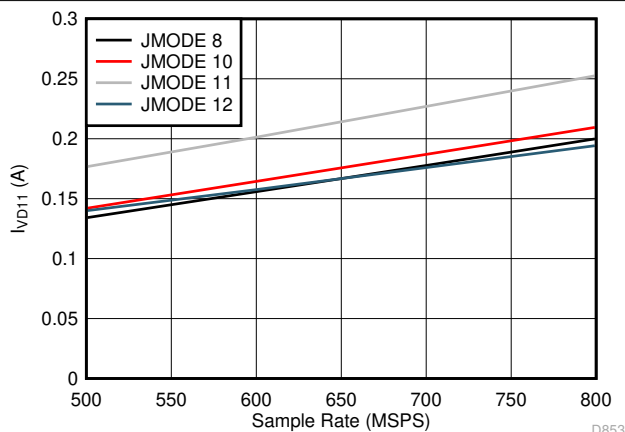
7-96. Dual Channel, I_{VD11} vs F_S for JMODES 8 - 12
