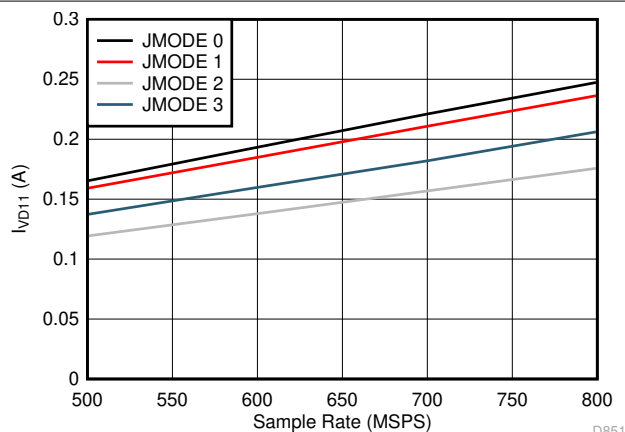
7-94. Dual Channel, I_{VD11} vs F_S for JMODES 0 - 3
