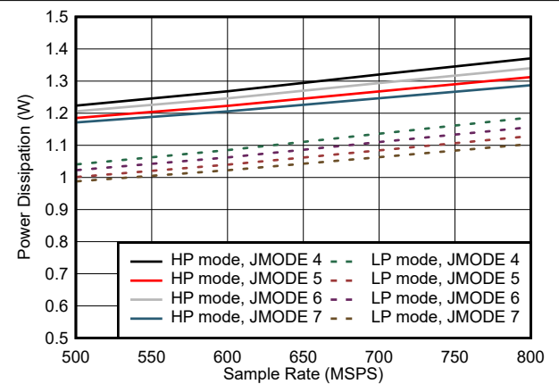
7-89. Dual Channel, Power Dissipation vs F_S for JMODES 4 - 7
