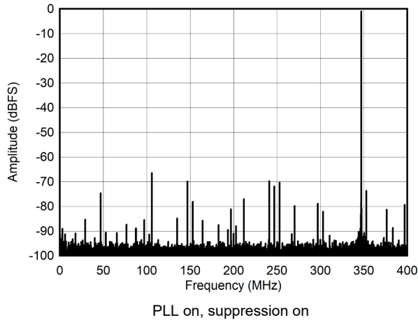
7-15. Single Tone FFT at 347 MHz and -1dBFS
