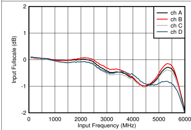
Figure 7-3. Input Fullscale vs Input Frequency
