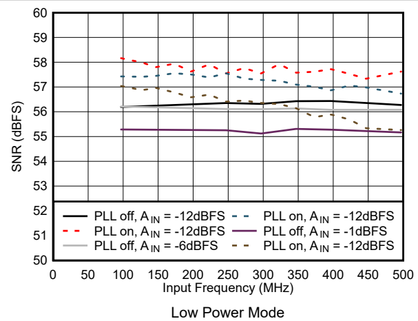
7-48. SNR vs Input Frequency in Low Power Mode
