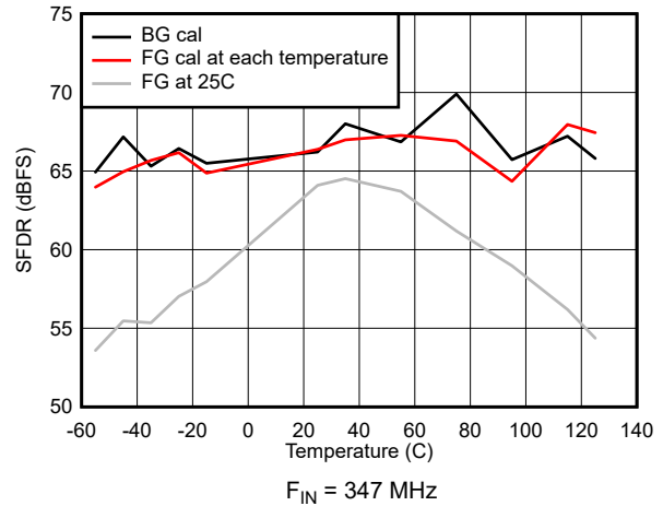
7-44. SFDR vs Temperature
