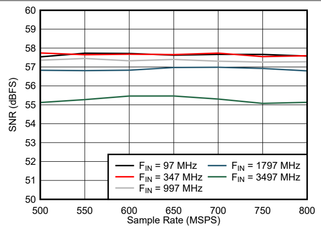
7-28. SNR vs Sample Rate
