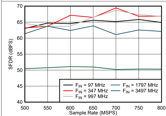
7-29. SFDR vs Sample Rate
