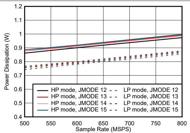
7-104. Single Channel, Power Dissipation vs F_S for JMODES 12 - 15
