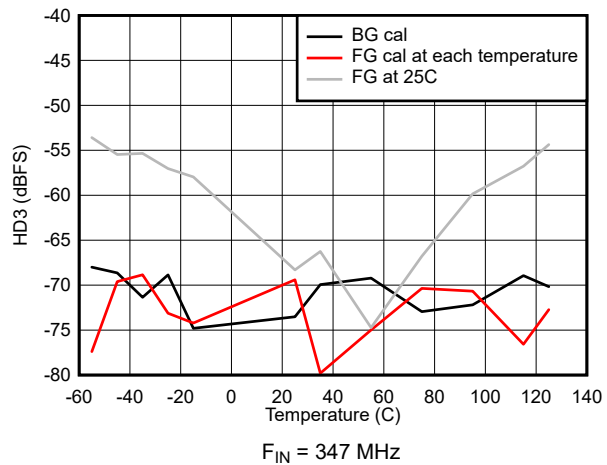
7-46. HD3 vs Temperature
