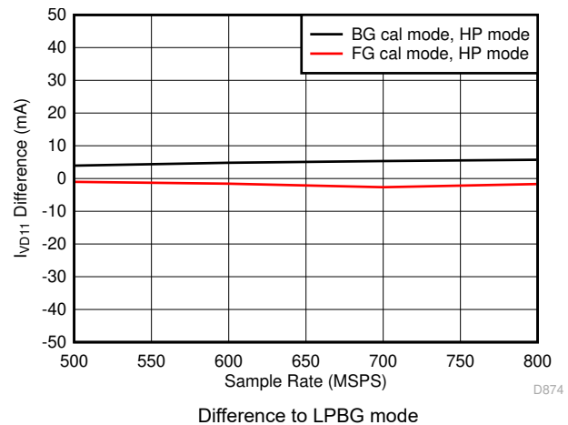
7-87. Quad Channel, I_{VD11} vs F_S over Modes
