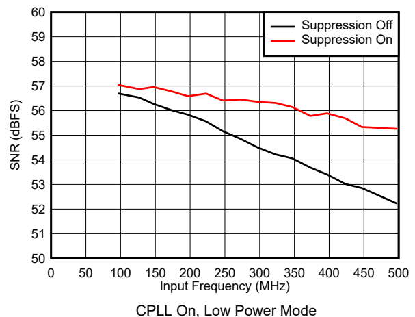
7-60. SNR vs Input Frequency
