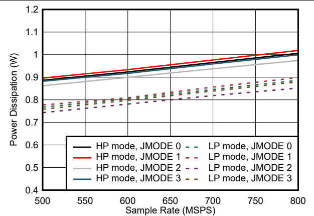
7-101. Dual Channel, Power Dissipation vs F_S for JMODES 0 - 3
