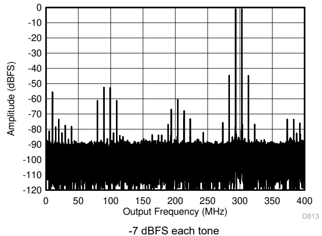
7-68. Two Tone FFT at 3498 MHz
