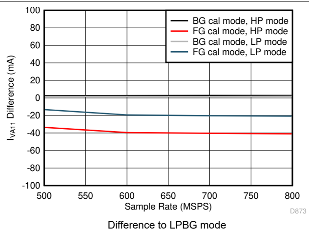
7-113. Single Channel, I_{VA11} vs F_S over Modes
