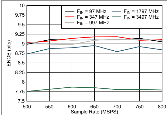
7-31. ENOB vs Sample Rate
