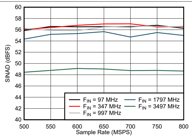
7-30. SINAD vs Sample Rate
