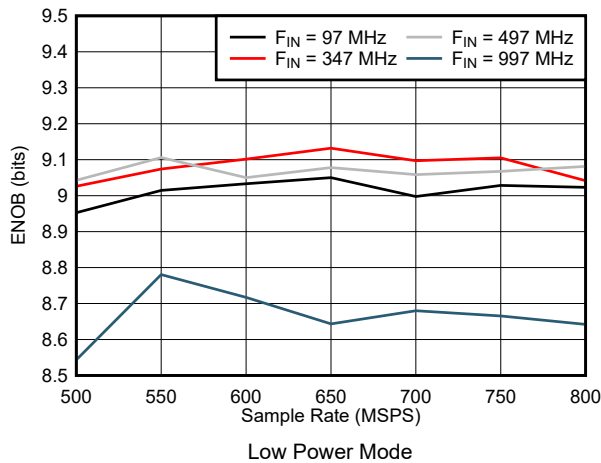
7-57. ENOB vs Sample Rate in Low Power Mode
