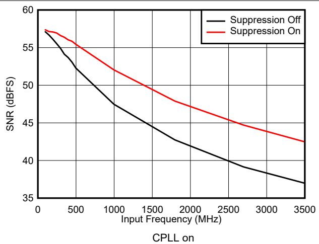
7-34. SNR vs Input Frequency and Suppression
