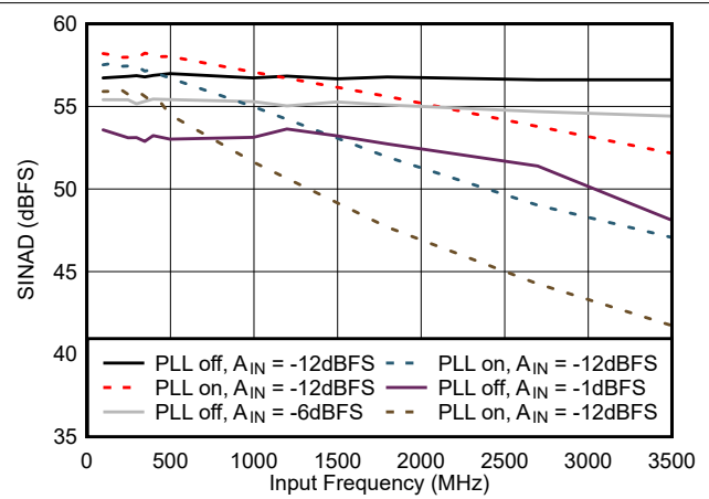
7-26. SINAD vs Input Frequency
