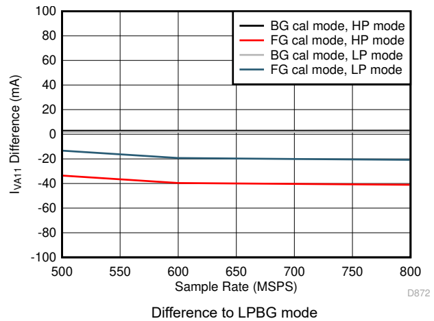
7-100. Dual Channel, I_{VA11} vs F_S over Modes
