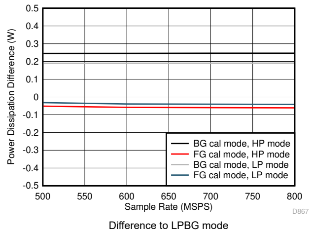
7-111. Single Channel, Power Dissipation vs F_S over Modes
