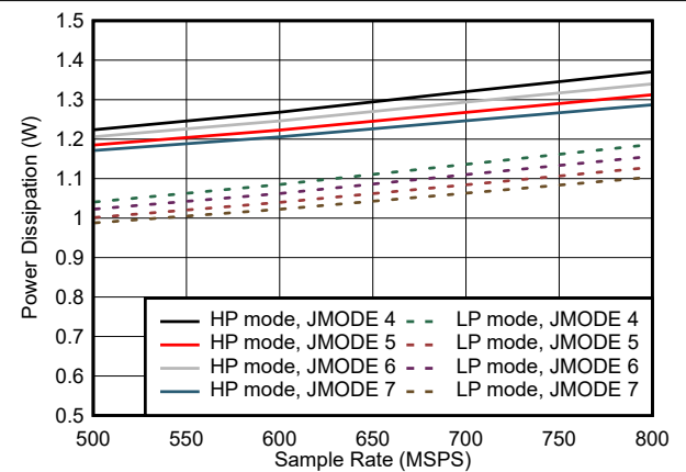
7-89. Dual Channel, Power Dissipation vs F_S for JMODES 4 - 7
