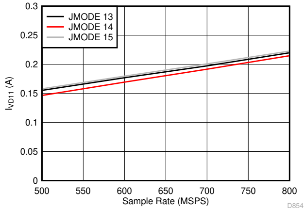
7-97. Dual Channel, I_{VD11} vs F_S for JMODES 13 - 15
