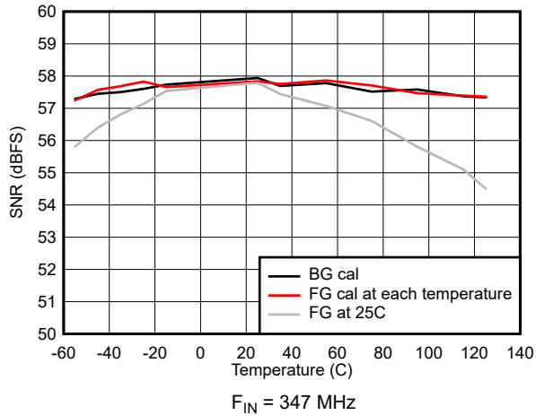
7-43. SNR vs Temperature
