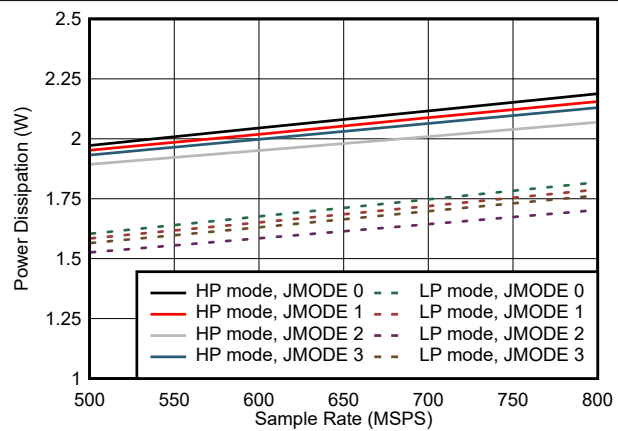
7-74. Quad Channel, Power Dissipation vs F_S for JMODES 0 - 3
