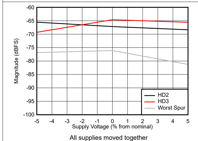
7-39. HD2, HD3 and worst non-HD vs Supply Voltage
