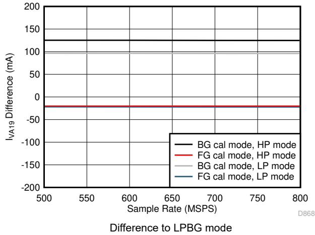
7-85. Quad Channel, I_{VA19} vs F_S over Modes
