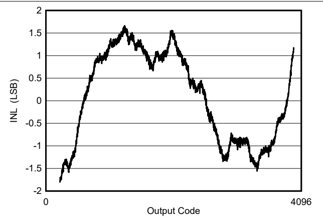
Figure 7-2. INL vs Code
