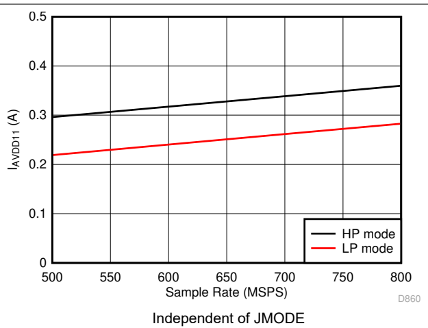
7-106. Single Channel, I_{VA11} vs F_S
