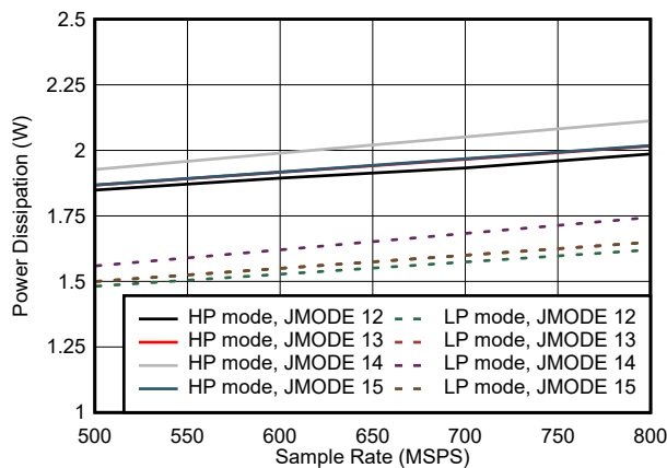
7-77. Quad Channel, Power Dissipation vs F_S for JMODES 12 - 15
