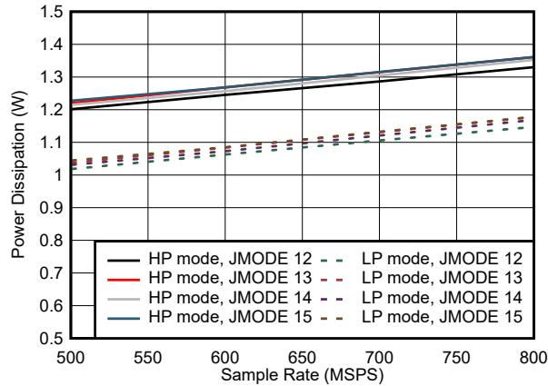
7-91. Dual Channel, Power Dissipation vs F_S for JMODES 12 - 15
