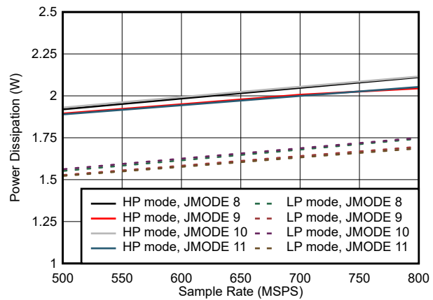
7-76. Quad Channel, Power Dissipation vs F_S for JMODES 8 - 11
