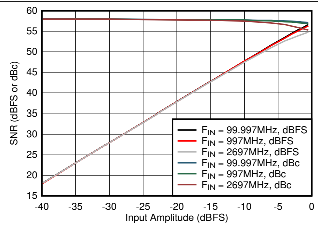
7-32. SNR vs Input Amplitude
