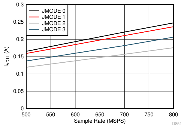
7-94. Dual Channel, I_{VD11} vs F_S for JMODES 0 - 3
