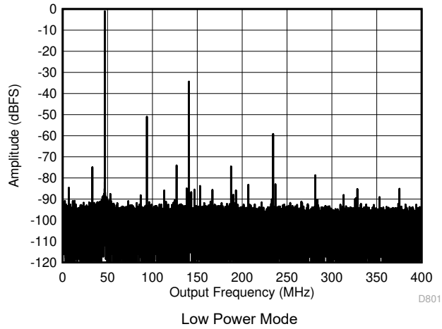
7-13. Single Tone FFT at 3247 MHz and -1dBFS
