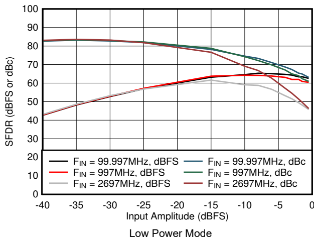
7-59. SFDR vs Input Amplitude in Low Power Mode
