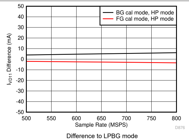
7-114. Single Channel, I_{VD11} vs F_S over Modes
