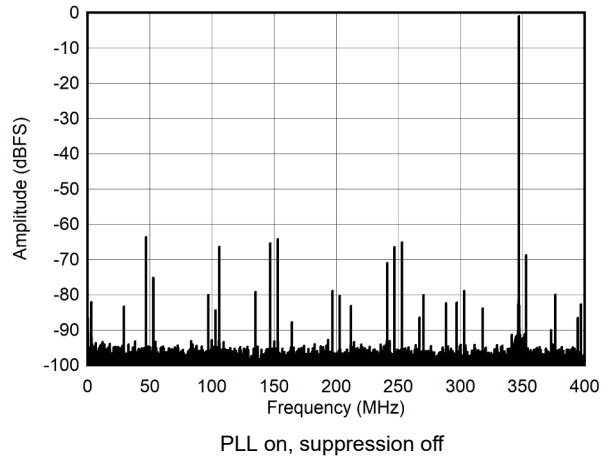
7-14. Single Tone FFT at 347 MHz and -1dBFS
