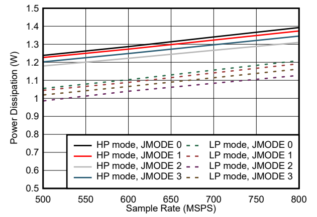
7-88. Dual Channel, Power Dissipation vs F_S for JMODES 0 - 3
