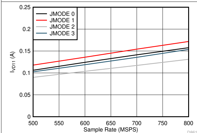
7-107. Single Channel, I_{VD11} vs F_S for JMODES 0 - 3
