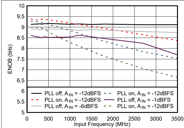
7-27. ENOB vs Input Frequency
