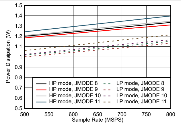
7-90. Dual Channel, Power Dissipation vs F_S for JMODES 8 - 11
