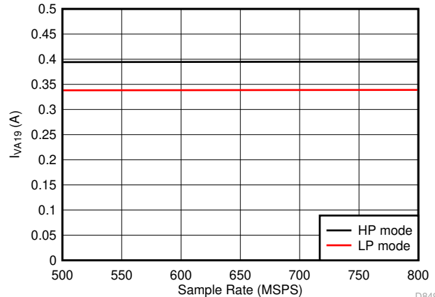
7-92. Dual Channel, I_{VA19} vs F_S Independent of JMODE
