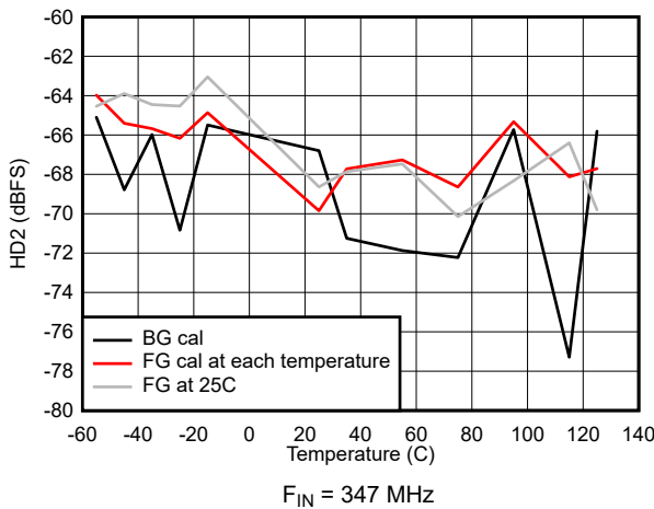
7-45. HD2 vs Temperature
