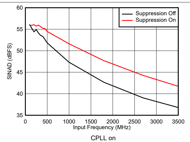
7-36. SINAD vs Input Frequency and Suppression
