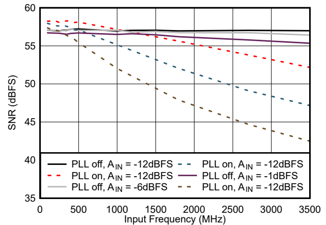
FIG 7-22. SNR vs Input Frequency
