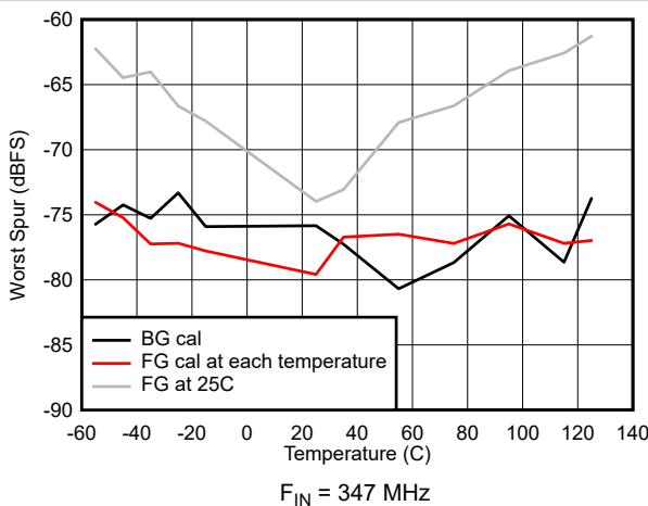
7-47. worst non-HD spur vs Temperature
