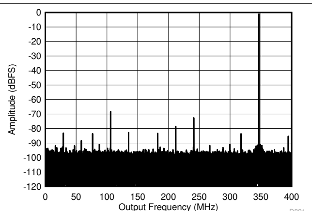
Figure 7-6. Single Tone FFT at 347 MHz and -1dBFS
