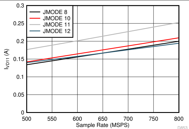
7-96. Dual Channel, I_{VD11} vs F_S for JMODES 8 - 12
