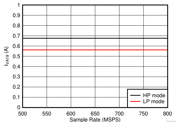
7-78. Quad Channel, I_{VA19} vs F_S Independent of JMODE
