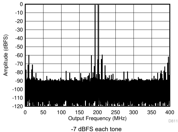
7-67. Two Tone FFT at 1798 MHz
