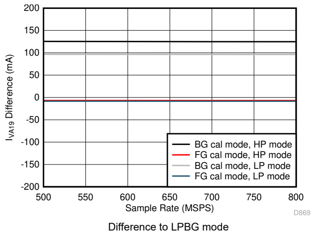
7-99. Dual Channel, I_{VA19} vs F_S over Modes
