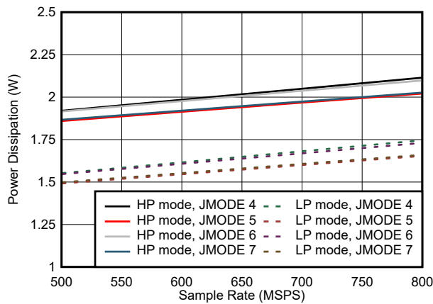
7-75. Quad Channel, Power Dissipation vs F_S for JMODES 4 - 7
