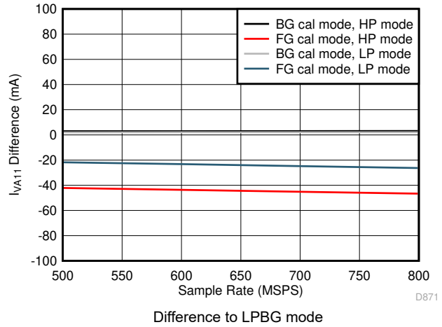
7-86. Quad Channel, I_{VA11} vs F_S over Modes
