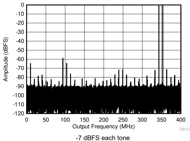
7-69. Two Tone FFT at 347 MHz in Low Power Mode
