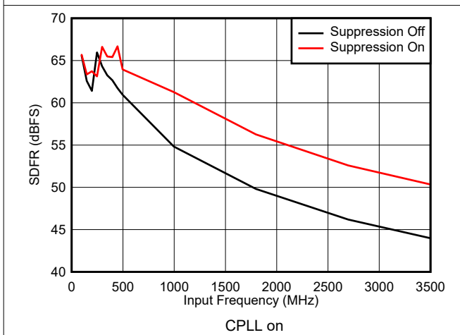
7-35. SFDR vs Input Frequency and Suppression
