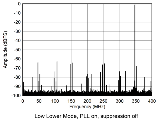
7-18. Single Tone FFT at 347 MHz and -1dBFS
