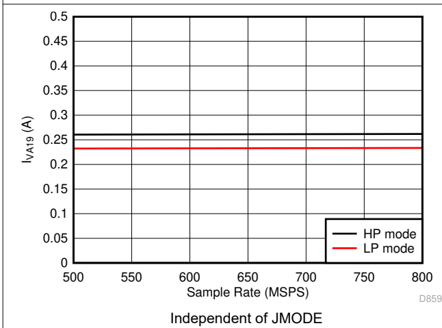
7-105. Single Channel, I_{VA19} vs F_S
