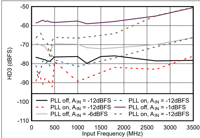
7-25. HD3 vs Input Frequency
