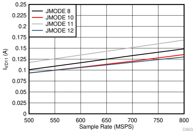
7-109. Single Channel, I_{VD11} vs F_S for JMODES 8 - 12
