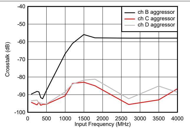
Figure 7-4. Crosstalk vs Input Frequency, Channel A victim
