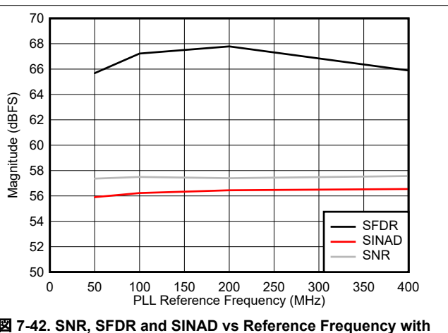
7-42. SNR, SFDR and SINAD vs Reference Frequency with PLL on
