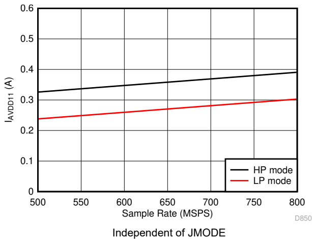
7-93. Dual Channel, I_{VA11} vs F_S
