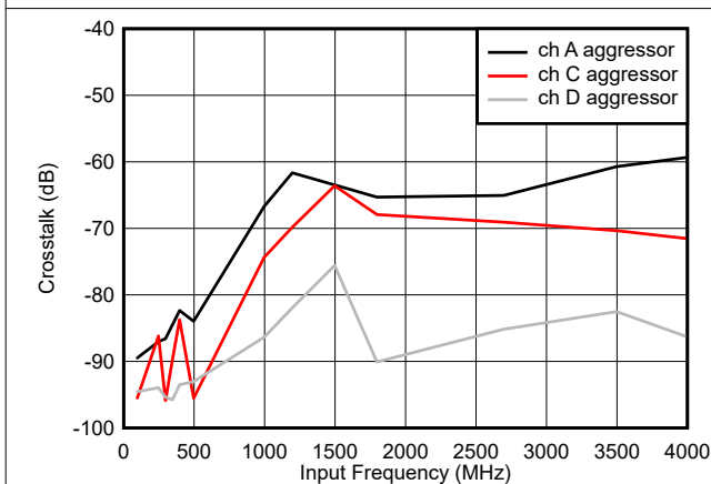
Figure 7-5. Crosstalk vs Input Frequency, Channel B victim
