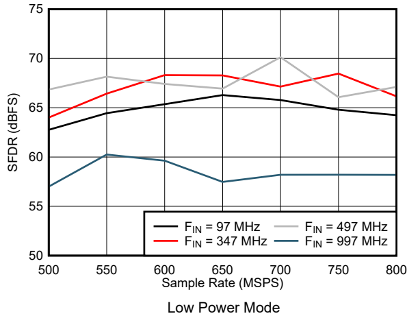
7-55. SFDR vs Sample Rate in Low Power Mode
