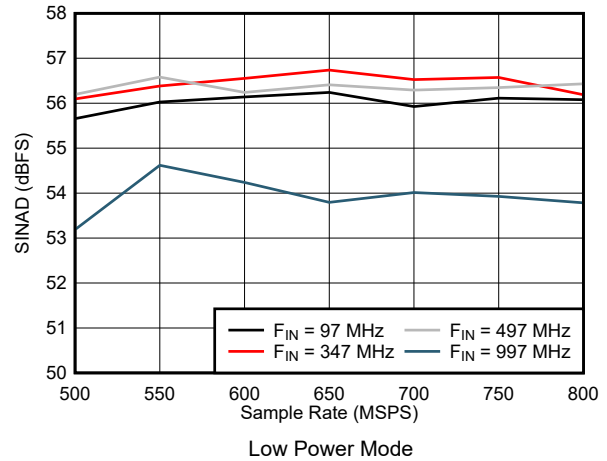
7-56. SINAD vs Sample Rate in Low Power Mode
