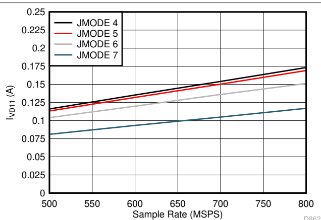
7-108. Single Channel, I_{VD11} vs F_S for JMODES 4 - 7
