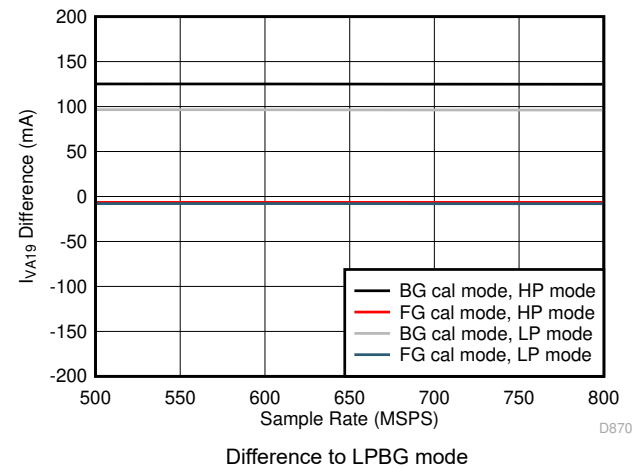
7-112. Single Channel, I_{VA19} vs F_S over Modes
