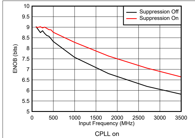
7-37. ENOB vs Input Frequency and Suppression
