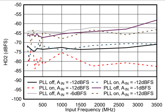
FIG 7-24. HD2 vs Input Frequency
