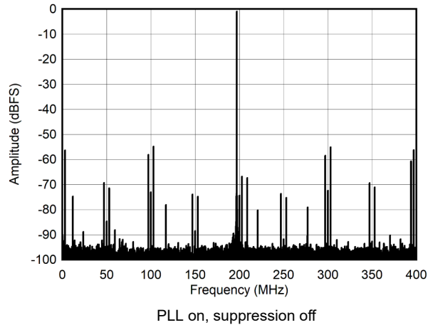
7-16. Single Tone FFT at 997 MHz and -1dBFS
