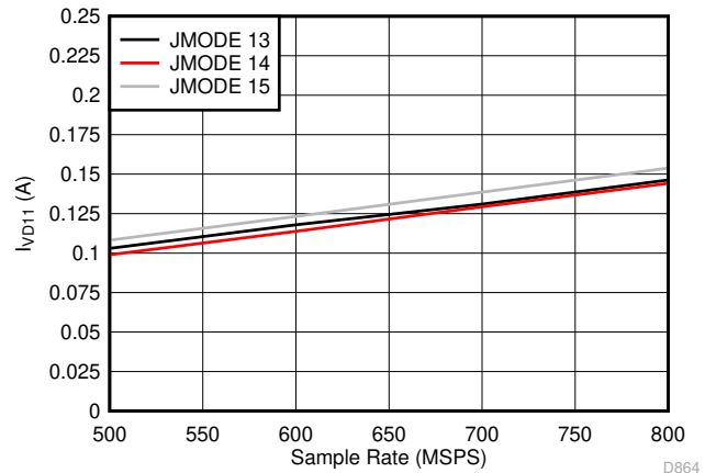
7-110. Single Channel, I_{VD11} vs F_S for JMODES 13 - 15
