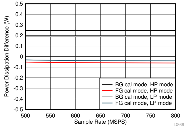
7-98. Dual Channel, Power Dissipation vs F_S over Modes
