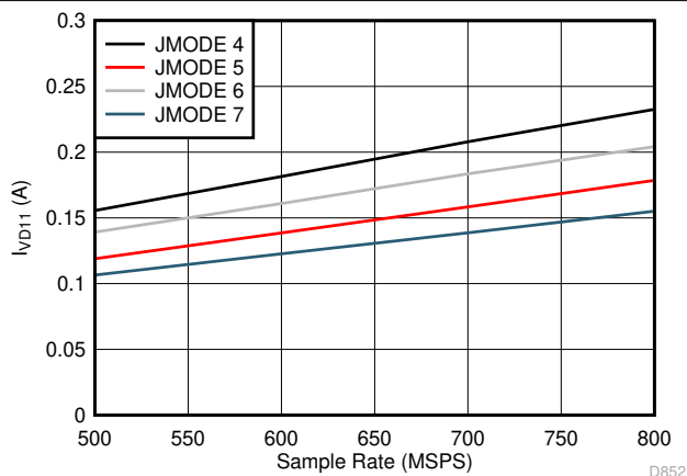
7-95. Dual Channel, I_{VD11} vs F_S for JMODES 4 - 7
