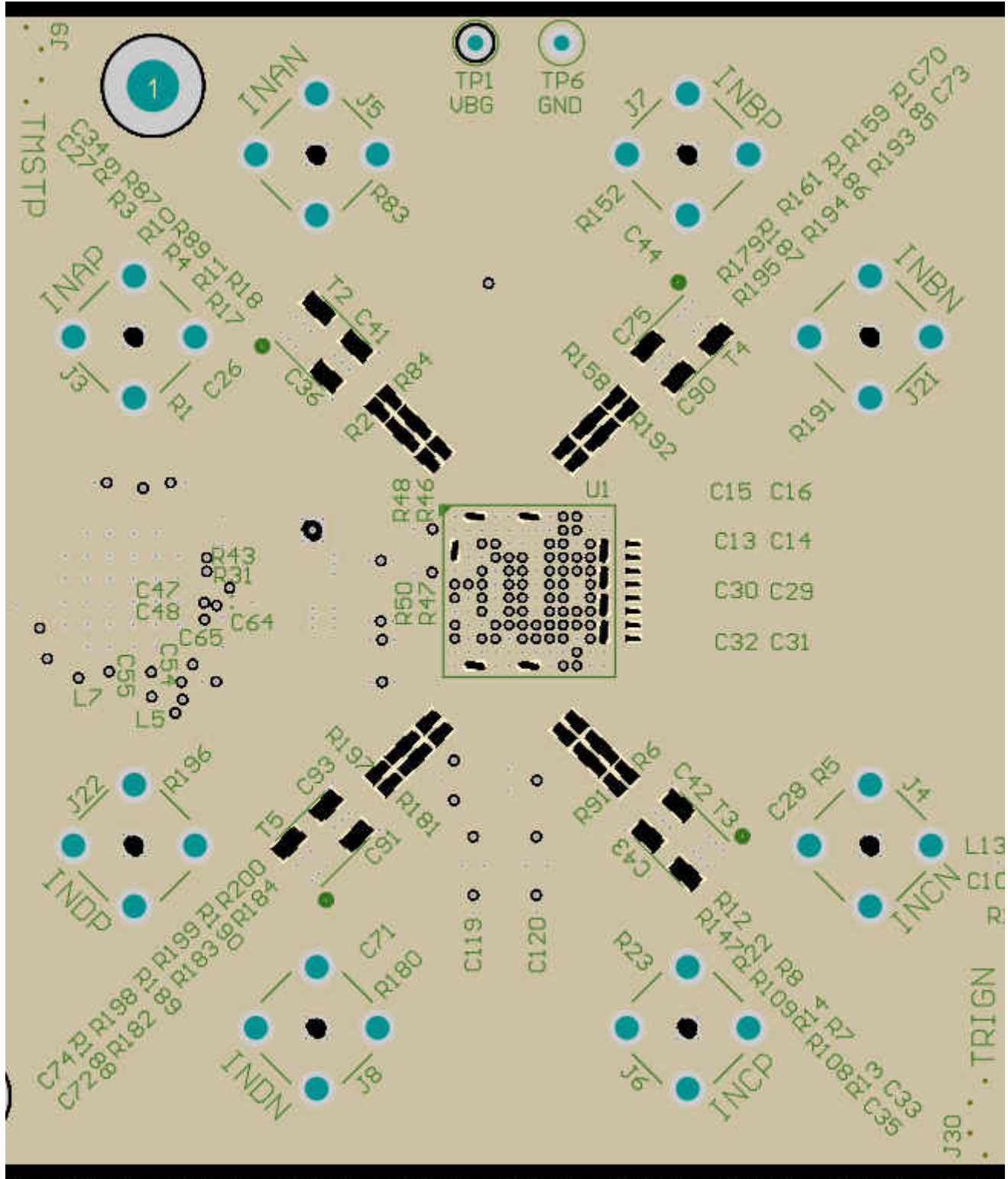
11-2. GND1 Cutouts to Optimize Impedance of Component Pads
