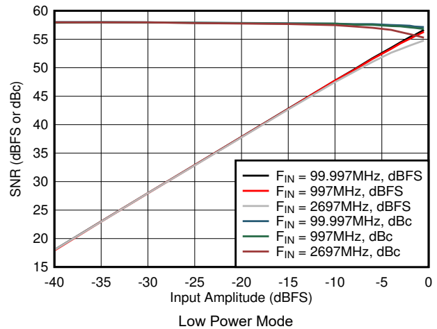
7-58. SNR vs Input Amplitude in Low Power Mode
