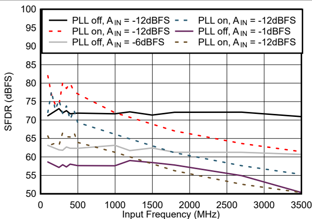
FIG 7-23. SFDR vs Input Frequency
