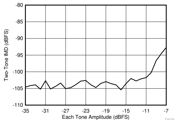
6-76. Intermodulation Distortion vs Input Amplitude (185 MHz and 190 MHz)
