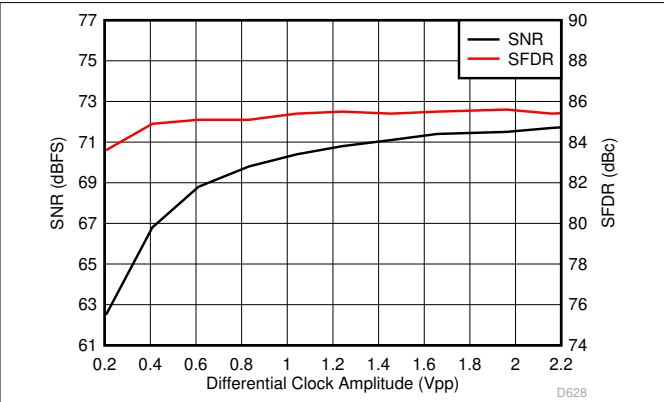
6-58. Performance vs Differential Clock Amplitude (150 MHz)
