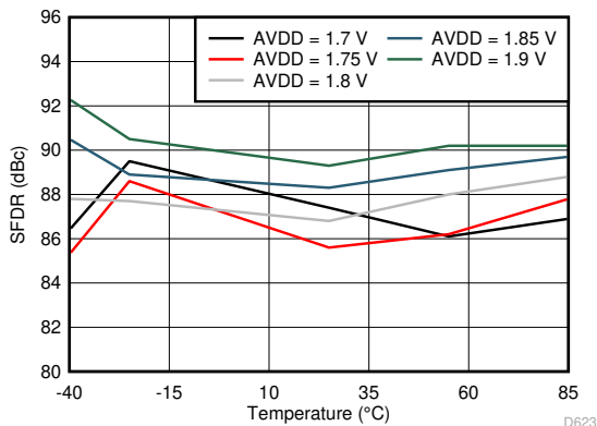
6-53. Spurious-Free Dynamic Range vs AVDD Supply and Temperature (30 MHz)
