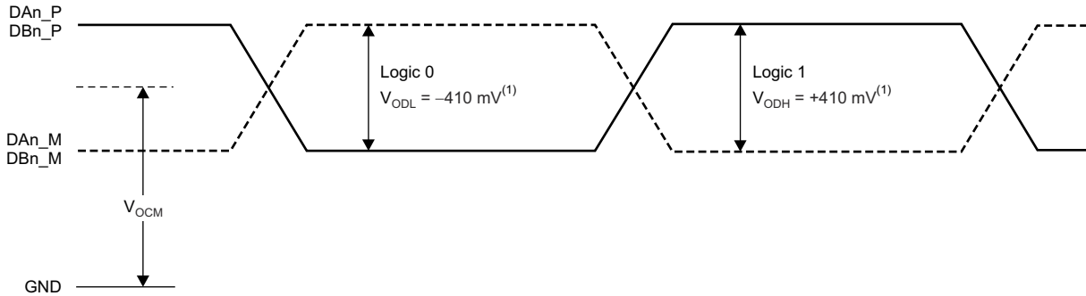
7-1. Serial LVDS Output Voltage Levels
