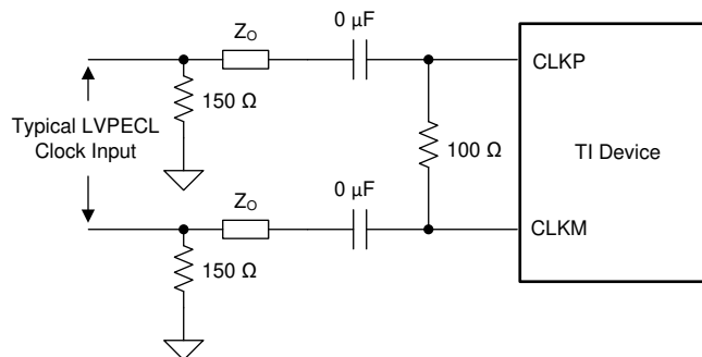
8-3. LVPECL Clock Driving Circuit
