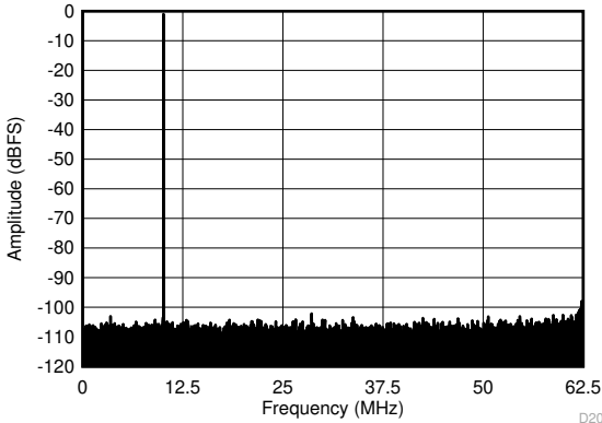
6-91. FFT for 10 MHz Input Signal (Chopper On, Dither On)
