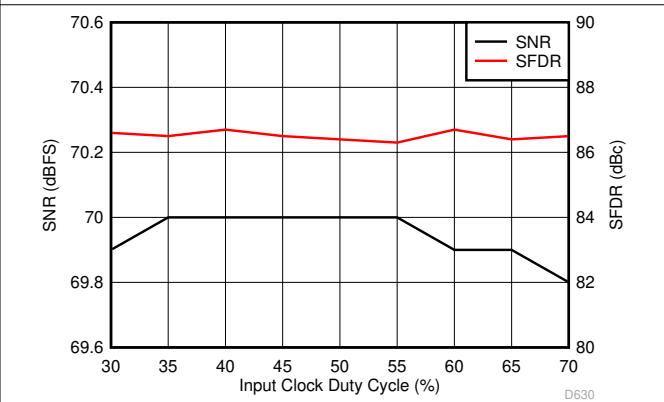
6-60. Performance vs Clock Duty Cycle (150 MHz)
