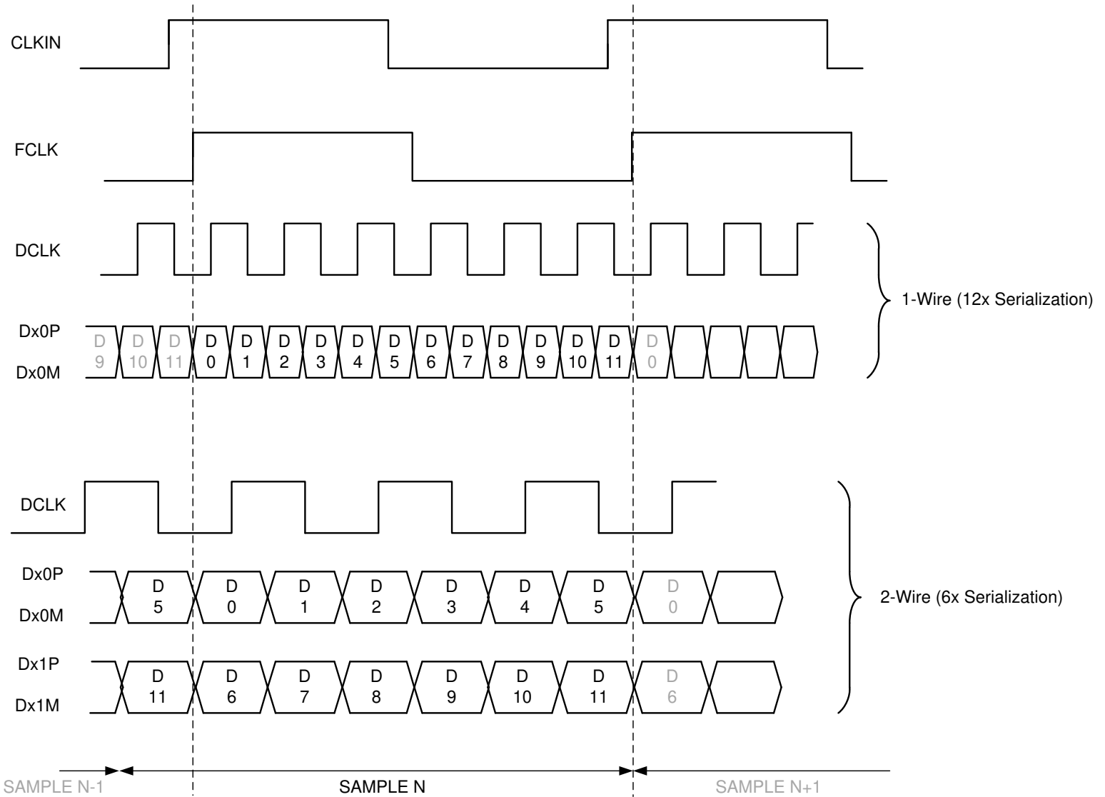
7-2. Output Timing Diagram
