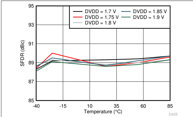
6-85. Spurious-Free Dynamic Range vs DVDD Supply and Temperature (170 MHz)
