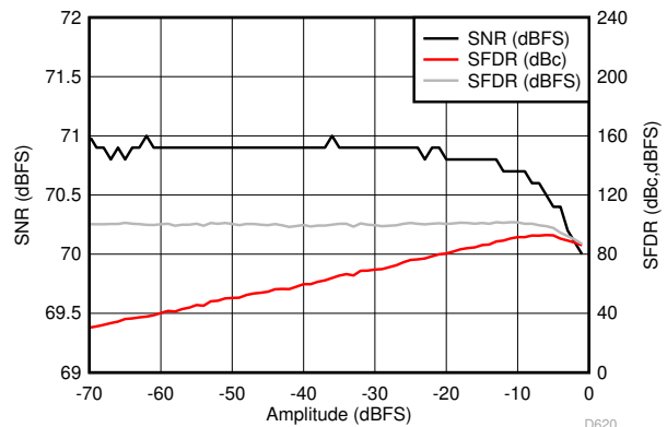
6-50. Performance vs Input Amplitude (170 MHz)
