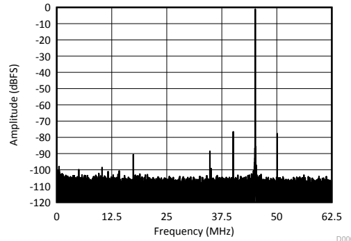
f_{IN} = 170.1\text{ MHz} , f_{CMRR} = 5\text{ MHz} , A_{CMRR} = 50\text{ mV}_{PP} , \text{SINAD} = 69.66\text{ dBFS} , \text{SFDR} = 75.66\text{ dBc}
