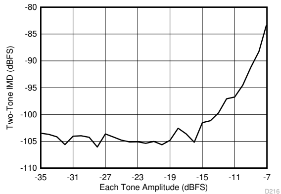
FIG 6-106. Intermodulation Distortion vs Input Amplitude (185 MHz and 190 MHz)
