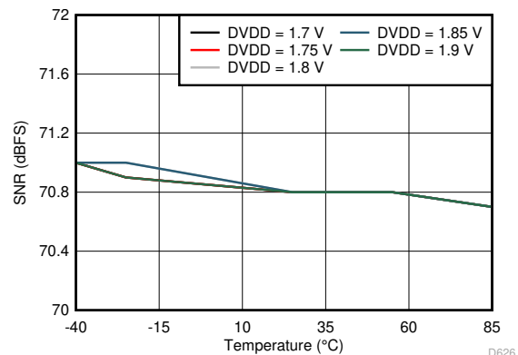
6-56. Signal-to-Noise Ratio vs DVDD Supply and Temperature (30 MHz)
