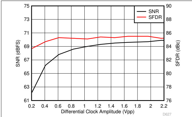
6-57. Performance vs Differential Clock Amplitude (40 MHz)
