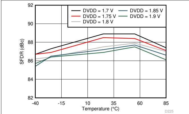
6-115. Spurious-Free Dynamic Range vs DVDD Supply and Temperature (170 MHz)
