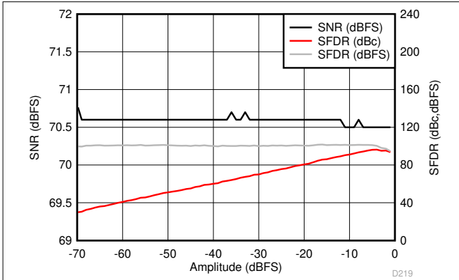
6-109. Performance vs Input Amplitude (30 MHz)
