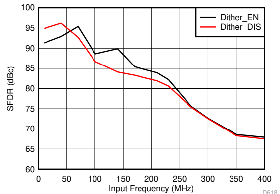
6-48. Spurious-Free Dynamic Range vs Input Frequency
