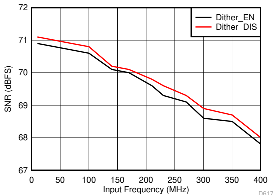
6-47. Signal-to-Noise Ratio vs Input Frequency
