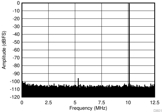
6-1. FFT for 10-MHz Input Signal (Dither On)
