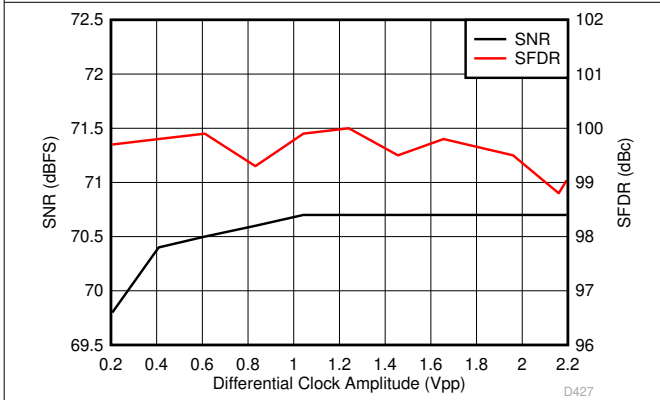
6-87. Performance vs Differential Clock Amplitude (40 MHz)
