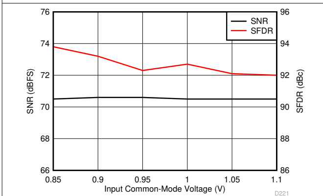
6-111. Performance vs Input Common-Mode Voltage (30 MHz)
