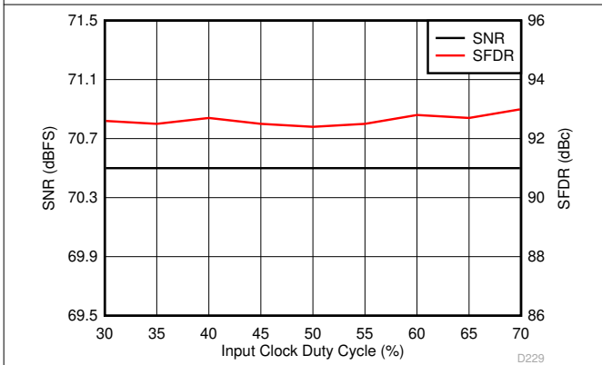
6-119. Performance vs Clock Duty Cycle (30 MHz)
