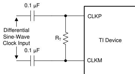
8-1. Differential Sine-Wave Clock Driving Circuit
