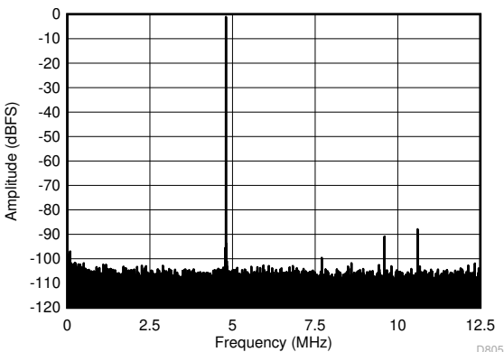
6-3. FFT for 70-MHz Input Signal (Dither On)
