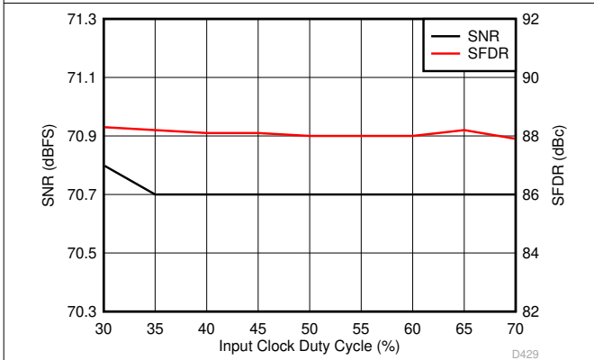
6-89. Performance vs Clock Duty Cycle (30 MHz)
