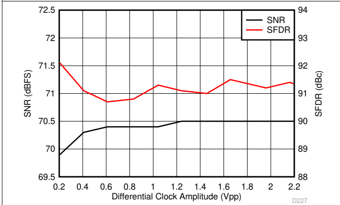
6-117. Performance vs Differential Clock Amplitude (40 MHz)
