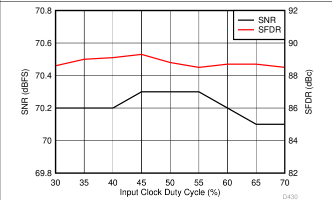
6-90. Performance vs Clock Duty Cycle (150 MHz)
