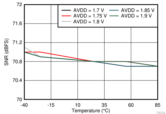
6-54. Signal-to-Noise Ratio vs AVDD Supply and Temperature (30 MHz)
