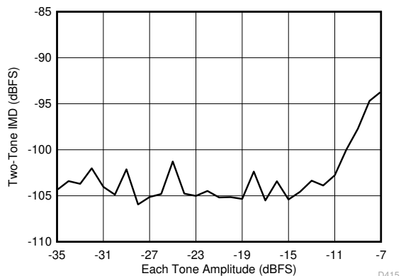
6-75. Intermodulation Distortion vs Input Amplitude (46 MHz and 50 MHz)
