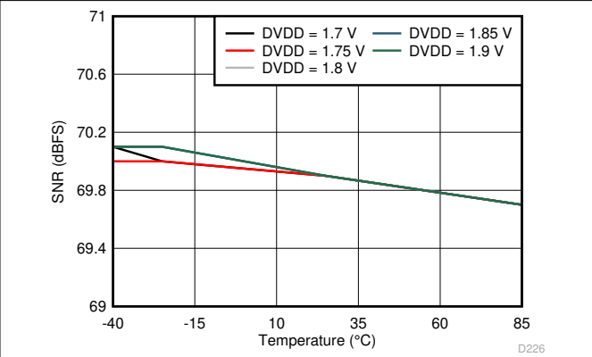
6-116. Signal-to-Noise Ratio vs DVDD Supply and Temperature (170 MHz)
