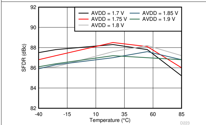
6-113. Spurious-Free Dynamic Range vs AVDD Supply and Temperature (170 MHz)
