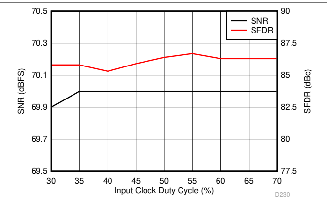
6-120. Performance vs Clock Duty Cycle (150 MHz)
