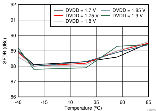
6-55. Spurious-Free Dynamic Range vs DVDD Supply and Temperature (30 MHz)
