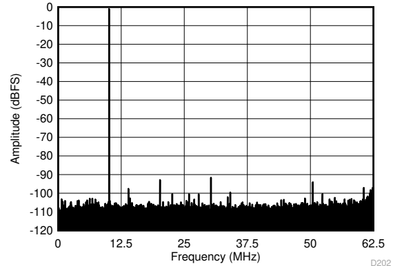
6-92. FFT for 10-MHz Input Signal (Chopper On, Dither Off)
