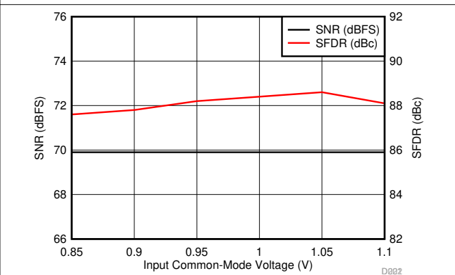
6-112. Performance vs Input Common-Mode Voltage (170 MHz)
