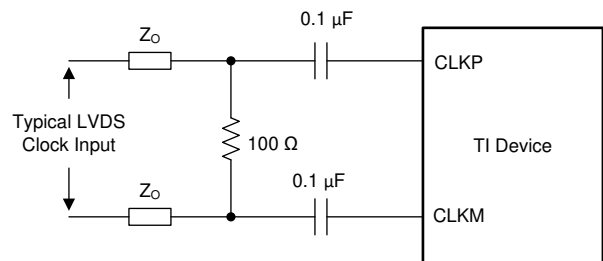
8-2. LVDS Clock Driving Circuit
