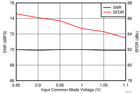
6-52. Performance vs Input Common-Mode Voltage (170 MHz)
