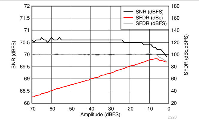
6-110. Performance vs Input Amplitude (170 MHz)
