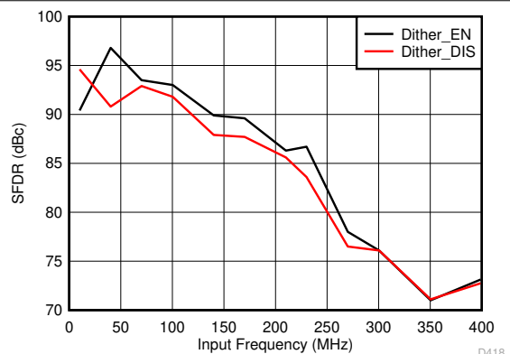
6-78. Spurious-Free Dynamic Range vs Input Frequency
