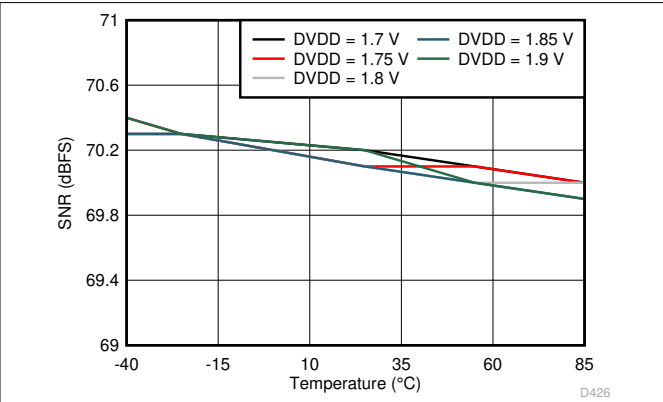
6-86. Signal-to-Noise Ratio vs DVDD Supply and Temperature (170 MHz)
