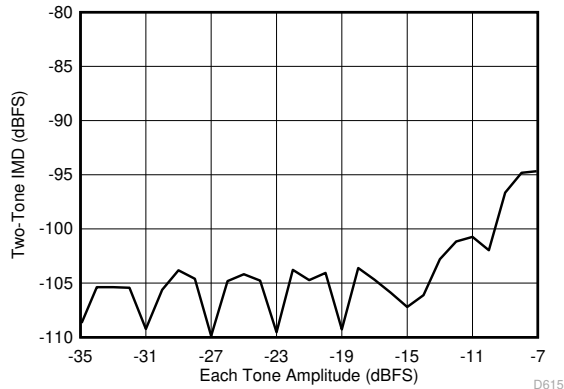
6-45. Intermodulation Distortion vs Input Amplitude (46 MHz and 50 MHz)
