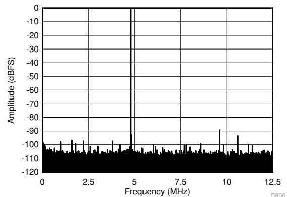
6-4. FFT for 70-MHz Input Signal (Dither Off)
