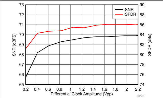
6-118. Performance vs Differential Clock Amplitude (150 MHz)
