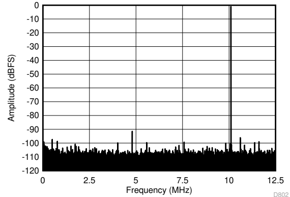
6-2. FFT for 10-MHz Input Signal (Dither Off)
