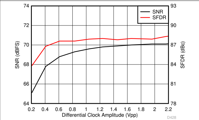
6-88. Performance vs Differential Clock Amplitude (150 MHz)
