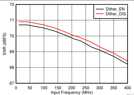
6-77. Signal-to-Noise Ratio vs Input Frequency
