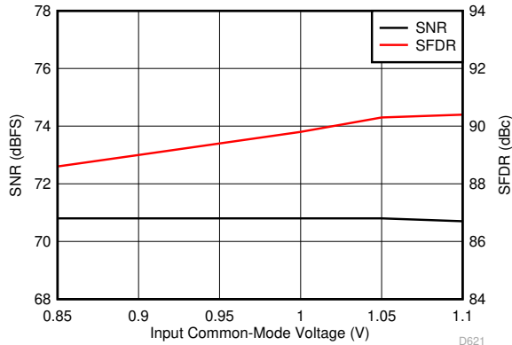
6-51. Performance vs Input Common-Mode Voltage (30 MHz)
