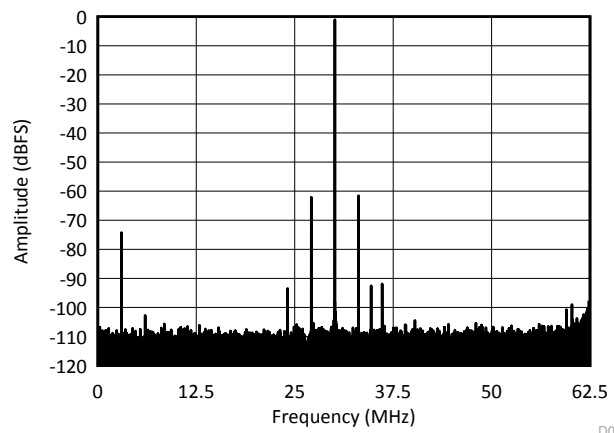
f_{IN} = 30.1\text{ MHz} , f_{PSRR} = 3\text{ MHz} , A_{PSRR} = 50\text{ mV}_{PP} , \text{SINAD} = 58.51\text{ dBFS} , \text{SFDR} = 60.53\text{ dBc}
