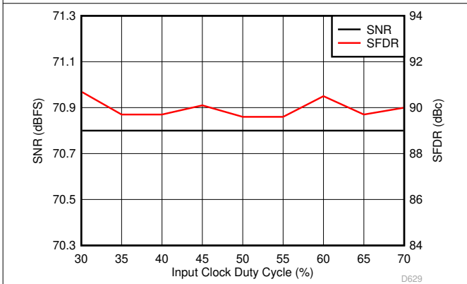
6-59. Performance vs Clock Duty Cycle (30 MHz)
