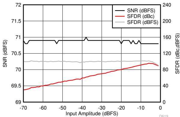
6-49. Performance vs Input Amplitude (30 MHz)
