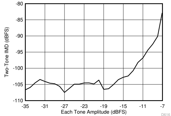
6-46. Intermodulation Distortion vs Input Amplitude (185 MHz and 190 MHz)
