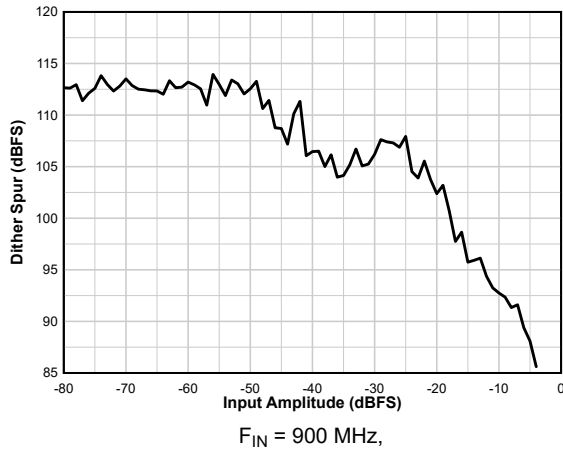
6-84. Dither Spur vs A_{IN}
