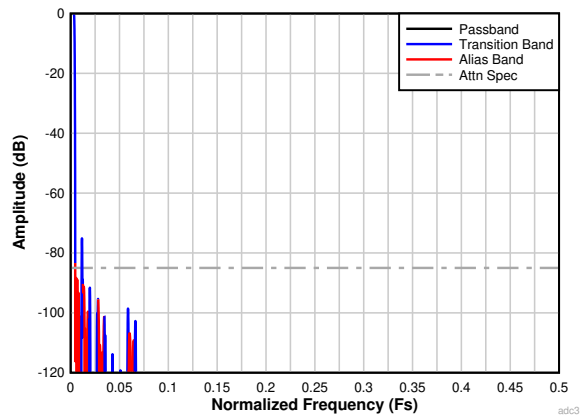
7-35. Complex Decimation by 128 Filter Response
