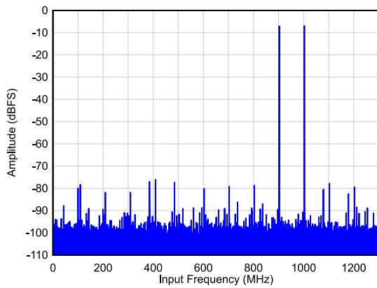
Figure 6-23. Two Tone FFT at F_{IN} = 900/1000 MHz
