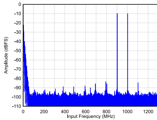
Figure 6-24. Two Tone FFT at F_{IN} = 900/1000 MHz
