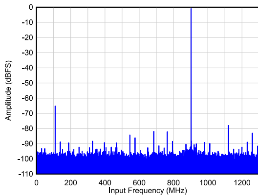
6-5. Single Tone FFT at F_{IN} = 900\text{ MHz}
