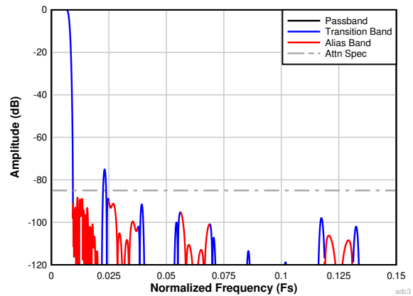
7-33. Complex Decimation by 64 Filter Response
