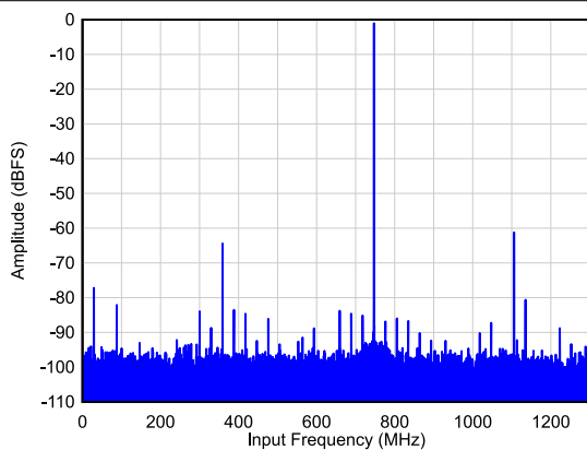
6-7. Single Tone FFT at F_{IN} = 1400\text{ MHz}
