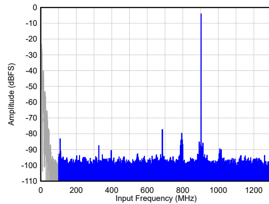
6-6. Single Tone FFT at F_{IN} = 900\text{ MHz}
