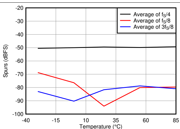
☒ 9-8. Offset Corrector Block Disabled
