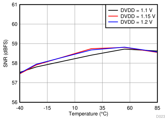
6-47. Signal-to-Noise Ratio vs. DVDD Supply and Temperature
