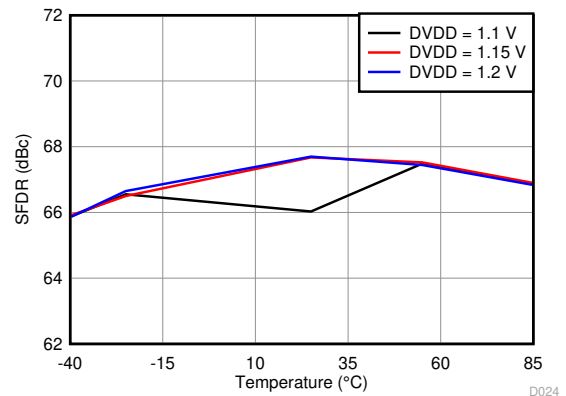
6-48. Spurious-Free Dynamic Range vs. DVDD Supply and Temperature
