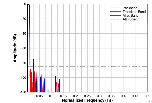
7-29. Complex Decimation by 64 Filter Response
