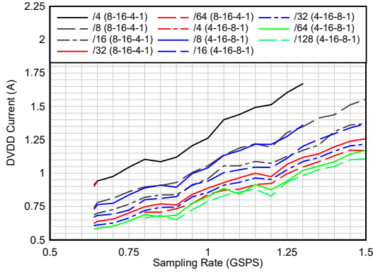
6-49. Current vs Sampling Rate vs Complex Decimation
