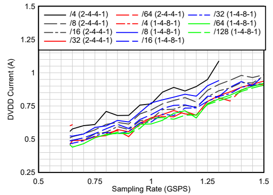
6-44. Current vs Sampling Rate vs Averaging
