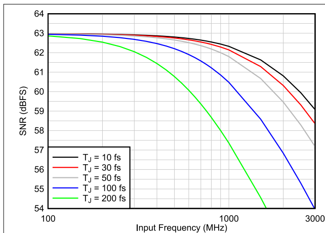
8-2. SNR vs T_{\text{jitter}} vs F_{\text{IN}} (1x AVG)
