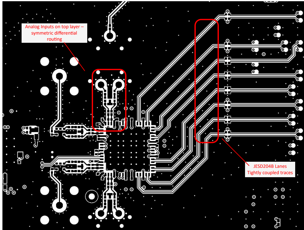
8-11. Layout example: top layer of the EVM
