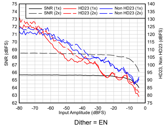
6-30. AC Performance vs A_{IN}
