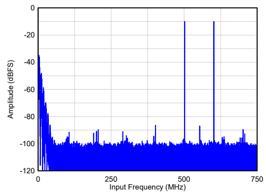
IMD3 = 75 dBc A_{IN} = -10 dBFS/tone, 1x AVG, Dither = EN
