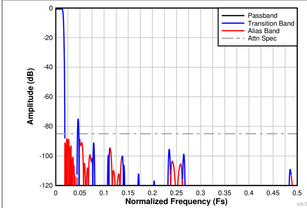
7-27. Complex Decimation by 32 Filter Response
