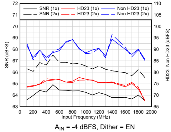
6-26. AC Performance vs F_{IN}
