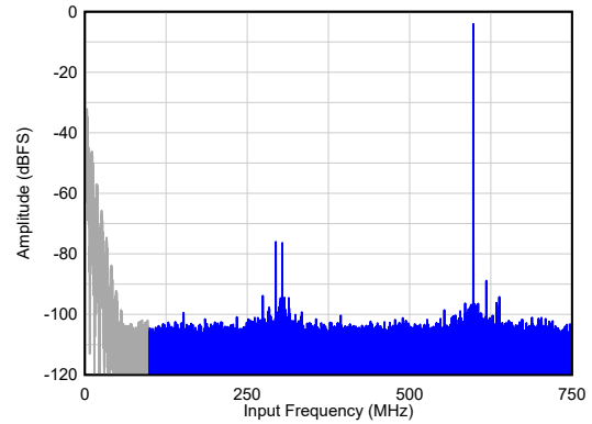
A_{IN} = -4 dBFS, 2x AVG, Dither = EN SNR = 67.0 dBFS 2 , HD23 = 72 dBc, Non HD23 = 89 dBFS
