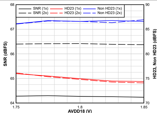
6-36. AC Performance vs AVDD18
