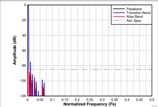
7-32. Complex Decimation by 128 Filter Response
