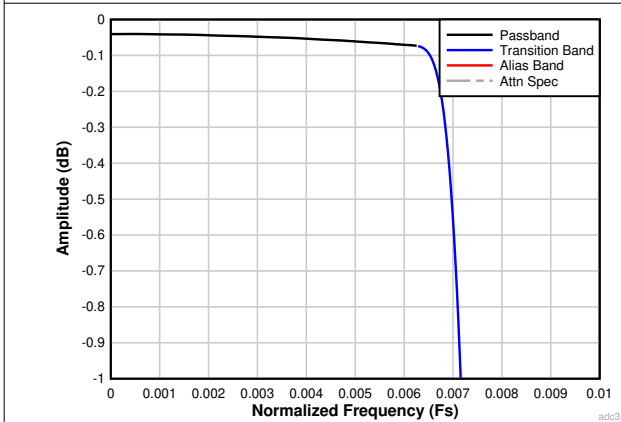
7-31. Decimation by 64 Passband Ripple Response
