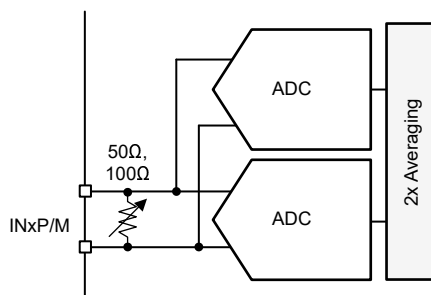
图 7-42. Internal Digital Averaging
