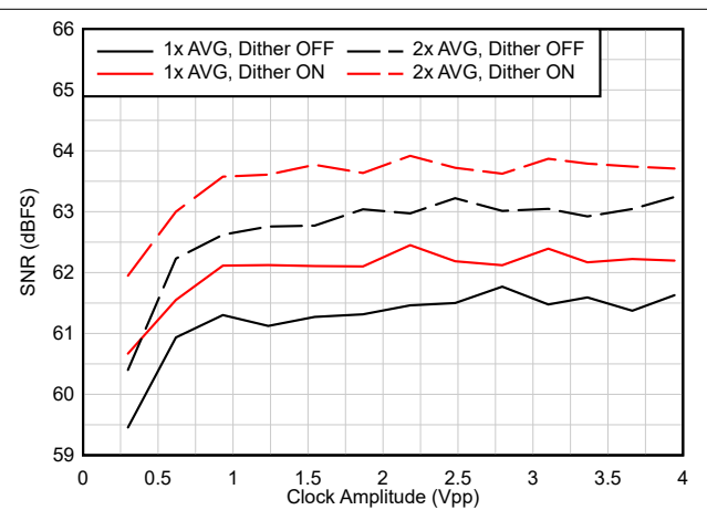
8-3. SNR vs Clock Amplitude
