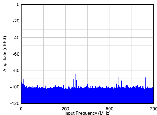
A_{IN} = -20 dBFS, 1x AVG, Dither = DIS SNR = 65.2 dBFS, HD23 = 64 dBc, Non HD23 = 88 dBFS
