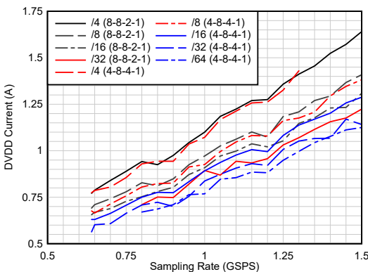
6-45. Current vs Sampling Rate vs Real Decimation
