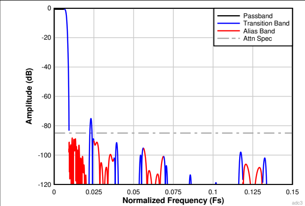
7-30. Complex Decimation by 64 Filter Response
