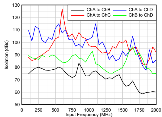
6-34. Isolation vs Input Frequency
