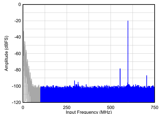
A_{IN} = -20 dBFS, 1x AVG, Dither = EN SNR = 64.8 dBFS 1 , HD23 = 59 dBc, Non HD23 = 79 dBFS
