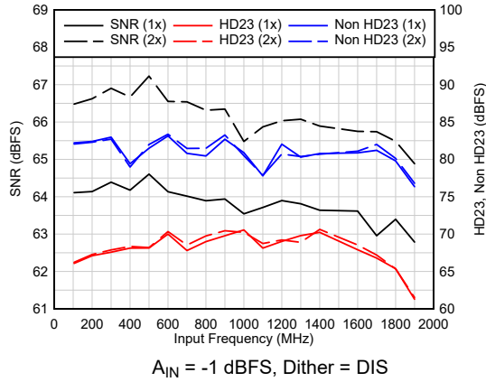
6-25. AC Performance vs F_{IN}
