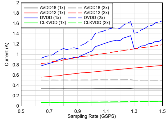
6-44. Current vs Sampling Rate vs Averaging
