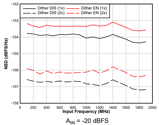
6-28. NSD Performance vs F_{IN}
