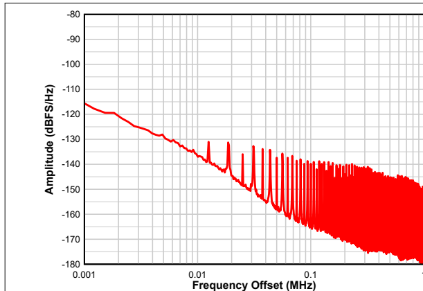
Figure 7-6. Dither Close-Up
