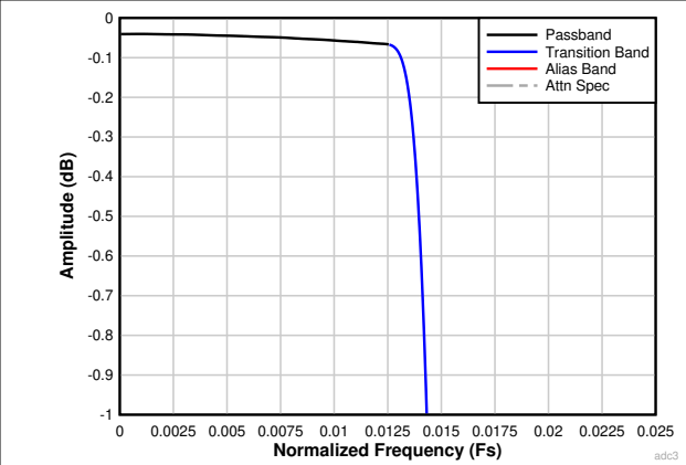
7-28. Decimation by 32 Passband Ripple Response
