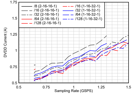
6-50. Current vs Sampling Rate vs Complex Decimation
