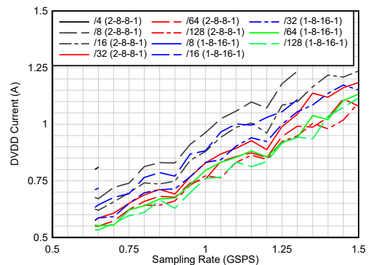
6-46. Current vs Sampling Rate vs Real Decimation
