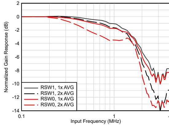
7-2. Full power input bandwidth (100 Ω)
