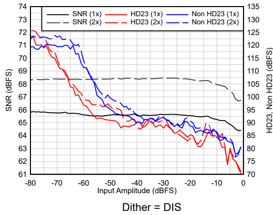
6-29. AC Performance vs A_{IN}
