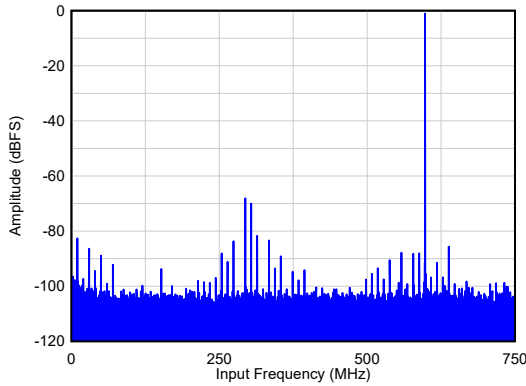
A_{IN} = -1 dBFS, 2x AVG, Dither = DIS SNR = 66.8 dBFS, HD23 = 67 dBc, Non HD23 = 82 dBFS
