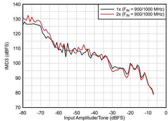
6-32. IMD3 Performance vs A_{IN}
