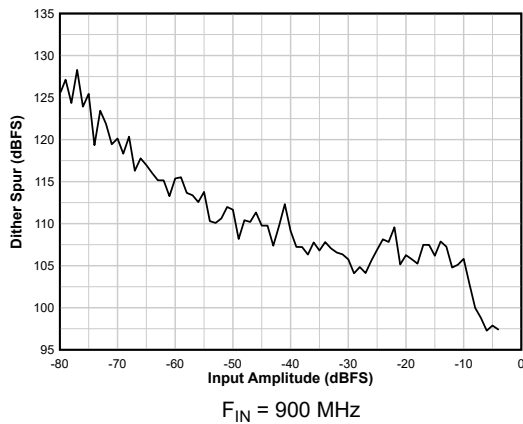
6-27. Dither Spur vs A_{IN}
