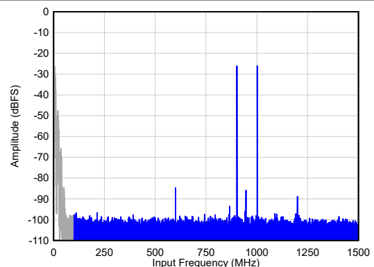
IMD3 = 71 dBc A_{IN} = -26\text{ dBFS/tone} , 1x AVG, Dither = EN
