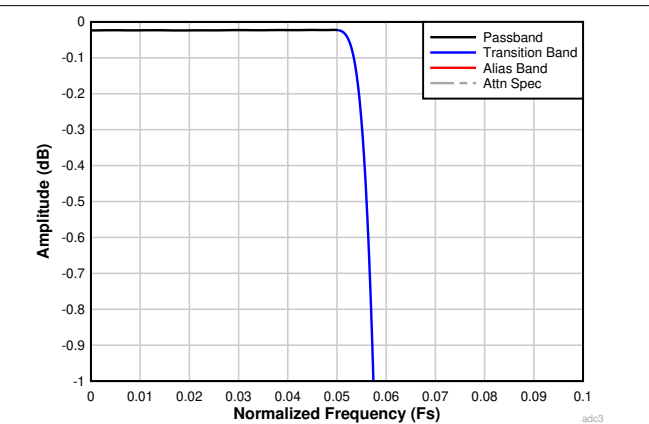
6-27. Decimation by 8 Passband Ripple Response
