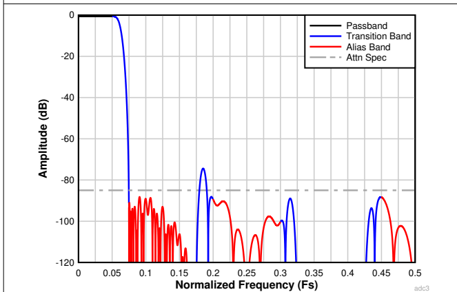
6-26. Complex Decimation by 8 Filter Response
