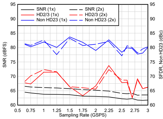
F_{IN} = 900\text{ MHz} , A_{IN} = -1\text{ dBFS} , Dither = DIS
