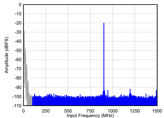
5-14. Single Tone FFT at F_{IN} = 900 MHz
