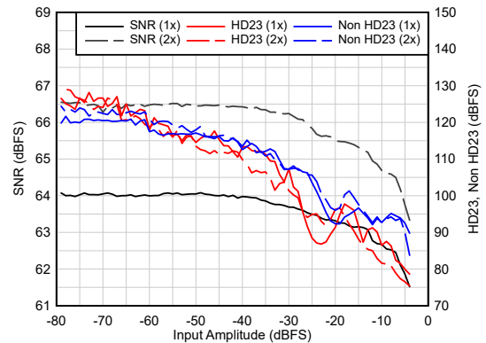
F_{IN} = 900\text{ MHz} , Dither = EN 5-28. AC Performance vs A_{IN}
