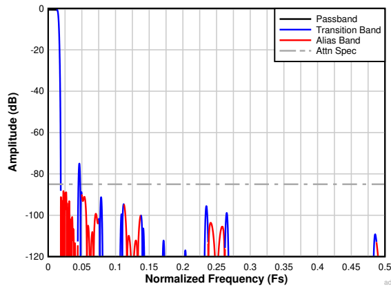
6-30. Complex Decimation by 32 Filter Response
