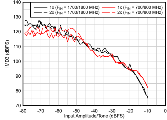
5-30. IMD3 Performance vs A_{IN}
