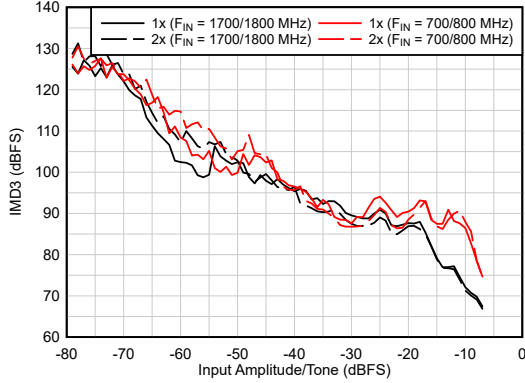
5-29. IMD3 Performance vs A_{IN}
