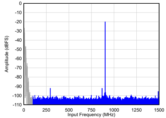
SNR = 65.5 dBFS 1 , SFDR = 73 dBc, Non HD23 = 95 dBFS A_{IN} = -20\text{ dBFS} , 2x AVG, Dither = EN
