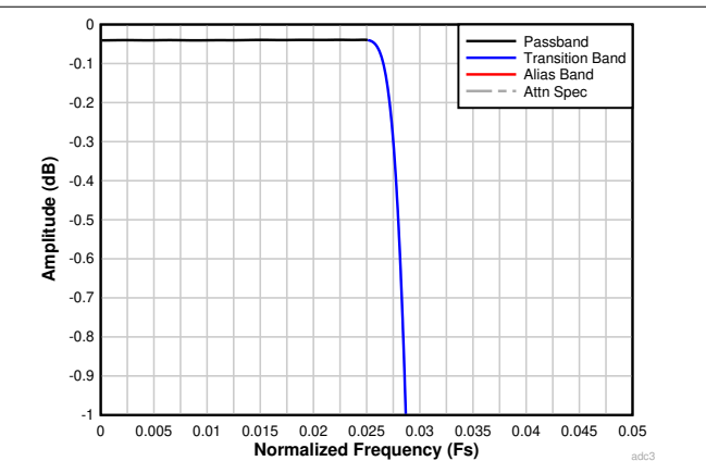
6-29. Decimation by 16 Passband Ripple Response
