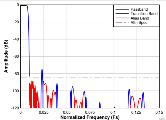
6-33. Complex Decimation by 64 Filter Response
