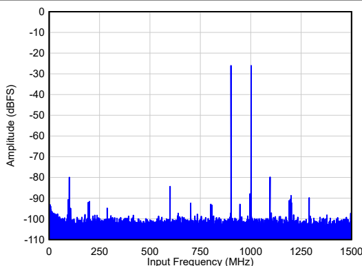
IMD3 = 54 dBc A_{IN} = -26\text{ dBFS/tone} , 1x AVG, Dither = DIS
