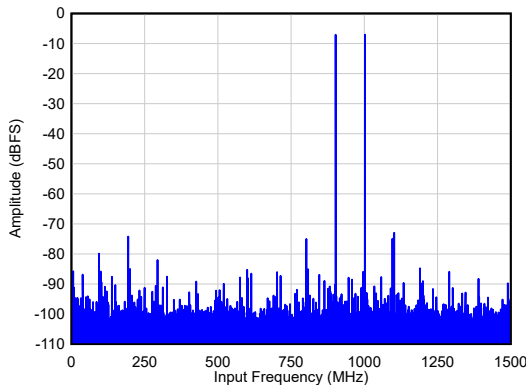
IMD3 = 68 dBc A_{IN} = -7\text{ dBFS/tone} , 1x AVG, Dither = DIS
