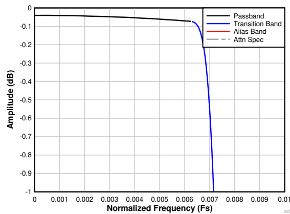
6-34. Decimation by 64 Passband Ripple Response
