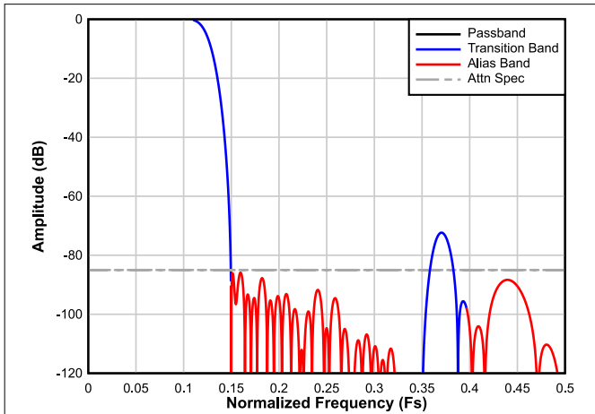
6-24. Complex Decimation by 4 Filter Response
