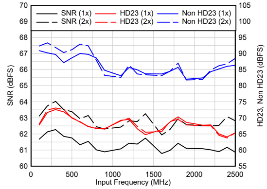
A_{IN} = -4\text{ dBFS} , Dither = EN 5-24. AC Performance vs F_{IN}
