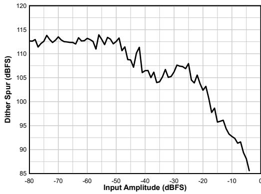
F_{IN} = 900\text{ MHz} , 5-25. Dither Spur vs A_{IN}
