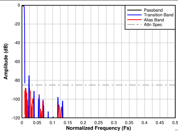
6-32. Complex Decimation by 64 Filter Response
