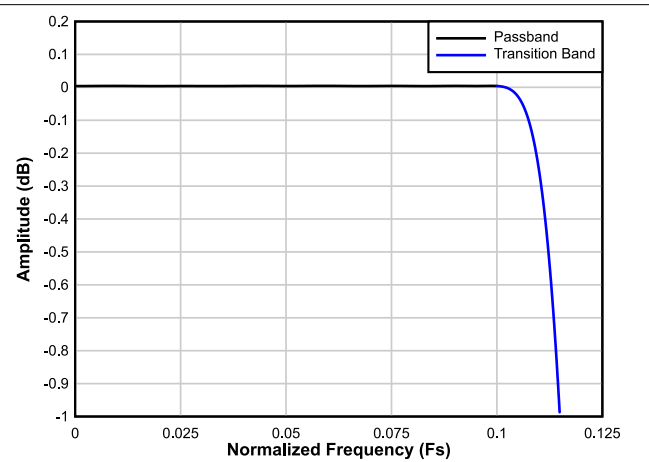
6-25. Decimation by 4 Passband Ripple Response
