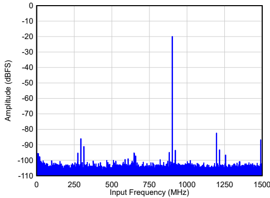
SNR = 66.4 dBFS, SFDR = 63 dBc, Non HD23 = 86 dBFS A_{IN} = -20\text{ dBFS} , 2x AVG, Dither = DIS
