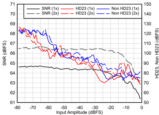
F_{IN} = 900\text{ MHz} , Dither = DIS 5-27. AC Performance vs A_{IN}
