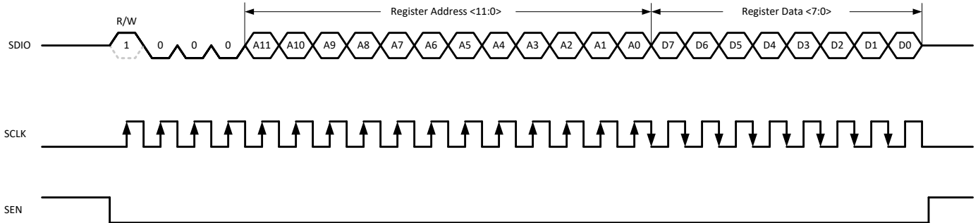
図 6-47. Serial Register Read Timing Diagram
