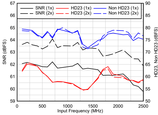
A_{IN} = -1\text{ dBFS} , Dither = DIS 5-23. AC Performance vs F_{IN}
