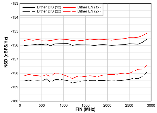
A_{IN} = -20\text{ dBFS} 5-26. NSD Performance vs F_{IN}
