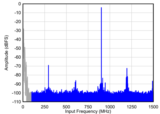
5-6. Single Tone FFT at F_{IN} = 900\text{ MHz}
