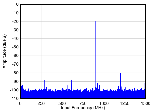
5-13. Single Tone FFT at F_{IN} = 900 MHz
