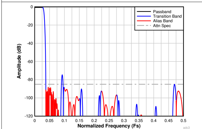
6-28. Complex Decimation by 16 Filter Response
