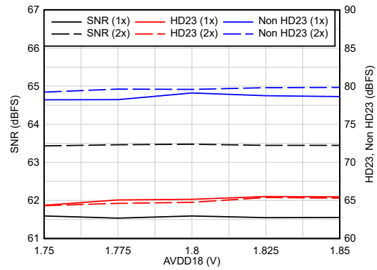
F_{IN} = 900\text{ MHz} , A_{IN} = -1\text{ dBFS} , Dither = DIS, Other supplies nominal
