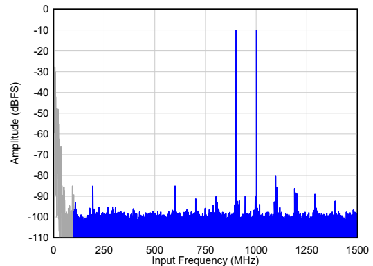
IMD3 = 70 dBc A_{IN} = -10\text{ dBFS/tone} , 1x AVG, Dither = EN
