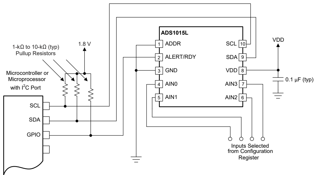
☒ 9-1. Typical Connections of the ADS1015L
